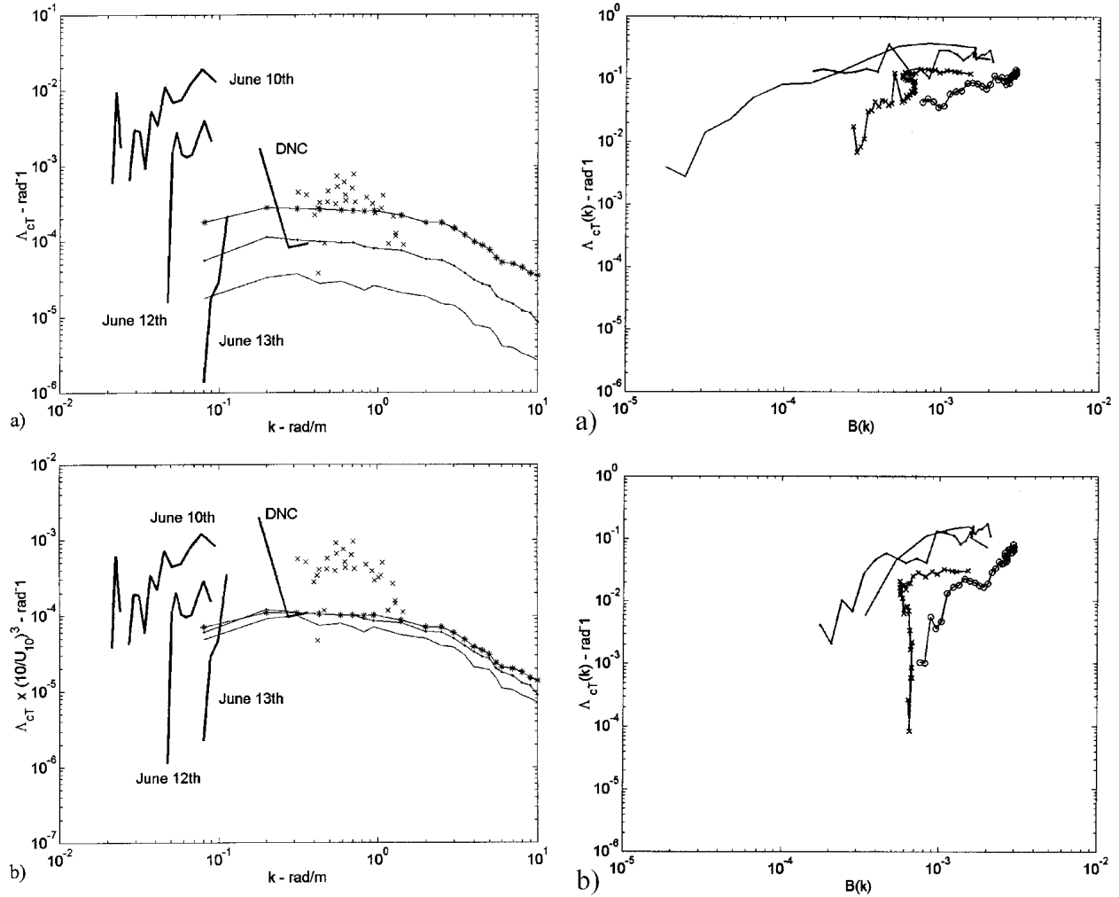
FIG. 7. (a) Estimates of \Lambda_{cT}(k) at wave slope threshold T = 0.12 for SOWEX and DNC experiment (thick lines). Phillips et al.'s (2001) estimates of \Lambda(k) are designated by crosses. Melville and Matusov's (2002) estimates of \Lambda(k) are shown at U_{10} = 7.2 (—), 9.8 (—), and 13.6 \text{ m s}^{-1} (*—). (b) As in (a) except \Lambda_{cT}(k) and \Lambda(k) are multiplied by (10/U_{10})^3 .
