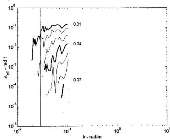
FIG. 4. As in Fig. 3 but for corrected steep wave statistic \Lambda_{cT} vs k . Vertical line indicates dominant wavenumber.
