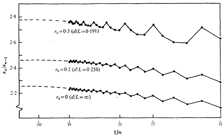
FIGURE 4. Domb-Sykes plot of the expansion for S = c/q_{\text{crest}} = \sum_{n=0}^{\infty} s_n h^n for three depths.
