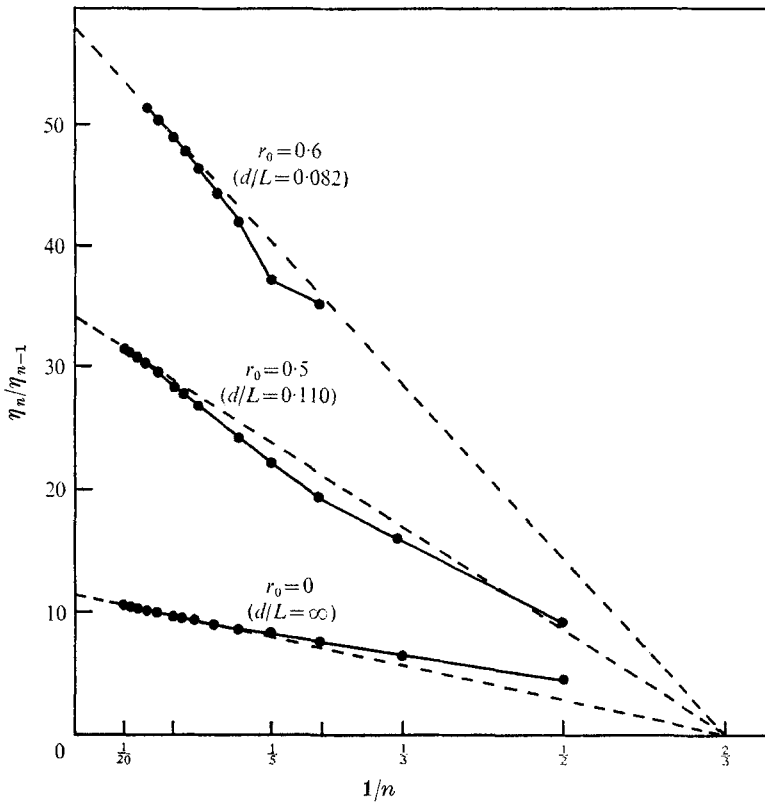
FIGURE 2. Domb-Sykes plot for wave height h = \sum_{n=1}^{\infty} \eta_n a_1^{2n-1} .
