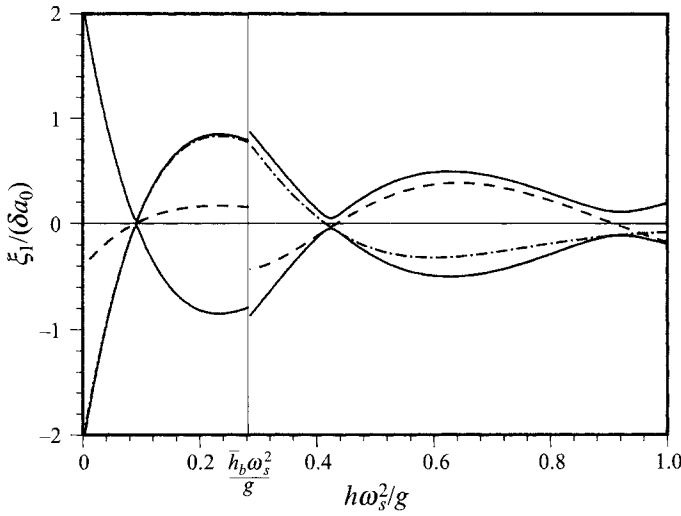
FIGURE 2. Dimensionless infragravity wave: —, envelope \pm|\hat{\xi}_1| , and elevations ----, \text{Re}\{\hat{\xi}_1\} at t=0 , and - · - · -, \text{Im}\{\hat{\xi}_1\} at t=T/4 , versus \hat{h} for the input parameters h_x \omega_s/\omega = 0.25 , \hat{h}_0 = 1 , \hat{a}_0 = 0.1 , \kappa = 1 , \gamma_0 = 0.4 , and \alpha_0 = 15^\circ , which yield R = 1.8 .
