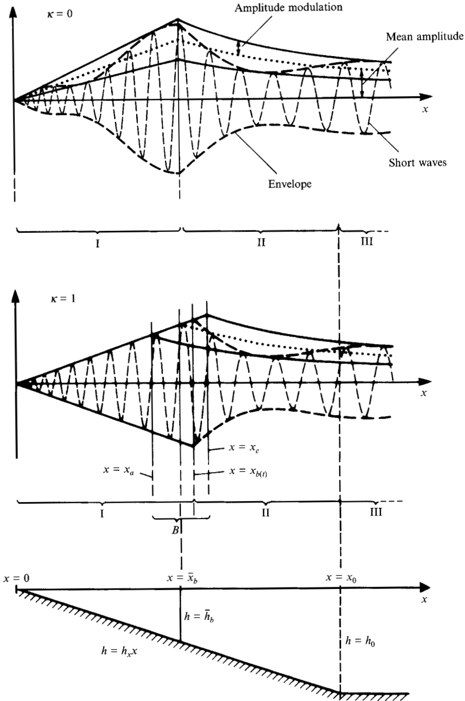
FIGURE 1. Sketch of bottom topography and two examples of short-wave modelling with associated definitions of the regions I, II, B, and III. From Schäfer (1993).
