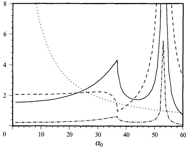
FIGURE 10. Some key results for the infragravity-wave solution versus the angle of incidence, 1^\circ \leq \alpha_0 \leq 60^\circ : —, 'reflection coefficient' R ; ---, shoreline infragravity-wave amplitude, |\xi_1(0)|/(\delta a_0) ; - · - · -, amplitude of the seaward progressing free long wave measured at the edge of the slope, |\xi_f|/(\delta a_0) . The other input parameters were h_x \omega_s/\omega = 0.25 , \hat{h}_0 = 1 , \hat{a}_0 = 0.1 , \kappa = 1 , and \gamma_0 = 0.4 . Also the derived parameter -a (·····) is shown. Note the special behaviour at the critical angle of incidence \alpha_{cr} = 36.86^\circ and the edge-wave resonance at \alpha_0 = 51.11^\circ .
