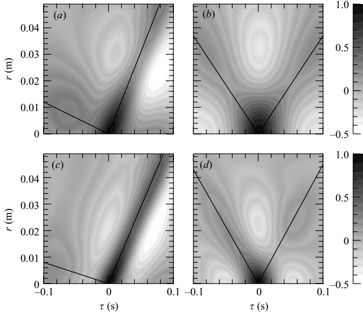
FIGURE 14. Space-time longitudinal correlation functions: (a), (c) C_{xx}(re_x, \tau) and (b), (d) C_{yy}(re_y, \tau) . (a), (b) Turbulence generated by the active grid (25OPT in table 1). (c), (d) Turbulence generated by the static grid (25STAT in table 1). Full lines indicate the convection velocity of structures: (a) v_f^{st} = 0.37 \text{ m s}^{-1} ; (b) v_f^{sp} = 0.37 \text{ m s}^{-1} ; (c) v_f^{st} = 0.33 \text{ m s}^{-1} ; (d) v_f^{sp} = 0.44 \text{ m s}^{-1} .
