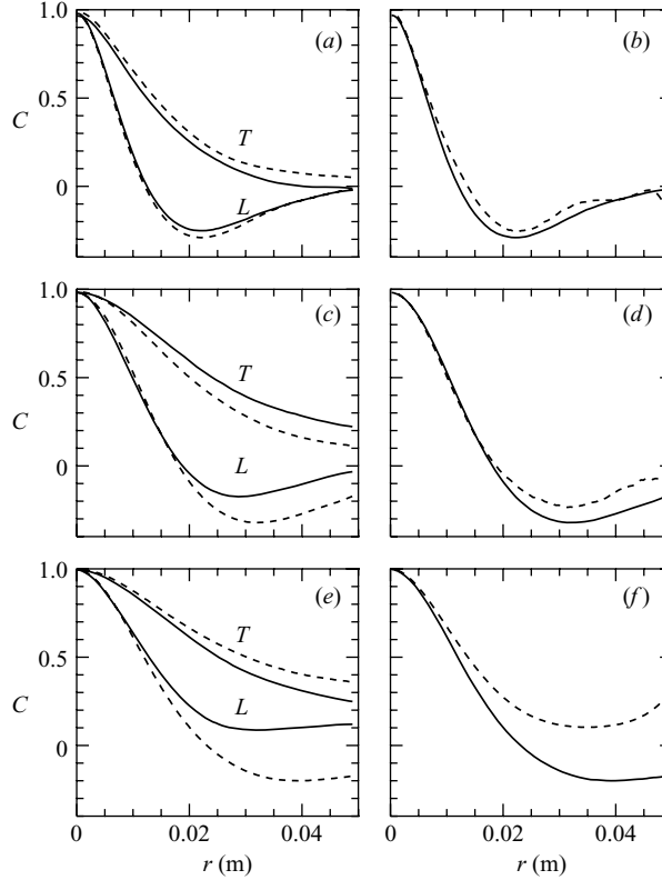
FIGURE 12. Longitudinal C_{\beta\beta}(\mathbf{r}\mathbf{e}_\beta) ( L ) and transverse C_{\alpha\alpha}(\mathbf{r}\mathbf{e}_\beta) ( T ) correlation functions of the surface gradient field. (a) Near-isotropic turbulence stirred by the passive grid (25STAT in table 1); full lines: \beta = x ; dashed lines \beta = y . (b) Full line: longitudinal C_{yy}(\mathbf{r}\mathbf{e}_y) from (a); dashed line: longitudinal C^L computed from transverse C_{xx}(\mathbf{r}\mathbf{e}_y) from (a), using the isotropy relation (4.2). (c) Near-isotropic turbulence stirred by the active grid (25OPT in table 1); full lines: \beta = x ; dashed lines \beta = y . (d) Full line: C_{yy}(\mathbf{r}\mathbf{e}_y) from (c); dashed line: C^L computed from C_{xx}(\mathbf{r}\mathbf{e}_y) from (c), using the isotropy relation (4.2). (e) Anisotropic turbulence (25RAN in table 1); full lines: \beta = x ; dashed lines \beta = y . (f) Full line: C_{yy}(\mathbf{r}\mathbf{e}_y) from (e); dashed line: C^L computed from C_{xx}(\mathbf{r}\mathbf{e}_y) from (e), using the isotropy relation (4.2).
