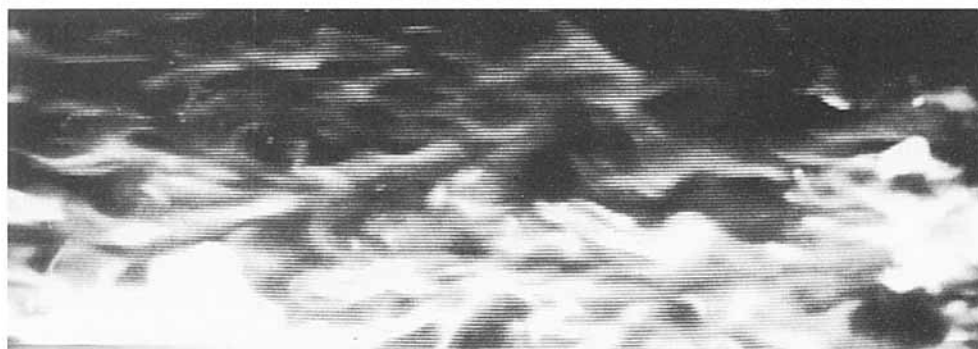
FIGURE 15. The evolution of low-speed streaks when the viscosity of the fluid in the wall layer is increased by about 30% (the first frame is at about -113 time units from the moment of maximum deceleration. Subsequent frames are 12.5 time units apart). The structural differences in streak formation relative to the pure water case (see figures 7i–7xxv) are rather striking.
