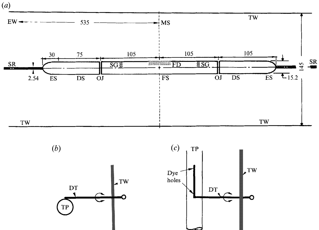
FIGURE 1. (a) Schematic side view of experimental set-up (dimensions are given in centimetres). DS, dummy section; ES, end section of test cylinder; EW, endwall of tunnel; FD, fluorescent dye; FS, force sleeve; MS, mid-section; OJ, overlapping joint; SG, strain gauges; SR, supporting rod; TW, tunnel wall. (b) Schematic cross-sectional view of dye introduction system. DT, dye tube; TP, test pipe; TW, tunnel wall. (c) Schematic plan view of dye tube and location of dye holes.
