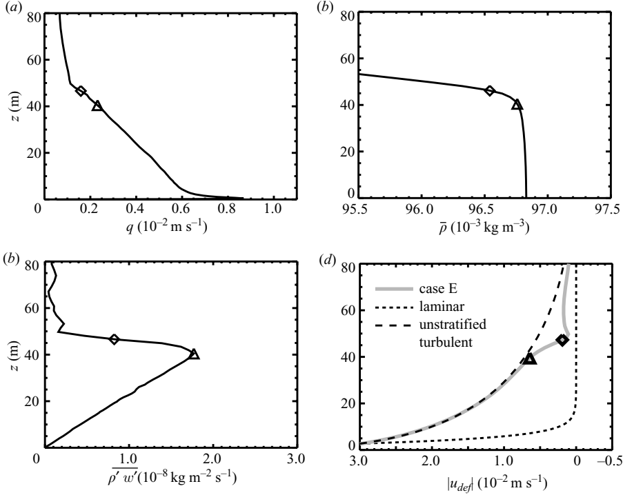
FIGURE 6. The vertical profiles of (a) the velocity scale of turbulence q , (b) the horizontal averaged density \bar{\rho}^{x,y} , (c) the turbulent density flux \rho'w'^{x,y} and (d) the velocity defect of the mean tidal current |u_{def}| (the grey line) in case E. The profiles are averaged over the last tidal cycle of the experiment ( t = 47\text{--}48 ). \triangle , z_m ; \diamond , z_t . The short-dashed and long-dashed lines in (d) indicate the velocity defects of the laminar and unstratified turbulent tidal flows, respectively.
