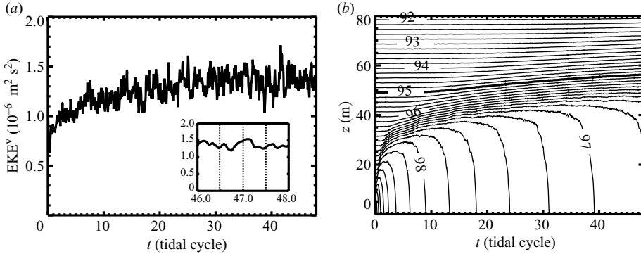
FIGURE 4. Time evolution of (a) the areal average of the eddy kinetic energy \overline{\text{EKE}}^V and (b) the horizontal averaged density \overline{\rho}^{x,y} in case E. The inset in (a) shows \overline{\text{EKE}}^V for t=46-48 . The contour interval of (b) is 2.0 \times 10^{-4} \text{ kg m}^{-3} .
