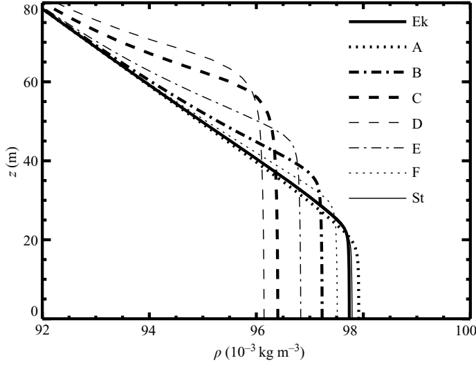
FIGURE 5. The vertical profiles of the horizontal averaged density \bar{\rho}^{x,y} for all cases. The profiles are averaged over the last tidal cycle of the experiments ( t = 47\text{--}48 ).
