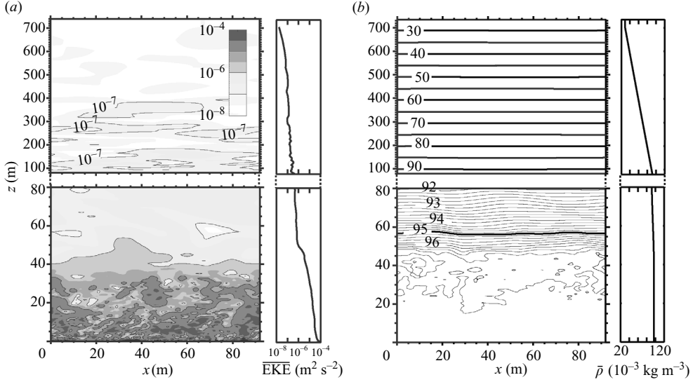
FIGURE 3. (a) Vertical section of the eddy kinetic energy EKE at y=0 and t=48 in case E ( Ro_t = 1.2 ), together with the vertical profile of the horizontal average \overline{\text{EKE}}^{x,y} . Contour lines indicate 10^{-7} , 10^{-6} and 10^{-5} \text{ m}^2 \text{ s}^{-2} , and darker shades represent larger values. Note that the vertical scale is different for the lower panel showing the range from the bottom ( z=0 \text{ m} ) to z=80 \text{ m} and the upper panel showing from z=80 to 740 \text{ m} . (b) Same as (a), but for density \rho . The contour interval of the thin (thick) line is 2.0 \times 10^{-4} \text{ kg m}^{-3} ( 5.0 \times 10^{-3} \text{ kg m}^{-3} ). The thin contour lines are omitted in the upper panel.
