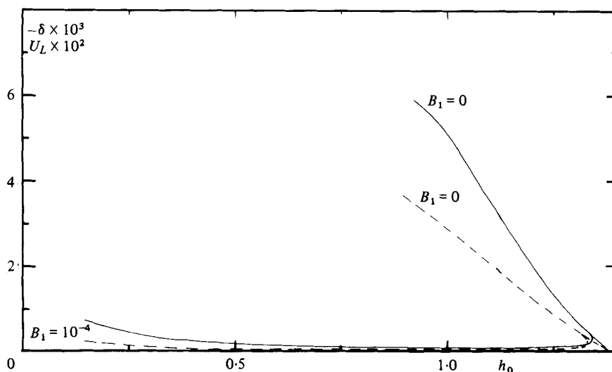
FIGURE 8. Variation of set-down \delta and mean longshore Stokes-drift velocity U_L for waves near a caustic, with m_2 = 1.1 , B_1 = 0 and 10^{-4} . — \delta , U_L --- \delta , U_L - - - \delta , U_L .
