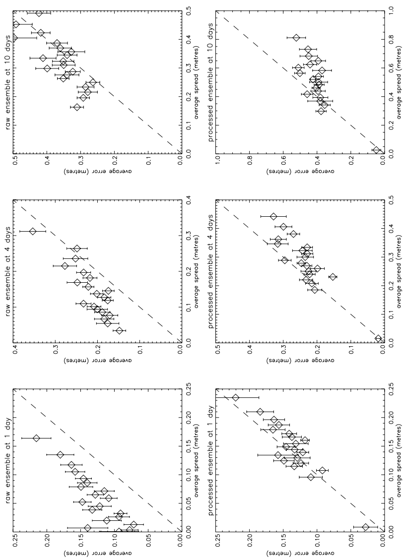
Fig. 10. As Fig. 7 but for the Santos Basin.
