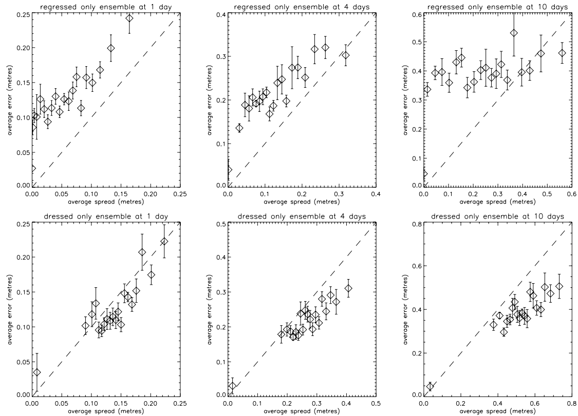
Fig. 15. A comparison of the spread-skill relationship of ensemble forecasts which have only been regressed but not dressed (top panels) with those which have been dressed but not regressed (bottom panels). The forecasts are for significant wave height in the Santos Basin. Notice that if the forecasts are regressed but not dressed the errors are greatly underestimated, even more than for the raw ensemble at 10 days (compare with Fig. 10). If the forecasts are only dressed, without first regressing them, the results are very similar to the full processing step.
