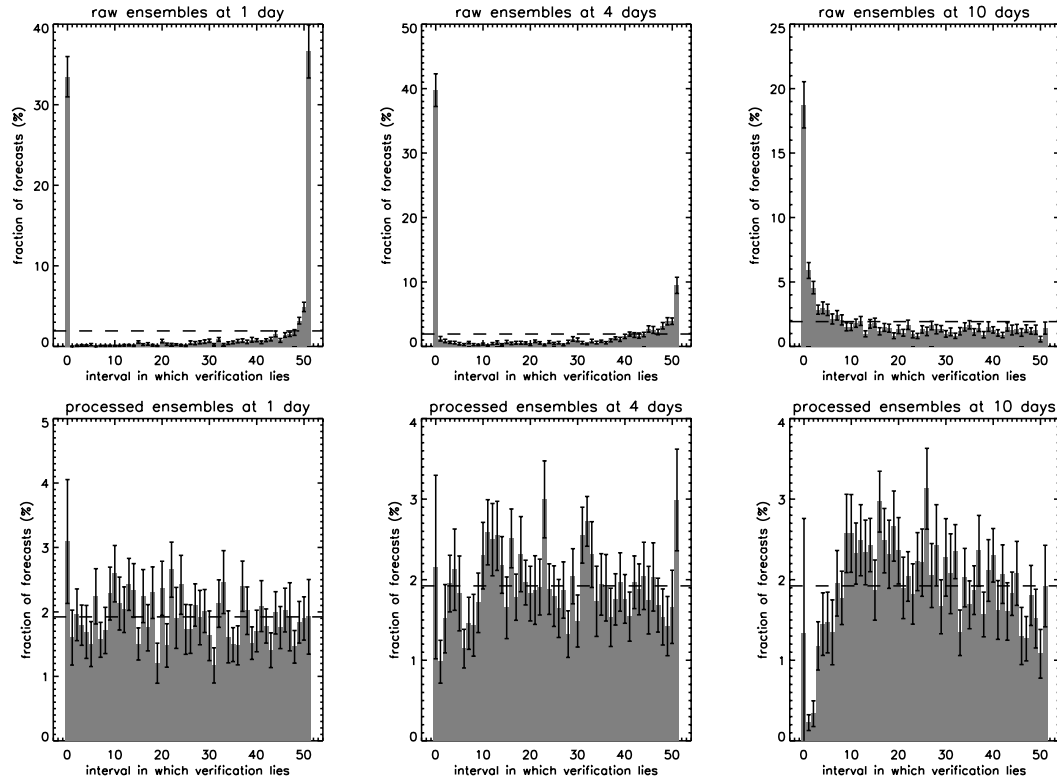
Fig. 11. A comparison of rank histograms of the 51-member unprocessed ECMWF ensemble and a 51-member ensemble constructed by regressing and dressing the ECMWF ensemble. The top panels show the rank histograms of the unprocessed ensembles at lead times of 1, 4 and 10 days. The bottom panels show the histograms of the processed ensemble for the same lead times. The histograms were constructed using forecasts for the period March 1999 to December 2001. The error bars are the standard error estimates obtained by bootstrap resampling the forecasts in blocks of 20 days. The dashed lines represent the fraction of forecasts that would lie in each interval in a flat rank histogram ( 1/52 \approx 1.9\% ). It can be seen that the raw ensembles have rank histograms which are overpopulated at the extremes whereas the processed ensembles have histograms which are nearly flat—a necessary condition of reliable forecasts. Note that the verification lies outside the raw ensembles far more often than would be expected for reliable forecasts—70% of the time at 1 day compared to the expected 2/52 \approx 3.8\% of the time.
