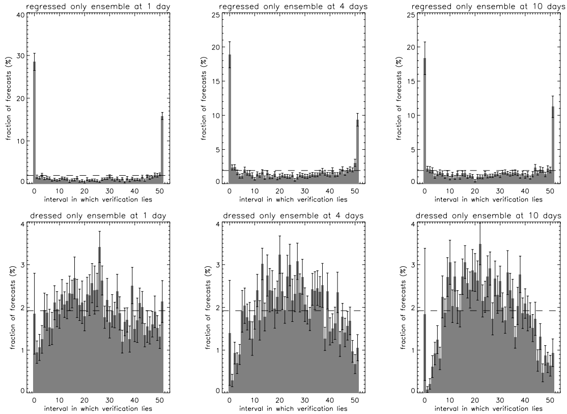
Fig. 16. A comparison of the reliabilities of ensemble forecasts which have only been regressed but not dressed (top panels) with those which have been dressed but not regressed (bottom panels). The forecasts are for significant wave height in the Santos Basin.
