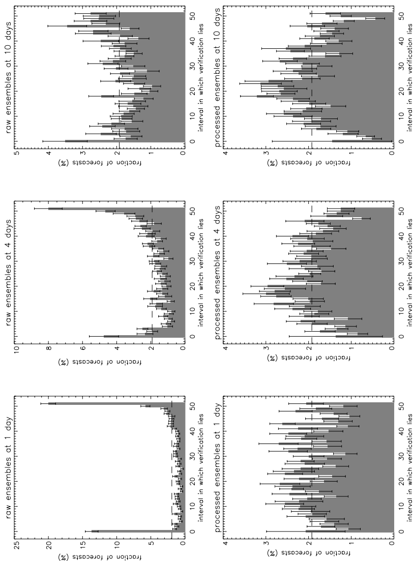
Fig. 14. As Fig. 11 but for the Santos Basin.
