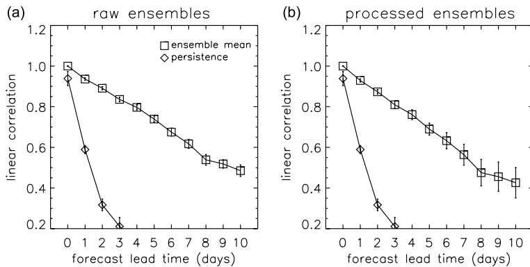
Fig. 6. As Fig. 3 but for the Santos Basin.
