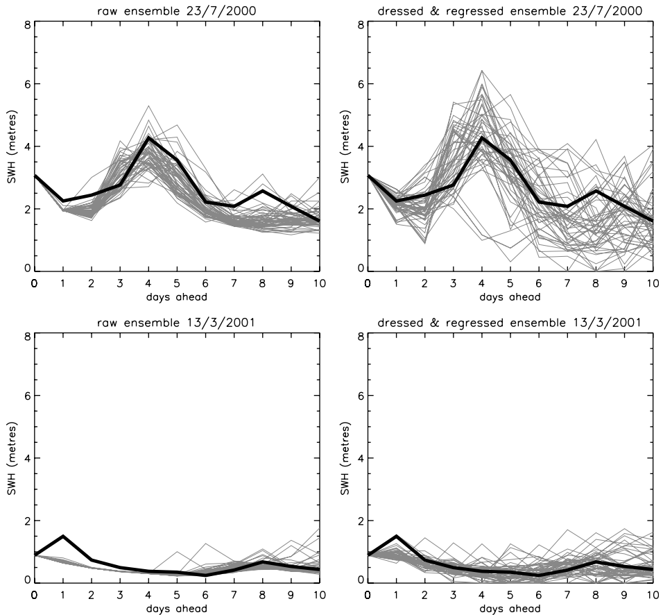
Fig. 2. An example of the impact of post processing on the raw 51-member ECMWF ensembles of significant wave height. The panels on the left show unprocessed ensemble forecasts for SWH at Maui for two different days. The panels on the right show the corresponding regressed and dressed forecasts. The thick black curve is the corresponding analyses. Notice that post-processing widens the distribution of ensemble members, and in doing so makes it a better representation of the actual forecast error, although this cannot be properly demonstrated using individual forecasts.
