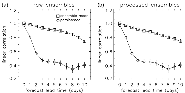
Fig. 3. The linear correlation between the ensemble means and the analyses for the Bonga site for the period March 1999 to December 2001 for significant wave height. The left panel is the correlation between the mean of the unprocessed ECMWF ensemble and the analyses, while the right panel is the correlation between the mean of the regressed and dressed ensemble and the analyses. The skill of a persistence forecast (assume current conditions persist) is shown for comparison. Note that post-processing has little impact on this measure of the skill of the ensemble mean, this is not surprising as the post-processing is designed to improve predictions of forecast uncertainty, not of the ensemble mean. The error bars are standard error estimates obtained using bootstrap resampling of 20 day blocks.
