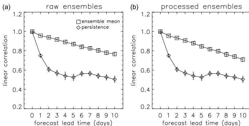
Fig. 4. As Fig. 3 but for Maui.
