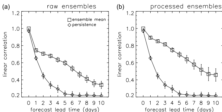
Fig. 5. As Fig. 3 but for the Campos Basin. In this case post-processing improves the skill of the ensemble mean at most lead times.
