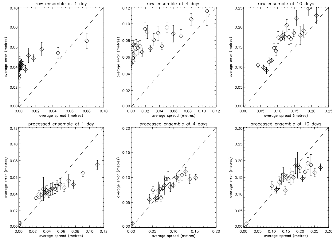
Fig. 7. A comparison of the spread-skill relationship of significant wave height forecasts at Bonga. Each point was obtained by calculating the average error of the ensemble mean of 70 ensembles between March 1999 and December 2001 with similar ensemble spreads. The dashed lines are the lines along which the points would be expected to fall if the ensembles were perfect. Points above this line correspond to cases when the ensemble spread underestimates the true error, points below this line mean that the ensemble spread is larger than the true error. The top panels show the spread-skill relationship for the raw 51-member ECMWF ensembles, while the bottom panels show the relationship for a 51-member ensemble obtained by regressing and dressing the raw ensemble. The error bars represent the standard error estimates obtained by bootstrap resampling. Note that the raw ensembles generally underestimate the error. The processed ensembles provide a better indication of the expected forecast error, although there is a tendency for them to overestimate the larger errors.
