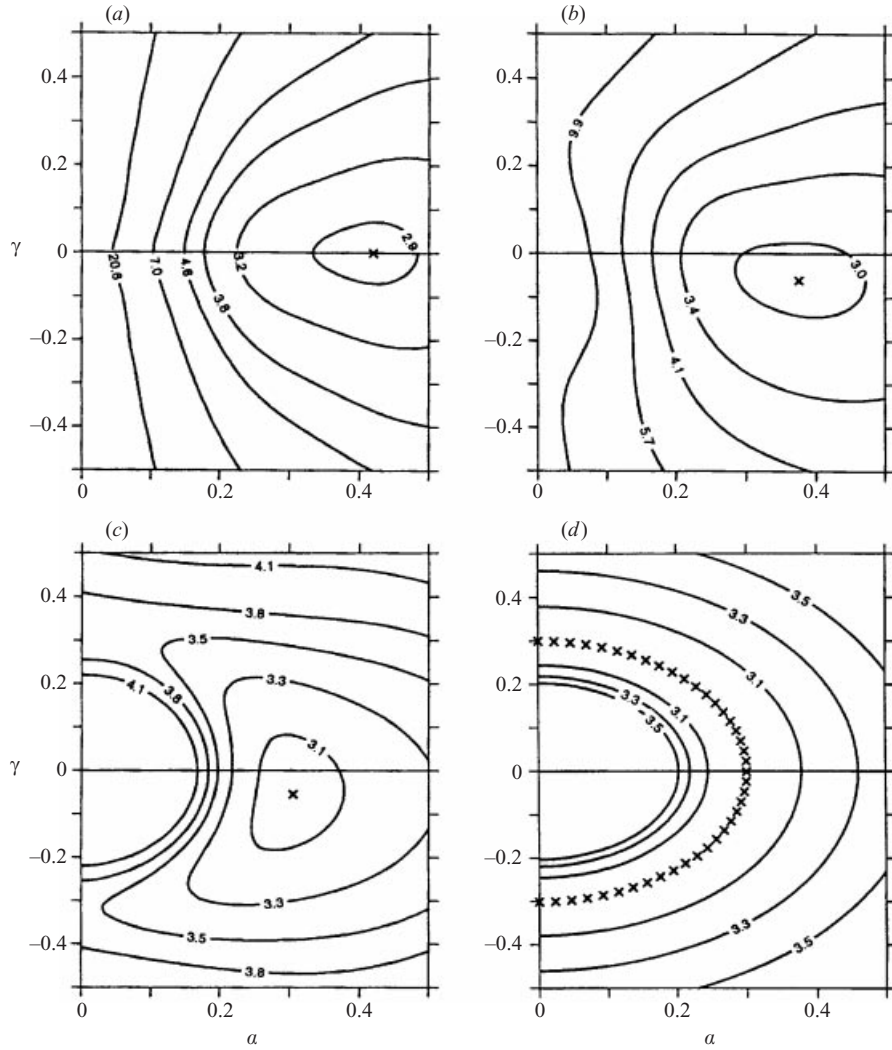
FIGURE 2. Contour plots of the marginal stability surface \Psi_{\text{marg}}(\alpha, \gamma) for different values of \sigma and R_b = 30 , R_d = 10 . Crosses indicate critical wavenumber(s) (\alpha_{\text{crit}}, \gamma_{\text{crit}}) . (a) \sigma = 0 , symmetric with respect to the line \gamma = 0 ; (b) \sigma = 0.5 and (c) \sigma = 0.9 , where the symmetry is lost and \Psi_{\text{crit}} is found off the line \gamma = 0 ; (d) \sigma = 1 , obeying rotational symmetry, where the critical wavenumbers form a semicircle.
