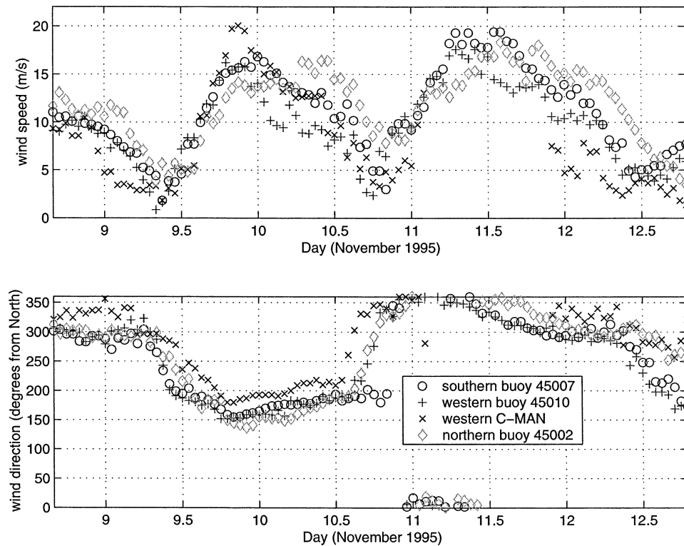
FIG. 6. Lake Michigan wind data at four instrument locations. Wind speed has been converted from 5- to 10-m altitude using a power-law relation. Direction is measured clockwise from north (NDBC notation).
