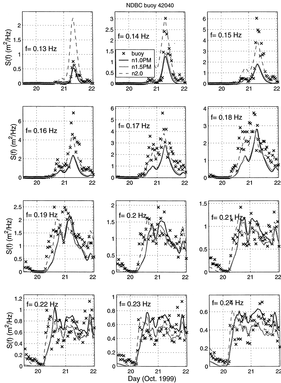
FIG. 10. Mississippi Bight time series of frequency spectra at location of NDBC buoy 42040. The SWAN models are compared with measurements. The n1.0PM,NDS model is not included in this comparison, because it is practically identical to the n1.0PM model in this simulation.
