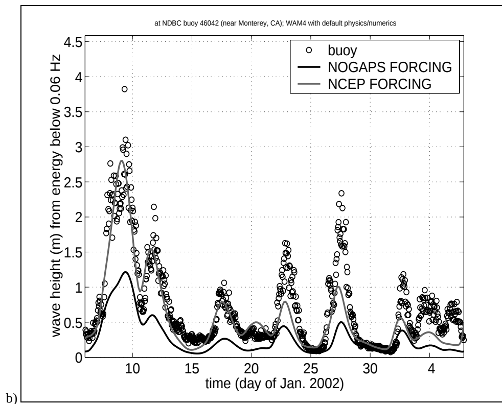
Fig. 1. Comparison of wave model hindcasts vs. buoy measurements. Location is buoy 46042, near Monterey, CA. Both WvW3 and WAM4 here are applied with default physics and numerics. Forcing is provided by analyses as indicated in figure legends. A) WvW3, B) WAM4.
