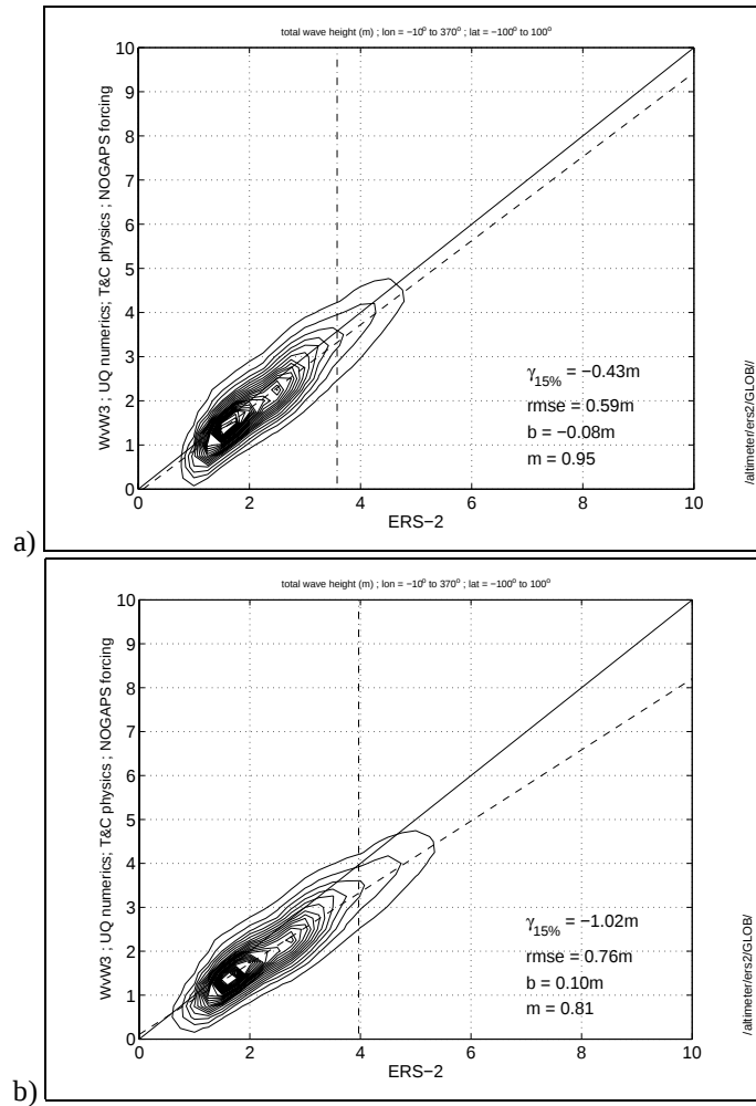
Fig. B2. Wave height comparison of WvW3 model hindcasts (default physics, numerics, January/February 2002) with NOGAPS (analyses) forcing vs. ERS-2 for the globe. A) Fast Delivery ERS-2 (FD); B). FD ERS-2 Corrected using Cotton equations (FDC).
