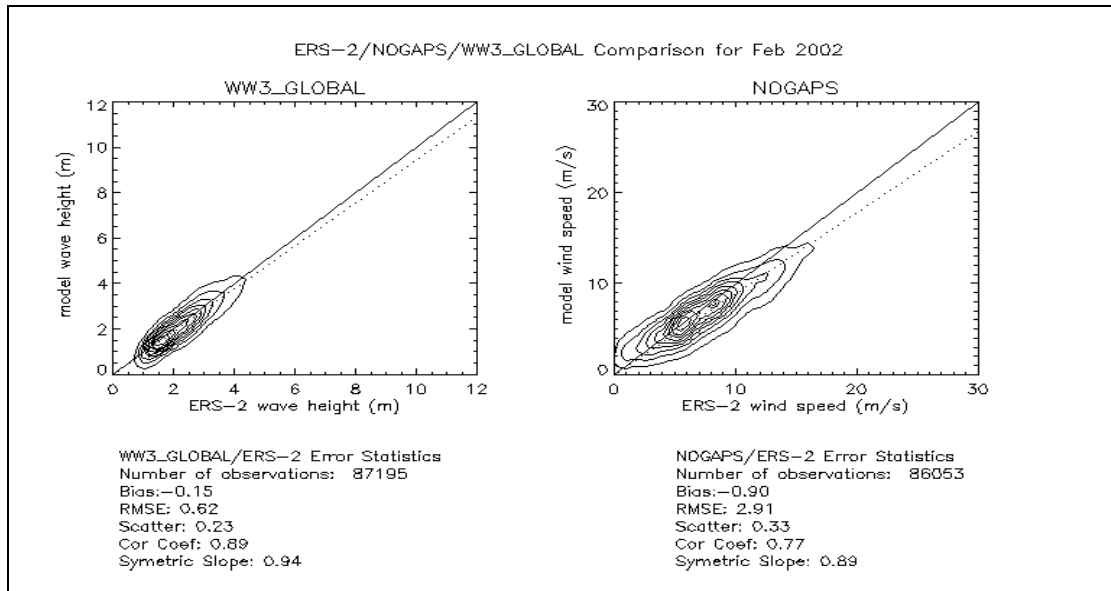
Fig. 12. FNMOC comparison for February 2002. These are the operational global wind and wave products (analyses) compared to FD ERS-2 globally. Standard definitions are used for statistics:
