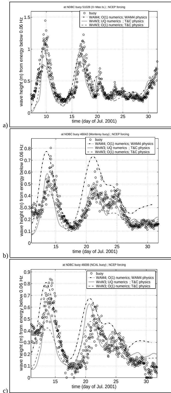
Fig. 2. Comparison of wave model hindcasts vs. buoy measurements. All models use NCEP analyses for forcing. A) Christmas Island buoy location, B) Monterey buoy, and C) northern California buoy.
