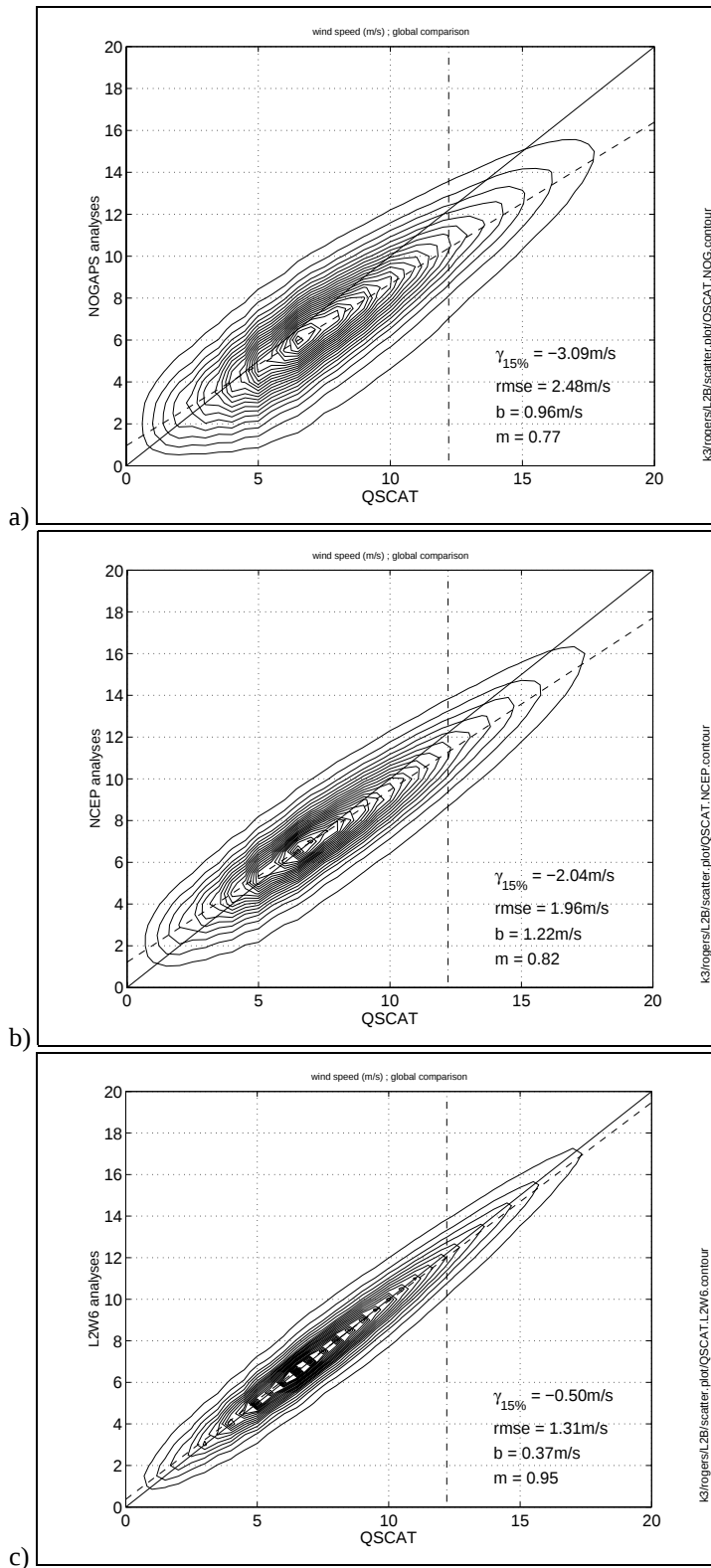
Fig. A1. Wind speed comparison of vs. QuikSCAT (PODAAC L2B) for the globe. A) NOGAPS analyses; B) NCEP analyses, C) L2W6 analyses. Only NOGAPS analyses are entirely independent of QuikSCAT data. See text for further explanation.
