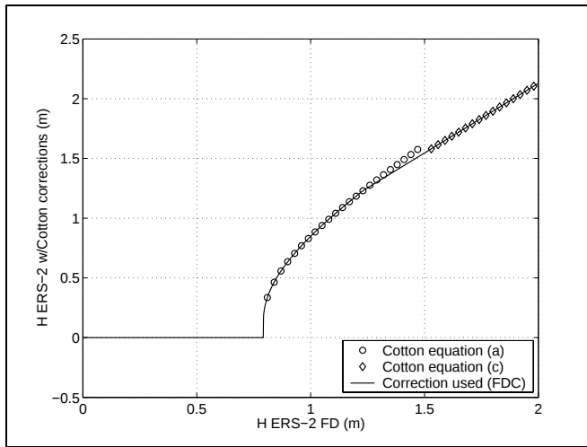
Fig. B1. Explanation of ERS-2 correction used in this study.
