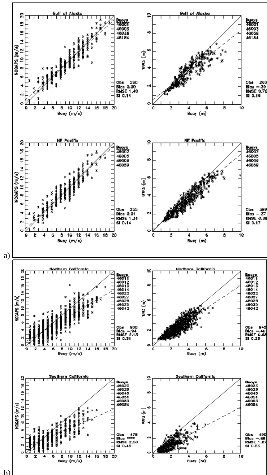
Fig. 5. FNMOC comparison for January 2002. These are the operational global wind and wave products (analyses) compared to buoys, by region. This is one of several comparisons that are made monthly. a) the “northeast Pacific” and “Gulf of Alaska” grouping, b) the “northern California” and “southern California” buoy groupings.
