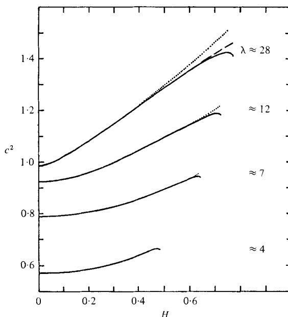
FIGURE 1. Comparison between the present method and the results of Cokelet (1977) for the wave speed squared, c^2 , as a function of wave height H . Present method: N = 8 (· · ·), N = 16 (---), N = 32 indistinguishable from Cokelet's results (—) at this scale. Each curve is drawn for a constant value of kQ/c taken from Cokelet's tables A2, A4, A6, A8, giving the almost constant values of wavelength shown.
