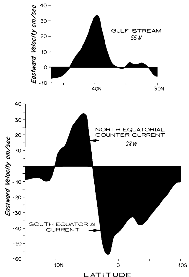
Fig. 2. Average yearly eastward surface velocity in the Gulf Stream near 55°W and average for July in the North Equatorial Countercurrent (NECC) and South Equatorial Current (SEC) near 28°W from historical ship drifts. Both sections are approximately 20° in longitude east of where the Gulf Stream and NECC leave the western boundary and have the swiftest currents. The amplitude and shape of the near-surface Gulf Stream and NECC are remarkably similar. Two major differences are the seasonal reversal of the NECC and the large shear between it and the South Equatorial Current.
