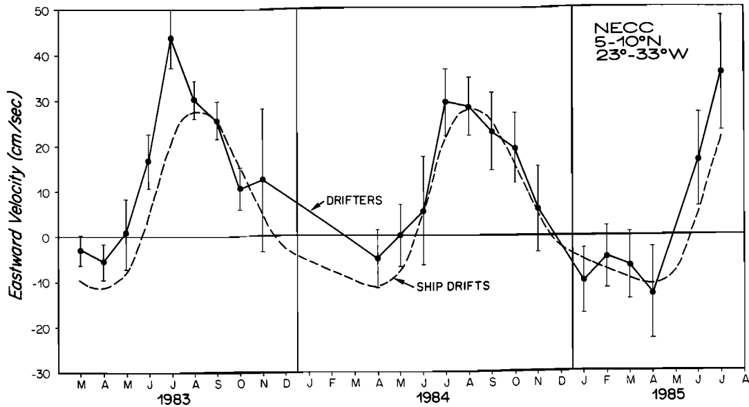
Fig. 14. Time series over 2\frac{1}{2} years of eastward velocity in the NECC. Average seasonal variation from historical ship drifts during 1875–1976 is included. Individual drifter and ship drift velocities were grouped into monthly averages in a box which extended from 5^{\circ} to 10^{\circ}\text{N} and from 23^{\circ} to 33^{\circ}\text{W} . Values from months with fewer than 40 observations were omitted. Error bars indicate estimated standard errors.
