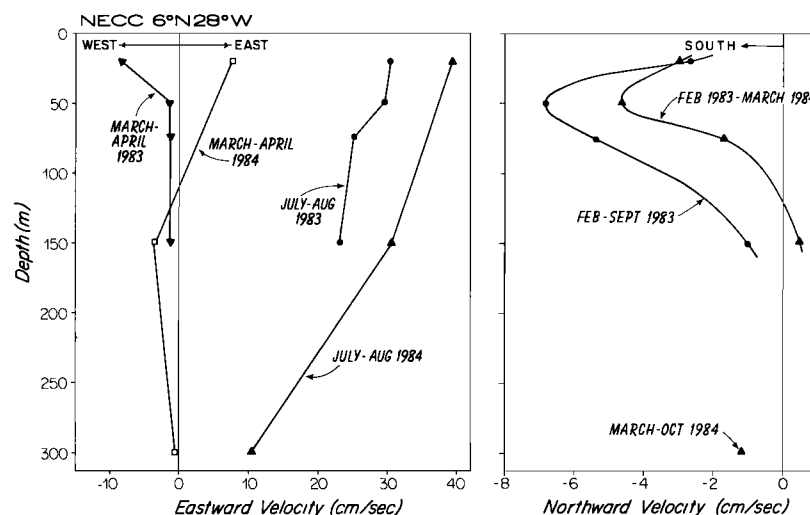
Fig. 10. Vertical profiles of velocity obtained from the current meter mooring at 6^\circ N, 28^\circ W (see Figure 16). The July–August profiles were chosen to match the time of maximum eastward subsurface velocity. The March–April profiles match times of minimum eastward velocity. The 300-m 1984 value is an average over April. The standard error in u at 20 m is estimated to be approximately 13 cm/s for these short pieces of the records. Profiles of northward velocity were averaged over longer time series because little seasonal variation was seen in the records. The standard error in v at 50 m is estimated to be approximately 3 cm/s.
