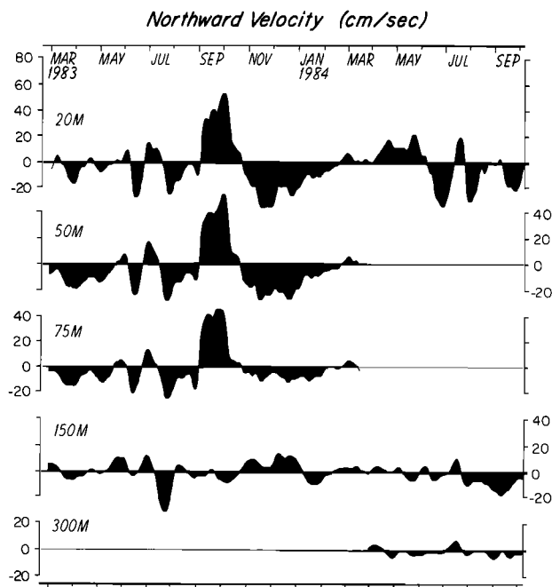
Fig. 17. Northward velocity time series from current meters.
