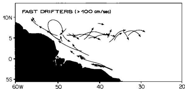
Fig. 6. Segments of trajectories of buoys that drifted faster than 100 cm/s after being smoothed with a 10-day filter to suppress inertial oscillations. Fastest speeds (2-day smoothing) were 167 cm/s in the North Brazil Current near the equator and 143 cm/s in the western NECC.
