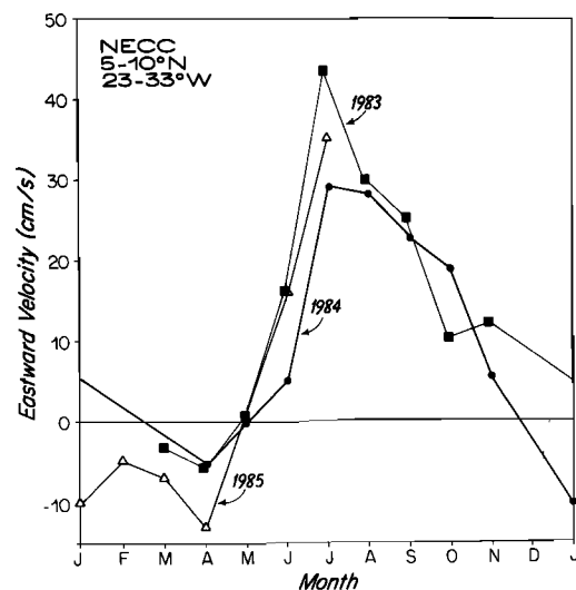
Fig. 15. Superposition of the NECC time series. The year-to-year differences are smaller than the standard errors. Some of these differences could be caused by a particular grouping of drifters within the box and the presence of energetic high-frequency oscillations.
