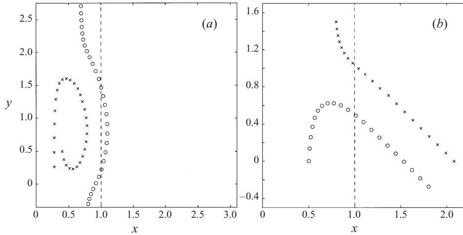
FIGURE 6. The motion of an equal and opposite vortex pair along a shoreline. The profile of this shoreline is plotted in figure 3(b). The positions of the vortices (of strengths \Gamma = 1 ( \times ) and \Gamma = -1 ( \circ )) are given at evenly spaced times 0.05 units apart are shown. In (a) the positive vortex ( \times ) starts from position (0.4, 0.5) and the negative one at the bottom of the picture. The same assumption about the initial distribution of vorticity within the core is used as used in figure 5 and it follows that here \epsilon = 0.1 and \mathcal{P} = 5\Gamma^2/4 .
