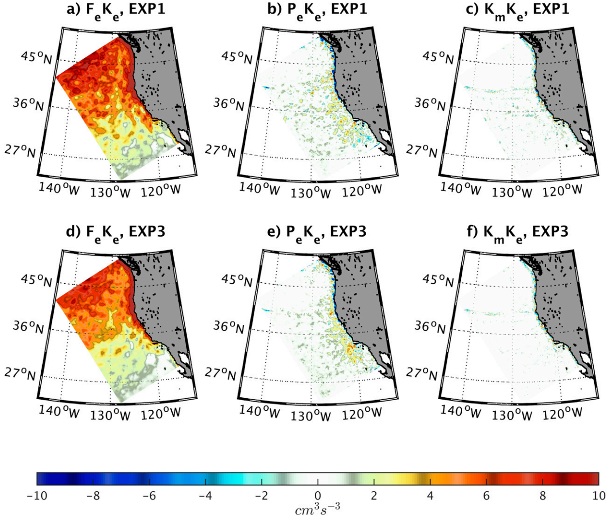
FIG. 2. Depth-integrated EKE-budget components ( \text{cm}^3 \text{s}^{-3} ) from (top) EXP1 and (bottom) EXP3: (left)–(right) the eddy wind work F_e K_e , the baroclinic conversion P_e K_e , and the barotropic conversion K_m K_e . The main energy source terms are F_e K_e and P_e K_e . The reduction of the EKE in Fig. 1 is explained by the reduction of F_e K_e by the current feedback.
