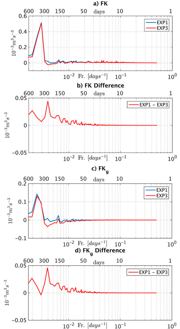
FIG. 7. (a) Temporal 1D cospectrum of the total wind work FK from EXP1 and EXP3 between 30^{\circ} and 45^{\circ} N for the offshore region ( d > 80 km). (b) Difference between EXP1 and EXP3. (c), (d) As in (a), (b), but for the geostrophic wind work. The current feedback to the atmosphere acts as an eddy killer by reducing F_e K_e through its geostrophic component, deflecting energy from the ocean to the atmosphere.
