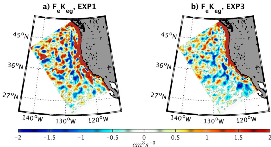
FIG. 4. Geostrophic eddy wind work F_e K_{eg} from (a) EXP1 and (b) EXP3. The reduction of F_e K_{eg} is mainly explained by a coastal reduction of F_e K_{eg} and an offshore sink of energy through F_e K_{eg} .
