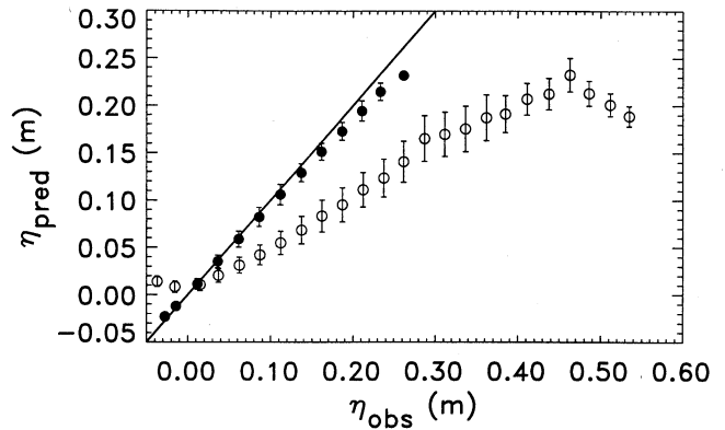
Figure 6. Predicted versus observed mean (circles) and standard deviation (vertical bars) of 512 s setdown and setup in total water depths of less than (open circles) and greater than (solid circles) 1 m.
