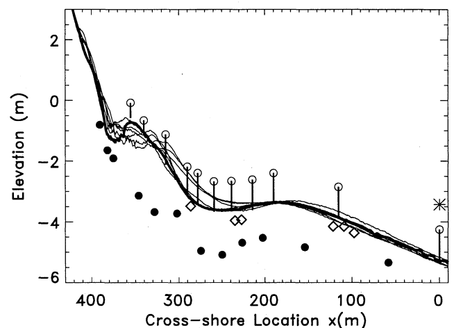
Figure 1. Locations of deeply buried pressure sensors used to measure setup (solid circles), colocated unburied pressure sensors, current meters, and sonar altimeters (open circles), near-bed pressure sensors (open diamonds), and the conductivity sensor (asterisk). The most seaward 11 setup sensors were accurate Paroscientific gages. All pressure measurements were corrected for temperature effects. The solid curves are selected beach profiles measured between 1 September and 31 November. The thick black curve is the 13 September profile. The x axis is positive onshore with the origin at the location of the offshore sensor.
