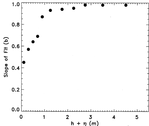
Figure 7. Slope of least squares fit of setup predictions to observations ( b in Table 1) versus total water depth ( h + \eta ).
