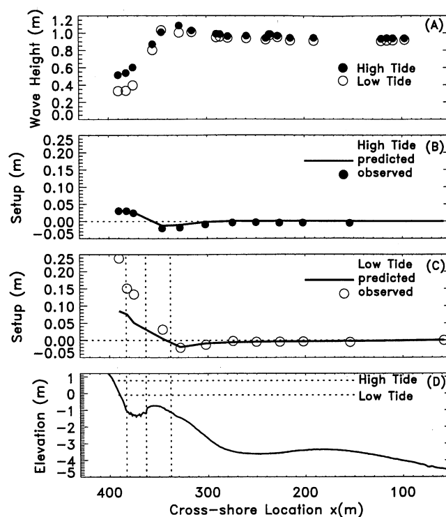
Figure 4. (a) Observed significant wave heights on 13 September, and observed (open circles) and predicted (solid curve) setdown and setup on 13 September at (b) high tide (1600) and (c) low tide (2042), and (d) measured beach profile versus cross-shore location (times represent the start of each 512 s record). The vertical dotted lines in Figures 4c and 4d mark the locations x = 338 , 363 , and 383 m discussed in the text. The horizontal dotted lines in Figures 4b and 4c are still water level. The horizontal dotted lines in Figure 4d are tidal elevations during the two runs.
