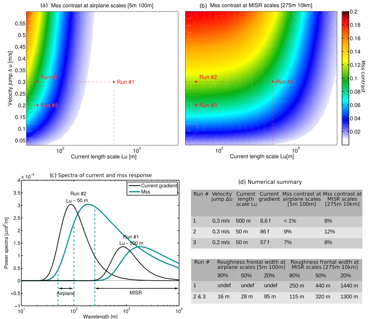
Figure 7. (a) Amplitude of the modeled mss response at scales in the range [5m, 100m], as function of the imposed current length scale L_u and velocity jump \Delta u . Location of the Runs 1, 2, and 3 are highlighted with the red dashed lines. (b) Same as (a) but for scales in the range [275m, 10km]. (c) Spatial power spectra of the current gradient \partial u / \partial x (black curves) and of the corresponding mss contrast (cyan curves), for the numerical model Runs #1 and #2. The ranges of scales observed by airplane and by MISR are also shown with double head arrows. Note that for display purposes, each spectrum of mss response has been normalized to match the maximum value of the corresponding imposed current spectra. (d) Summary of the numerical results for the three specific model Runs #1, #2, and #3.
