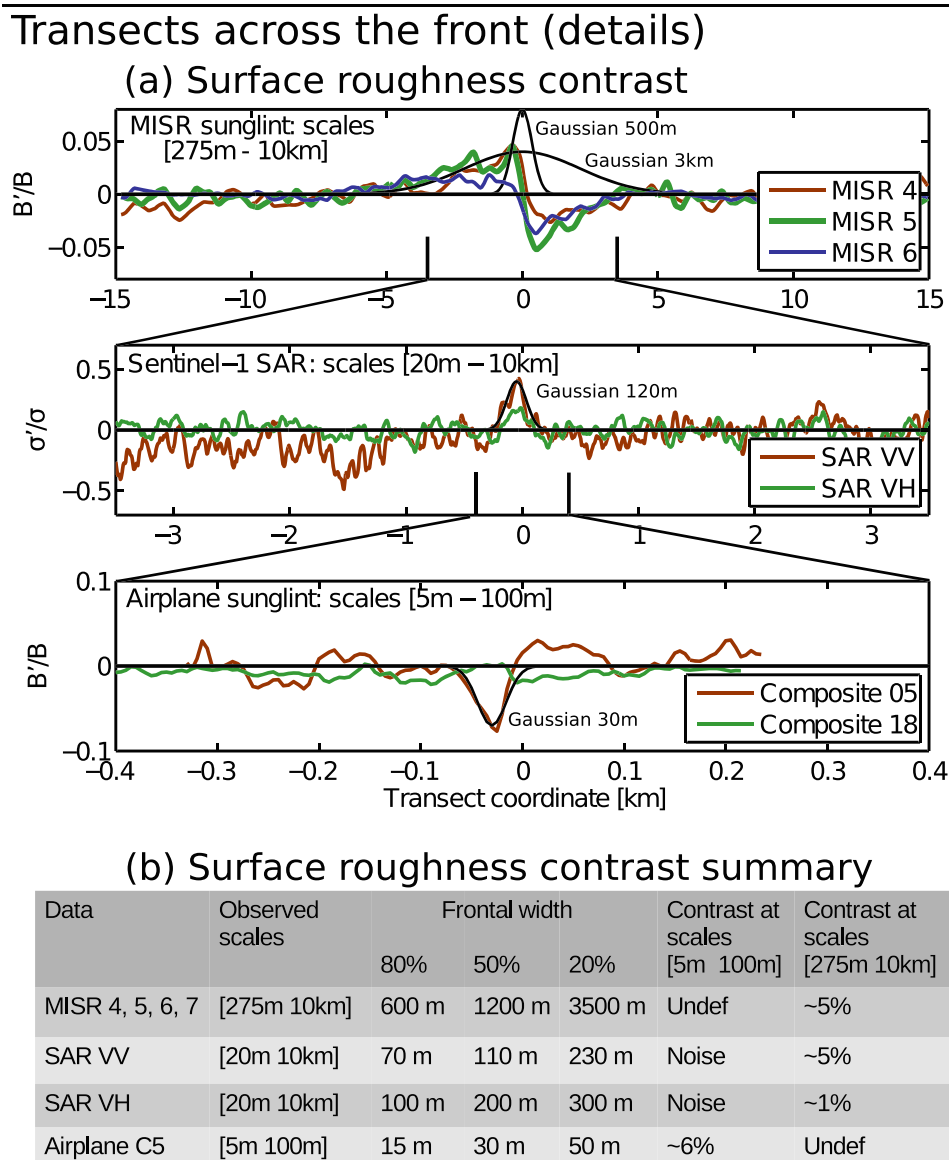
Figure 5. (a) Similar to Figure 4a (transects of the observed surface roughness across the front) but note that the three horizontal axes do not have the same scales. To help the interpretation, Gaussian fits (with standard deviations in meters) are added as thin black curves. (b) Table summarizing the horizontal extensions and amplitudes of the observed roughness contrasts at the front. The roughness frontal width at 80% (resp. 50% and 20%) is defined as the spatial extension over which the roughness contrast (in absolute value) reaches more than 80% (resp. 50% and 20%) of the maximum contrast at the front.
