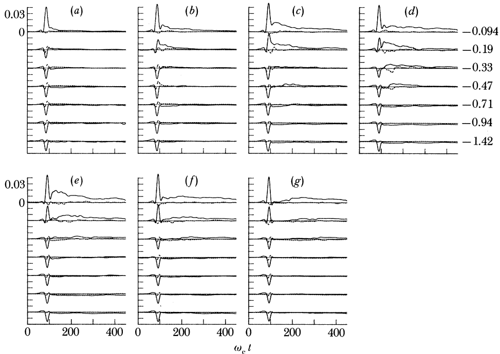
FIGURE 44. Time series of mean horizontal \langle \bar{u} \rangle / C , — and vertical \langle \bar{w} \rangle / C , ---- velocity for f_c = 0.88 Hz. k_c(x - x_{0h}) is (a) 1.9, (b) 2.7, (c) 3.8, (d) 4.7, (e) 5.7, (f) 6.6, (g) 7.6. The numbers on the graph are values of k_c z .
