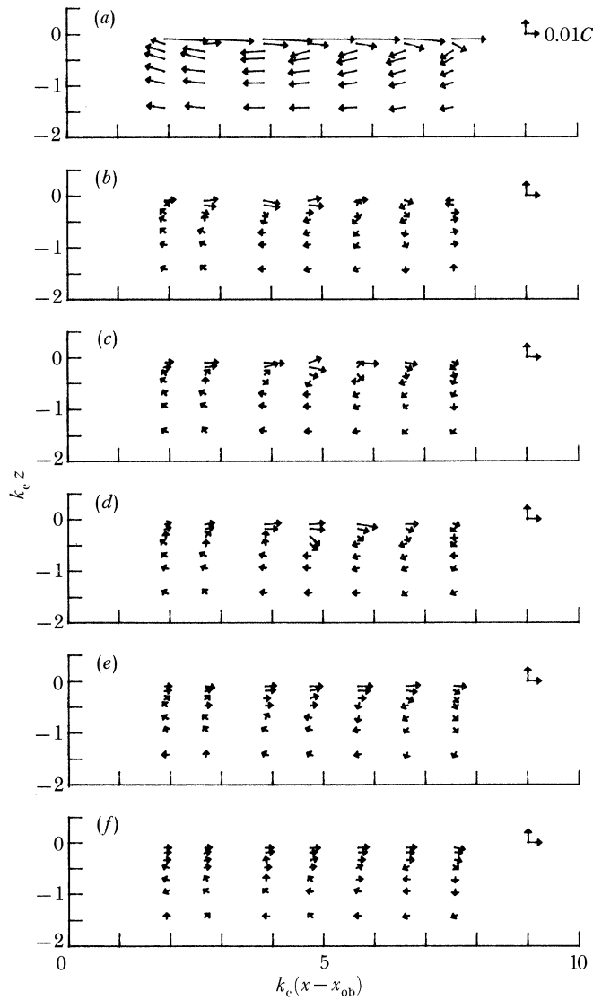
FIGURE 45. Mean velocity field for f_c = 0.88 Hz, ak_e = 0.278 (spilling) (a)–(f) as for figure 43.
