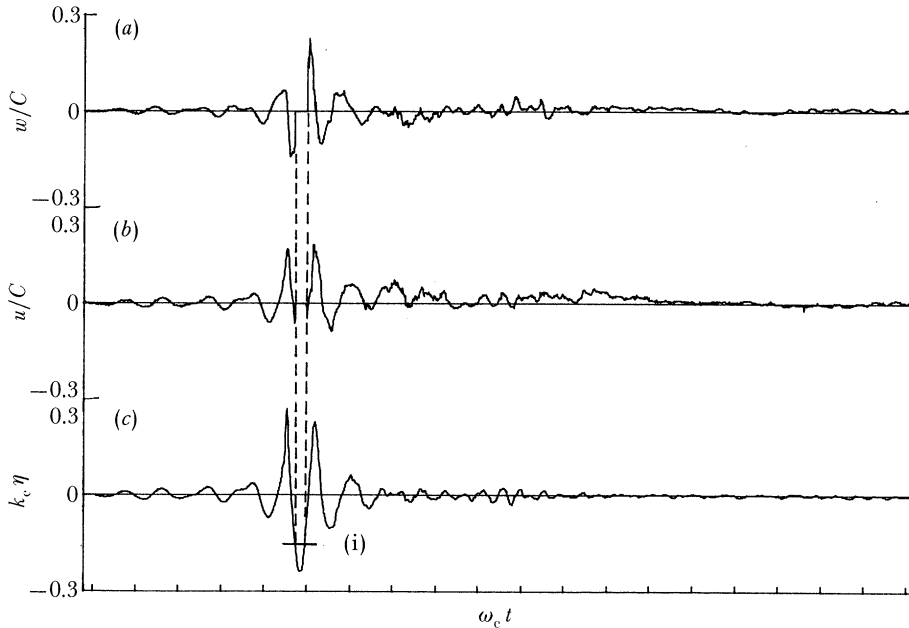
FIGURE 39. Coincident surface displacement and subsurface velocity measurement at k_c(x - x_{ob}) = 3.80 and k_c z = -0.16 downstream of plunging break. For f_c = 0.88 \text{ Hz} , ak_c = 0.352 , \Delta f/f_c = 0.73 , x_b k_c = 27.4 . C is the linear phase speed, k_c is the wavenumber corresponding to f_c for finite depth. (a) Vertical velocity, (b) horizontal velocity, (c) surface displacement, (i) elevation of velocity probe volume.
