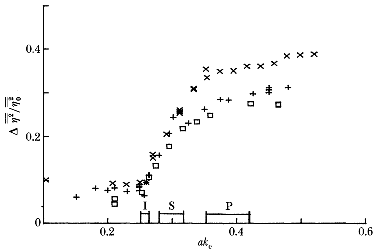
FIGURE 15. Loss of excess momentum flux as a function of the wave packet amplitude for three packet centre frequencies f_c = 0.88 Hz (x), 1.08 (+), 1.28 ( \square ) and \Delta f/f_c = 0.73 , x_b k_c = 27.4 . Occurrence of incipient breaking, single spilling, and plunging are marked by I, S, P with variations between scales shown by horizontal bars.
