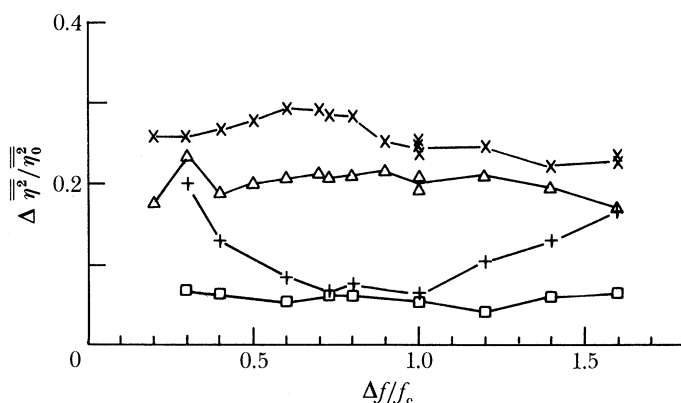
FIGURE 16. Loss of excess momentum flux against the wave packet bandwidth \Delta f/f_c for four input wave amplitudes, ak_c = 0.151 ( \square ), 0.257 ( + ), 0.296 ( \triangle ), 0.388 ( \times ) and f_c = 1.08 . These correspond to a non-breaking packet, incipient breaking, a single spill, and a single plunging wave, respectively, for f_c = 1.08 , x_b k_c = 27.4 and \Delta f/f_c = 0.73 .
