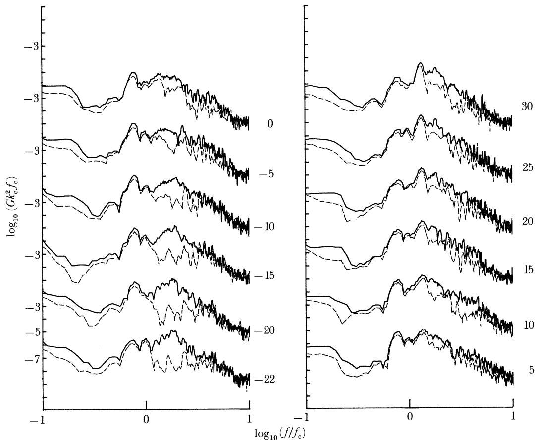
FIGURE 28. Spectra of waves radiated away from breaking disturbance f_c = 0.88 Hz, ak_c = 0.352 , plunging —, ak_c = 0.257 , incipient breaking ---. 95% confidence interval for spectral estimates is equal to 1 unit on the left axis. The numbers on the graphs are values of k_c(x - x_b) .
