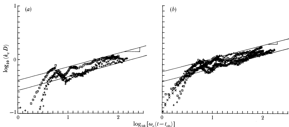
FIGURE 35. Log-log plot of maximum depth against time from observed breaking. Same symbols as figure 34. Plot shows fit of data to \omega_c(t-t_{ob})^{\frac{1}{4}} power law.
