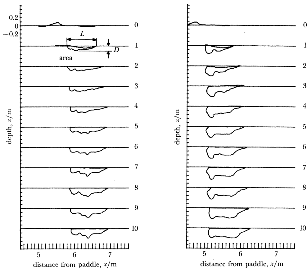
FIGURE 31 (left). Digitized data of dye boundary taken from ciné films. Wave packet with f_c = 1.08 Hz, k_c = 4.72 \text{m}^{-1} , ak_c = 0.296 (spilling). \Delta f/f_c = 0.73 , x_b k_c = 27.4 . Time steps are referenced from t_{ob} , time of observed breaking in seconds. Top contour is the free surface at breaking. Refer to table 1 for definition of t_{ob} . Numbers on right-hand side refer to t - t_{ob} .
