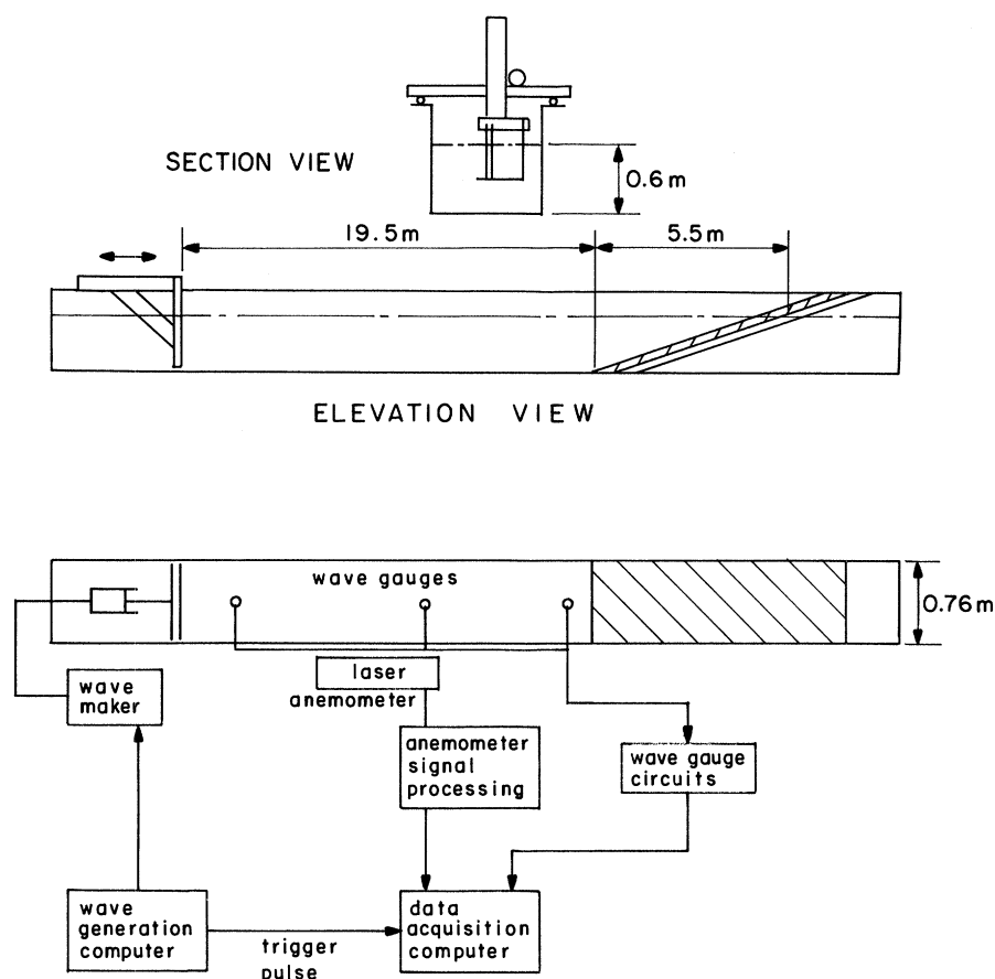
FIGURE 2. Wave channel and instrumentation.
