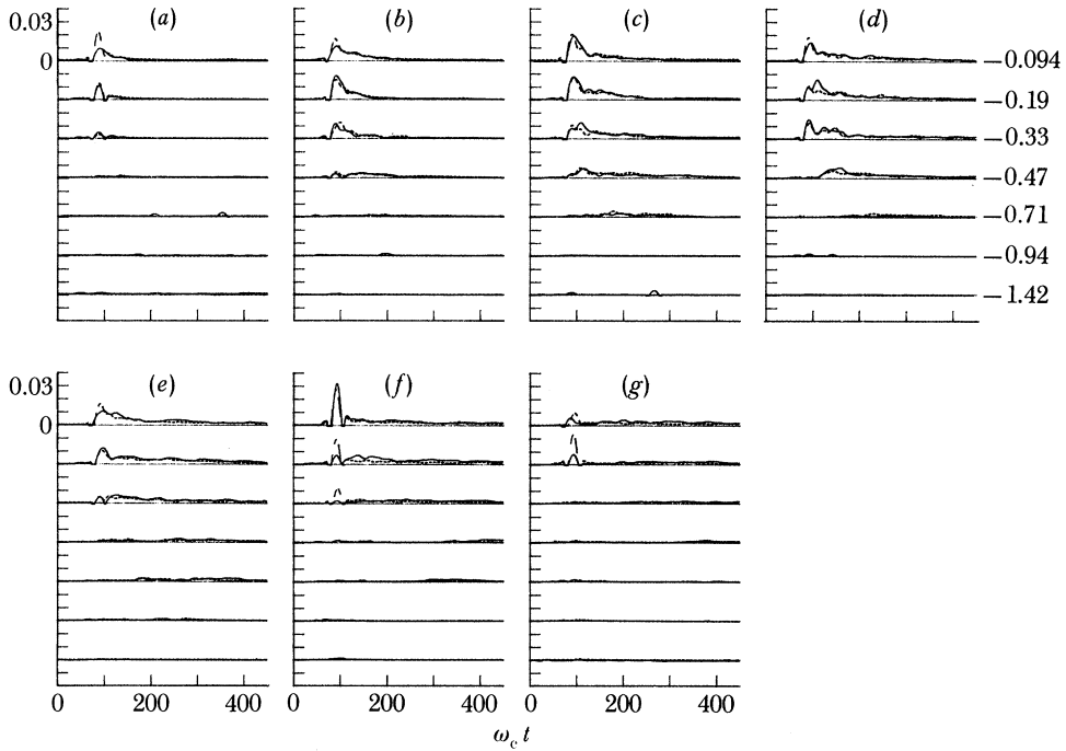
FIGURE 48. Time series of horizontal and vertical turbulence r.m.s. velocities (a)–(g) as for figure 46, except ak_c = 0.278 (spilling). The numbers on the graph are values of k_c z .
