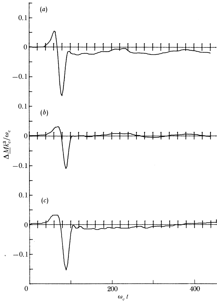
FIGURE 50. Total momentum in the breaking region as a function of time. f_c = 0.88 Hz with (a) plunge, (b) spill, (c) f_c = 1.28 Hz plunge.
