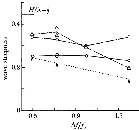
FIGURE 21. Spatial wave steepness measurements for incipient breaking. ak_c (○), a_{sb}k_c (△), \alpha = a_{sb}/L_t (□), \beta = \pi H/\lambda (∧). Refer to figure 20.
