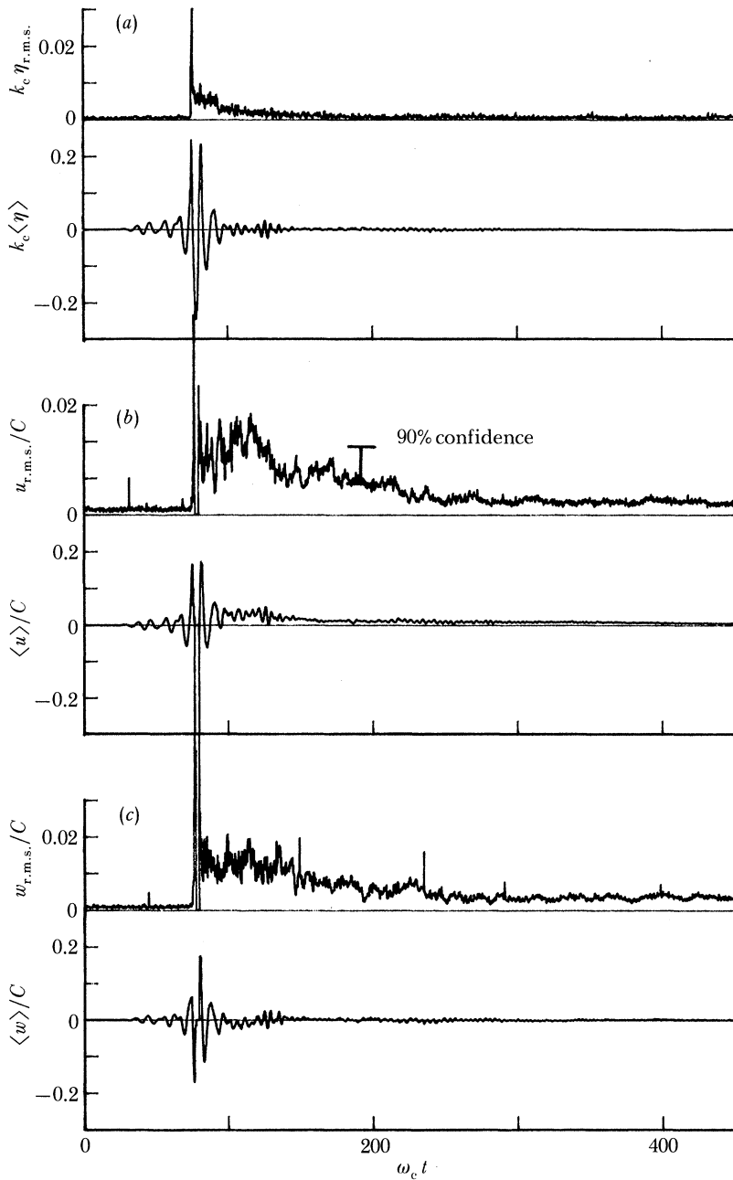
FIGURE 40. Ensemble averaged velocities \langle u \rangle , \langle w \rangle and surface displacement \langle \eta \rangle . Also the corresponding r.m.s. velocities, and surface displacement. Average of 10 repeats; same location as figure 39. (a) Surface displacement, (b) horizontal velocity, (c) vertical velocity.
