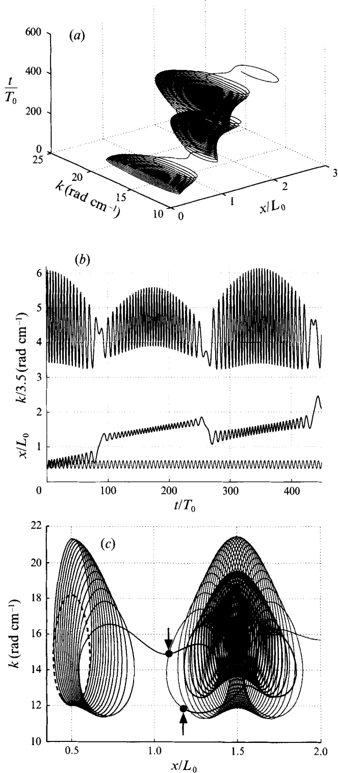
FIGURE 4. (a) Three-dimensional phase portrait of a capillary-gravity wave with initial wavenumber k_0 in the field of two long gravity waves. (b, c) Two-dimensional projections: (b) in the time-
