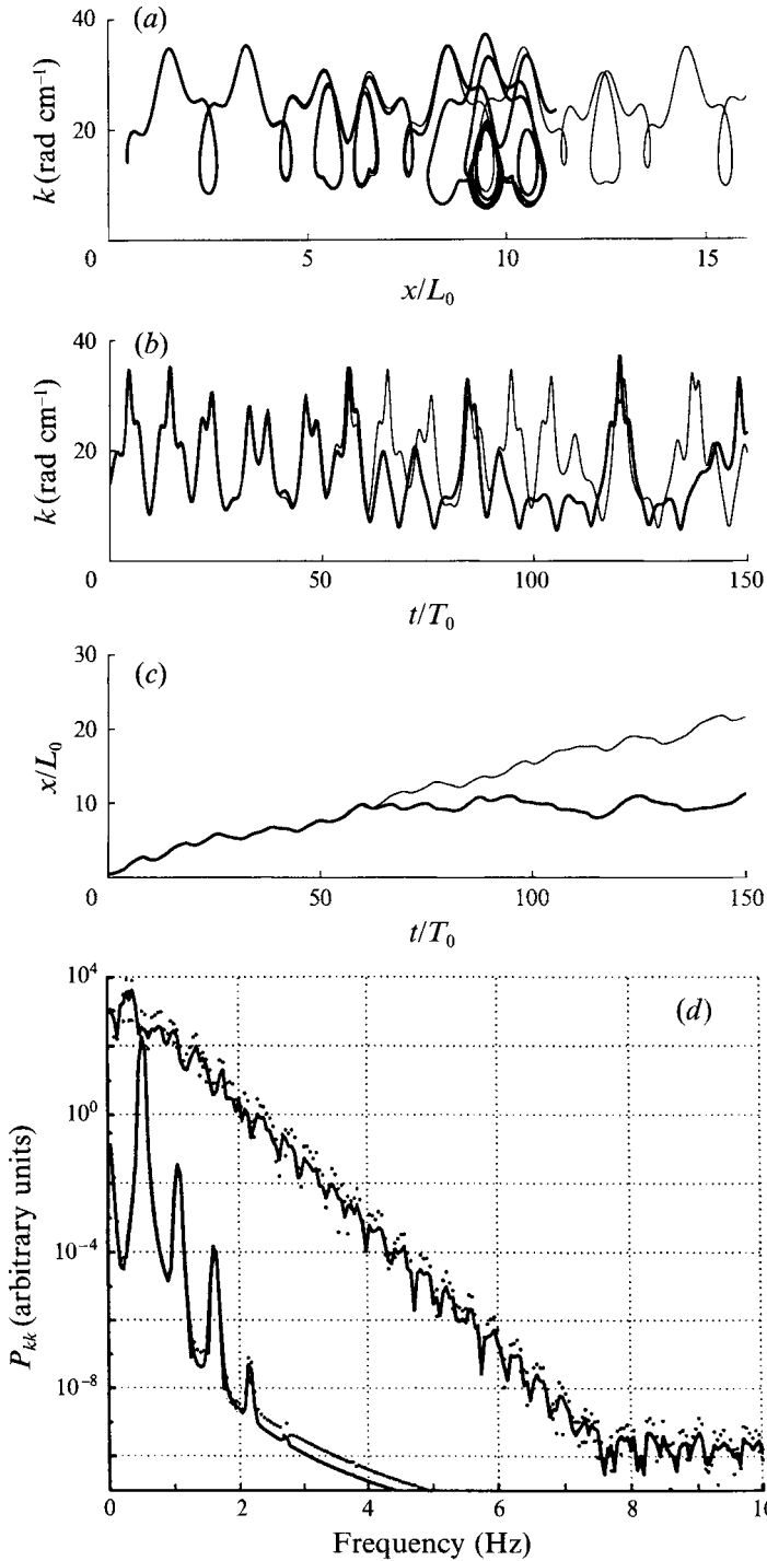
FIGURE 13. Short-wave trajectories in WKB phase space (a) and time evolutions of the wavenumber (b) and the position (c) corresponding to two slightly different initial conditions: k_0 = 14 rad cm -1 , x_0 = L_0/2 (light lines); k_0 = 14 + 0.01 rad cm -1 , x_0 = L_0/2 + 0.01 (heavy lines). (d) Frequency spectrum of the wavenumber variations with k_0 = 14 rad cm -1 , in the presence of a single long wave (lower curve) and in the presence of two long waves (upper curve \delta = 1/7 ); the dots display the 95 % confidence intervals.
