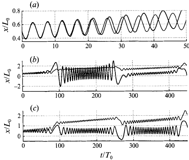
FIGURE 11. As figure 9(a) for \delta = 1/176 except that (23) is replaced by: (a, b), the inhomogeneous Mathieu equation (30) (heavy lines); (c) the homogeneous Mathieu equation (30) without the forcing term) (heavy line). The lighter lines are the exact solution, (15).
