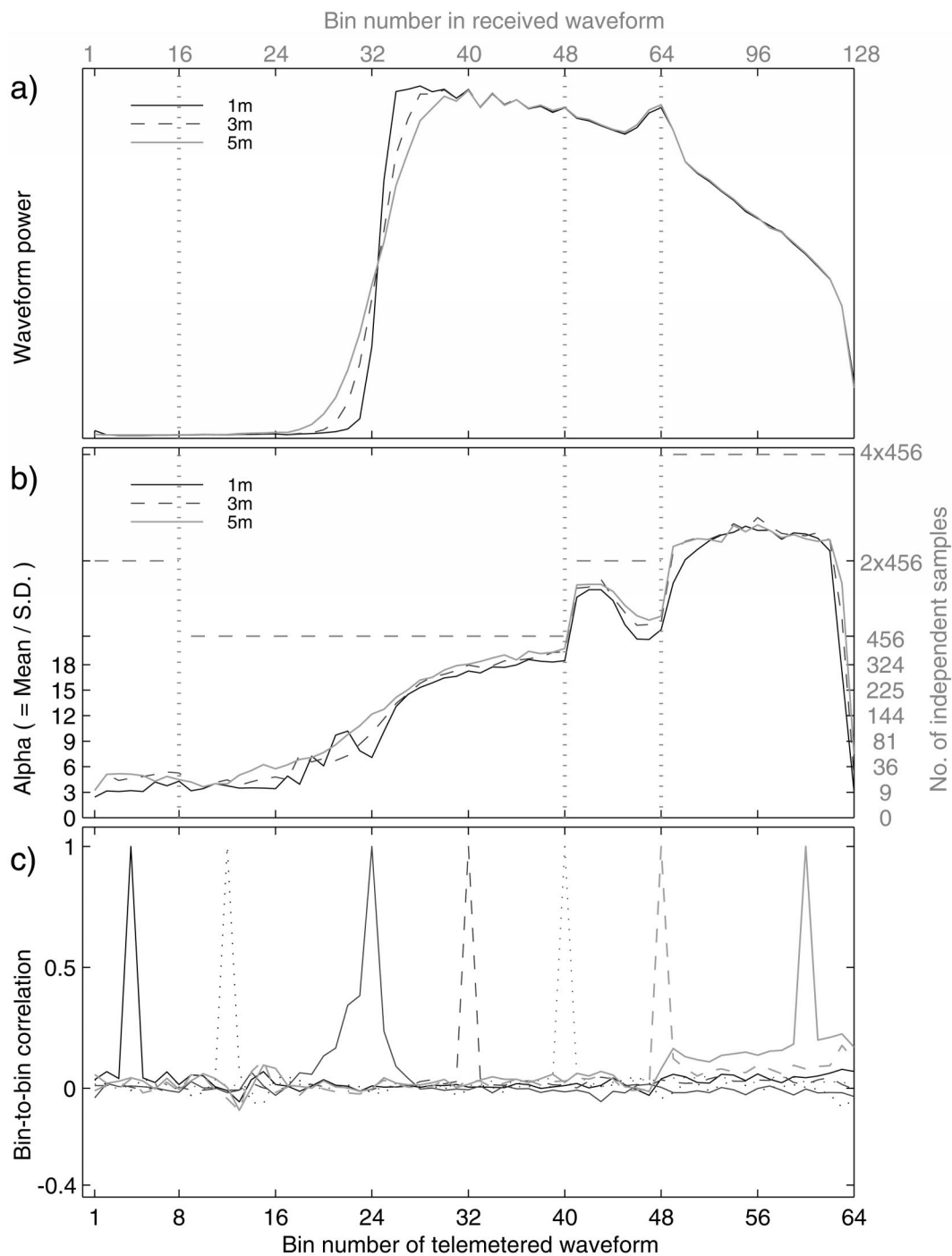
FIG. 5. TOPEX K_u band. (Description same as for Fig. 3, except bin numbering of received waveforms also provided at top, and the vertical dotted lines show the changes in transcription from received to telemetered.)
