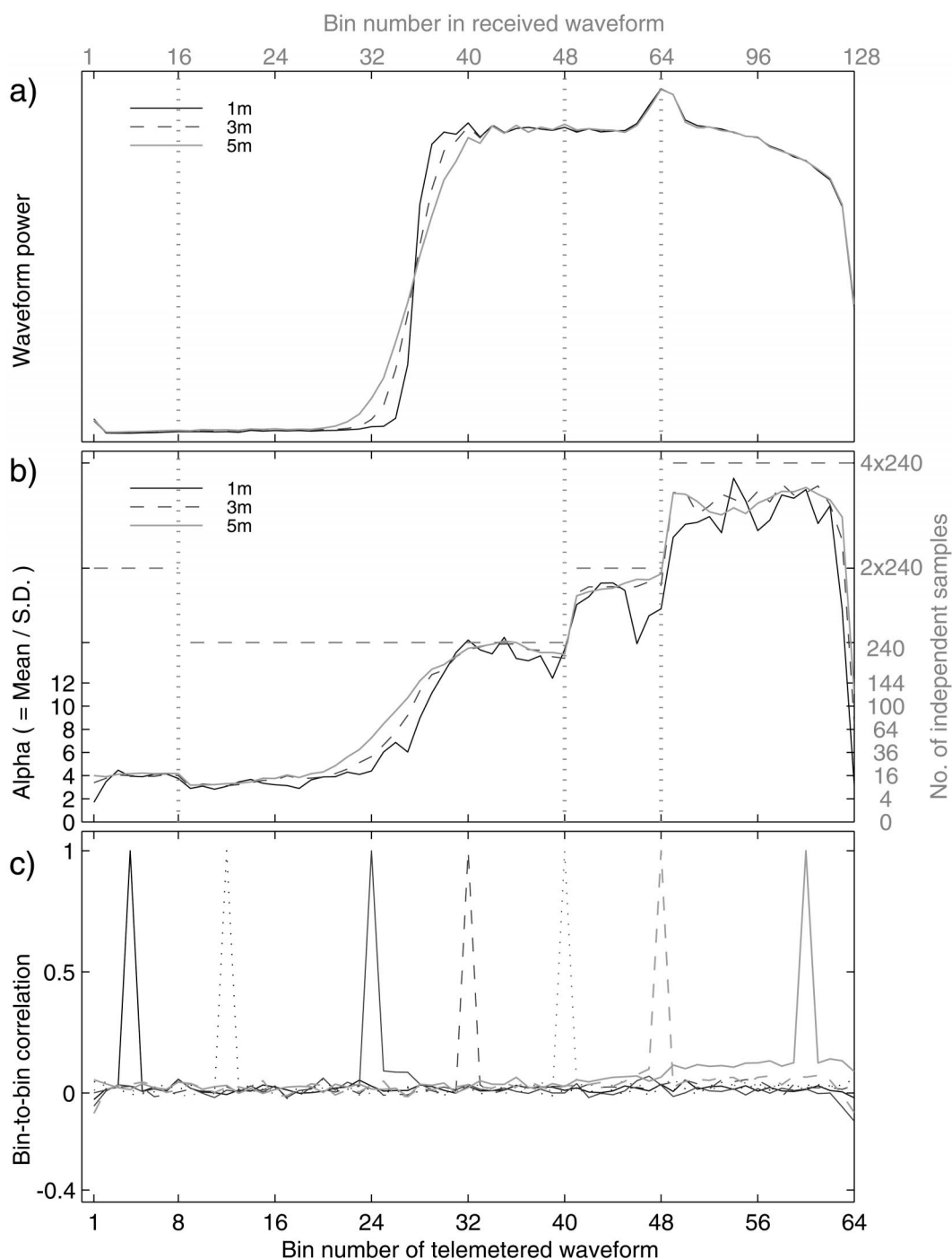
FIG. 6. TOPEX C band. (Description same as for Fig. 3, except bin numbering of received waveforms also provided at top, and the vertical dotted lines show the changes in transcription from received to telemetered.)
