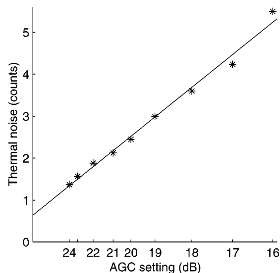
FIG. A2. Plot of power in thermal noise region (here average of bins 5–8) against adjusted AGC values on a logarithmic scale. (Data from cycle 186.)
