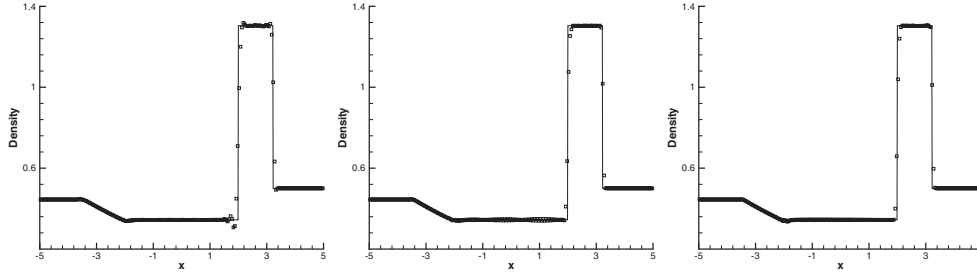
FIG. 7. Lax problem. t = 1.3 . RKDG with WENO limiters. 200 cells. TVB constant M = 50 . Density. Solid line: the exact solution. Squares: numerical solution (one point per cell). Left: k = 1 . Middle: k = 2 . Right: k = 3 .
