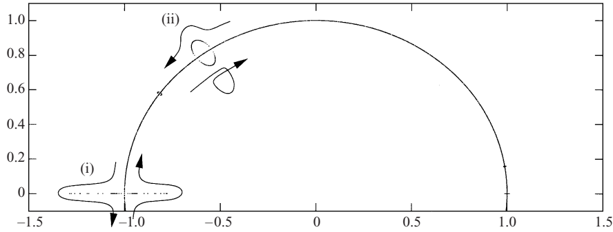
FIGURE 12. The trace of the eigenvalues in the complex plane for 0 < k_0 d < 5 corresponding to the results in figure 11. The arrows indicate the path two eigenvalues take as they meet on the unit circle.
