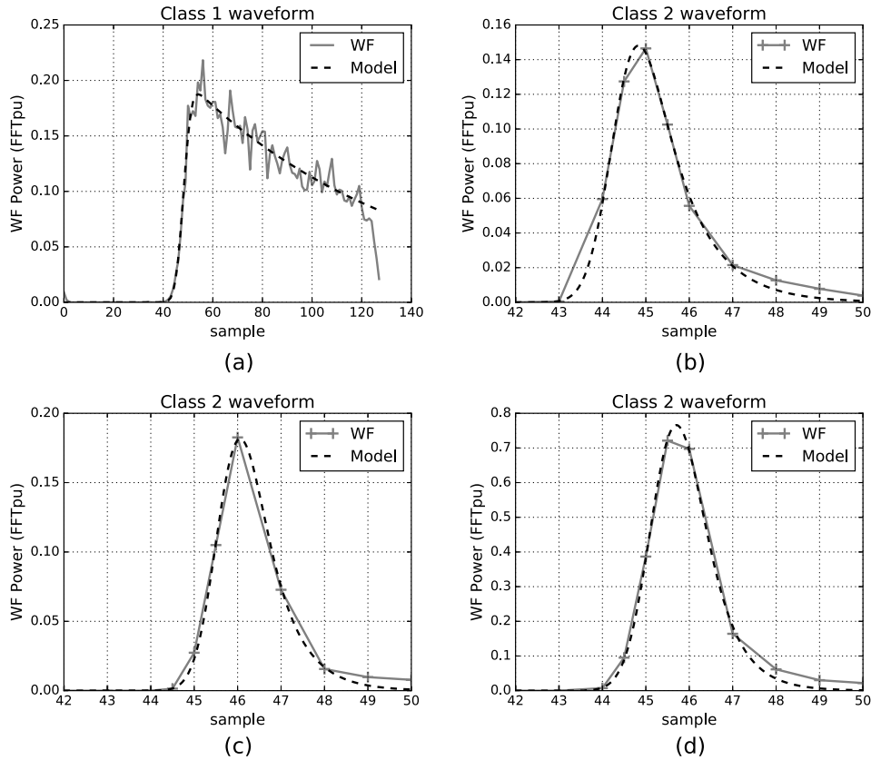
Fig. 10. Retracted modified Brown model superimposed on ENVISAT waveforms over (a) ocean and (b)–(d) three different sea-ice lead waveforms with their associated waveform class assigned by the neural network classification. The two DFT samples added by the RA-2 altimeter are considered and are localized at samples 44.5 and 45.5 (starting from 0).
