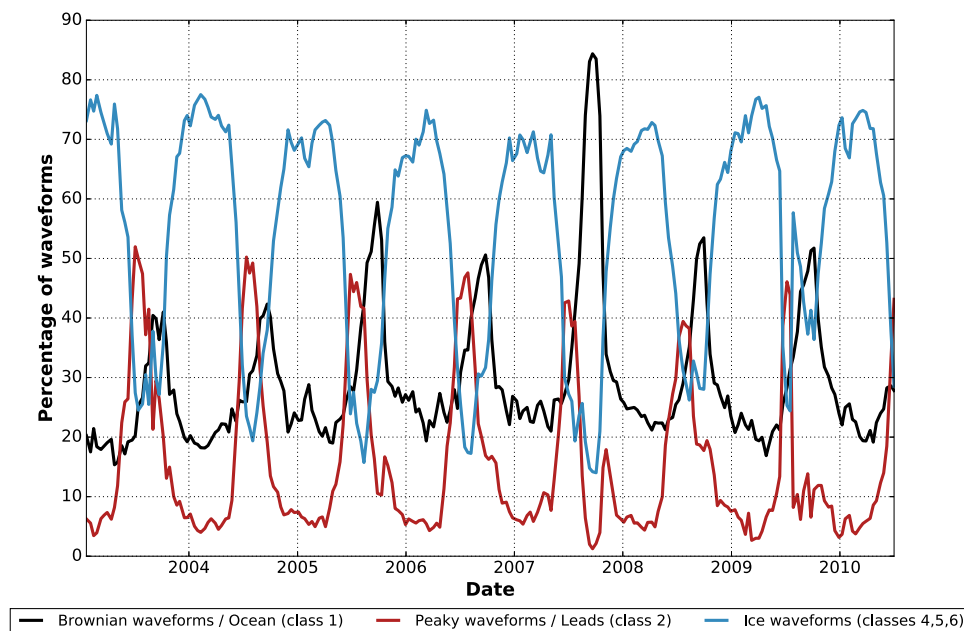
Fig. 5. Temporal evolution of the class proportion identified by the neural network algorithm during the ENVISAT period over the ocean above 60° of latitude.
