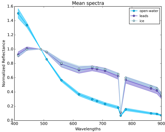
Fig. 7. Spectra normalized by value at 489.88 nm, with coloring according to the altimeter classification. Solid line: mean. Shading: \pm 1 s.d.
