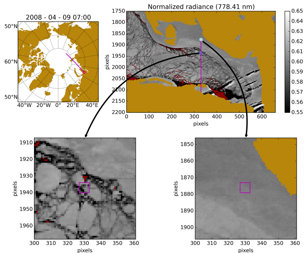
Fig. 6. Example MERIS data for April 9, 2008. (a) Map showing location of swath. (b) Zoomed-in view of region at southern end of track with pink line showing altimeter nadir view, orange indicating land, and red mark indicating cloud. (Note unflagged pixels in the bottom-right corner of image). (c) and (d) Details of regions of leads and ice floe, respectively, showing the greater spatial heterogeneity in the former. Pink box: example regions of 7 \times 7 pixels.
