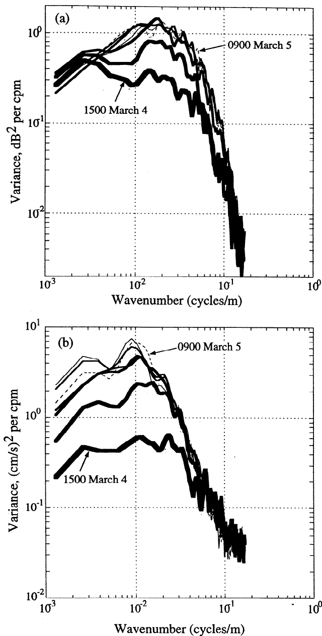
Figure 8. Time-lagged wavenumber spectra, analogous to wavenumber autospectra, except for the introduction of a 1-min time lag, from the Flip sonar beam directed most nearly crosswind. (a) A sequence of seven intensity spectra presented in 3-hour intervals starting just before the second wind event on March 5. (b) Velocity spectra from the same beam for the same time periods.
