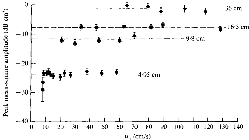
FIGURE 11. Maximum mean-square wave amplitude vs. the wind speed at which it occurs for various fetches.
