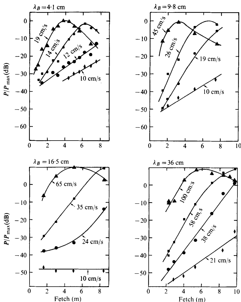
FIGURE 16. Normalized first-order Bragg peak intensity for several Bragg waves as a function of fetch at various u_* values.
