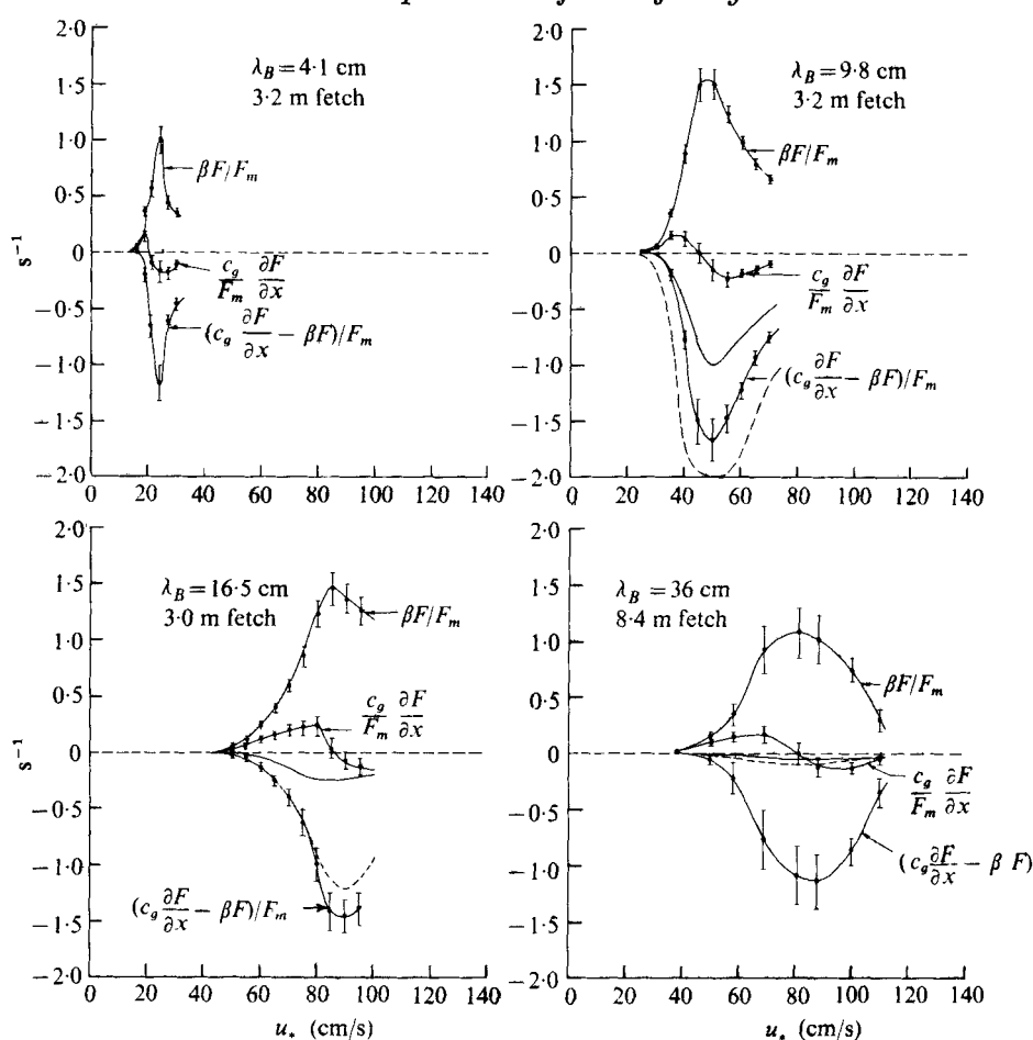
FIGURE 18. Normalized energy transfer curves. The unlabelled solid and dashed curves are values of S_{nl}/F_m calculated from second-order wave-wave interaction theory.
