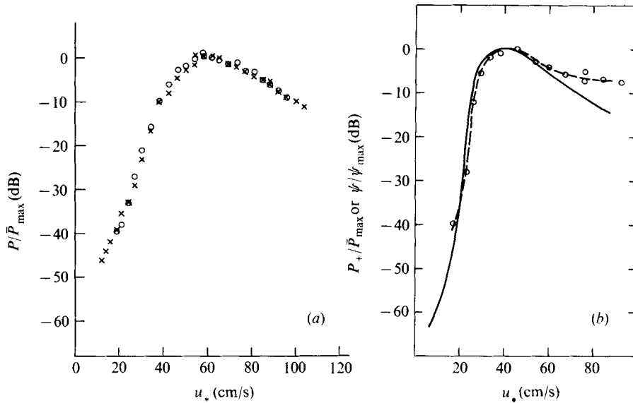
FIGURE 10. Spectral comparisons. (a) Normalized first-order Bragg peak intensity for \lambda_B = 9.8 cm vs. wind speed for two microwave frequencies: \times , 1.85 GHz, fetch = 2.25 m; \circ , 4.375 GHz, fetch = 2.0 m. (b) Comparison of first-order Bragg peak intensity for \lambda_B = 16.5 cm (solid line) with surface displacement spectra (dashed line and circles) at 8.4 m fetch.
