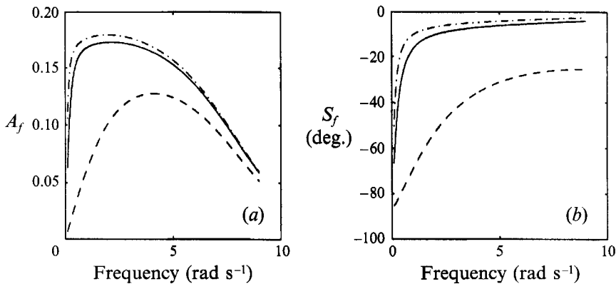
FIGURE 5. (a) Amplification factor and (b) phase lag. h_1 = 0.30 m, h_2 = 0.09 m; \nu_m ( \text{m}^2 \text{s}^{-1} ) = \cdots , 5 \times 10^{-4} ; \text{—} , 10^{-3} ; \text{-- --} , 10^{-2} ; \rho_m = 1230 \text{ Kg m}^{-3} .
