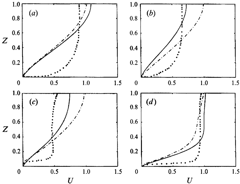
FIGURE 2. Drift velocity profile in the mud layer: \bullet , measured (Sakakiyama & Bijker); -\cdots , calculated (Sakakiyama & Bijker); - , calculated (Piedra-Cueva, present model). (a) Run A3, u_o = 4.9 \times 10^{-4} \text{ m s}^{-1} , at x = 3.5 \text{ m} ; (b) Run B1, u_o = 5.7 \times 10^{-4} \text{ m s}^{-1} , at x = 5.0 \text{ m} ; (c) Run C2, u_o = 1.1 \times 10^{-3} \text{ m s}^{-1} , at x = 6.0 \text{ m} ; (d) Run D3, u_o = 1.11 \times 10^{-3} \text{ m s}^{-1} , at x = 6.0 \text{ m} .
