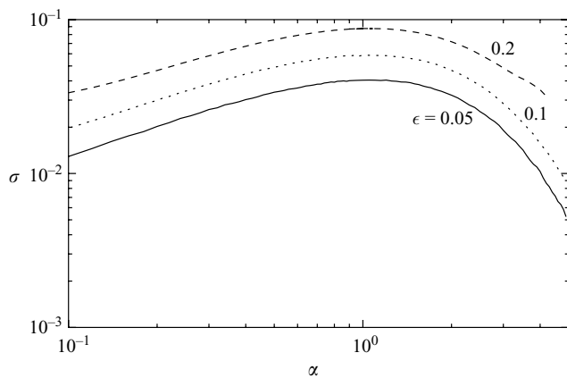
FIGURE 15. Trace of the growth rate \sigma = \epsilon \sigma_1 at the preferred wavenumber l_s for various wave slopes: \epsilon = 0.05, 0.1, 0.2 for \beta = 0.5 and z_a = -1 .
