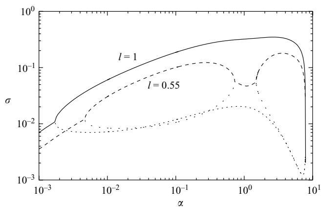
FIGURE 7. Growth rate \sigma = \epsilon \sigma_1 against \alpha for \epsilon = 0.1 and \beta = 0.5 when l = 0.55 and l = 1 with z_a = -1 .
