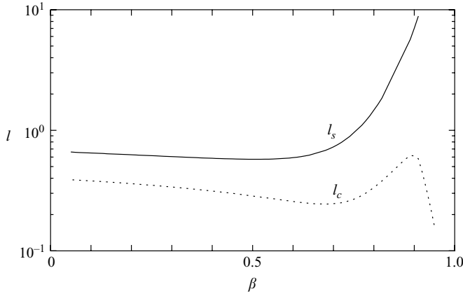
FIGURE 4. Trace of the preferred wavenumbers l_s and l_c against \beta for \epsilon = 0.1 , \alpha = 1 and z_a = -1 .
