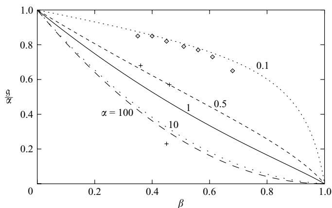
FIGURE 17. Plot of g/\alpha against \beta for various values of \alpha . + Data of Melville et al. (1998); \diamond data of Veron & Melville (2001).
