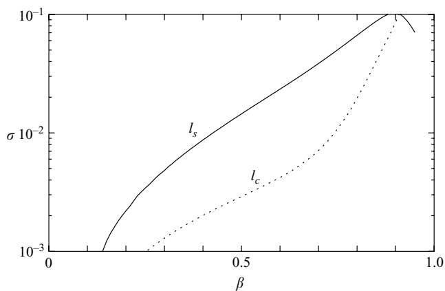
FIGURE 5. Growth rate \sigma = \epsilon \sigma_1 at the preferred wavenumbers l_s and l_c against \beta for \epsilon = 0.1 , \alpha = 1 and z_a = -1 .
