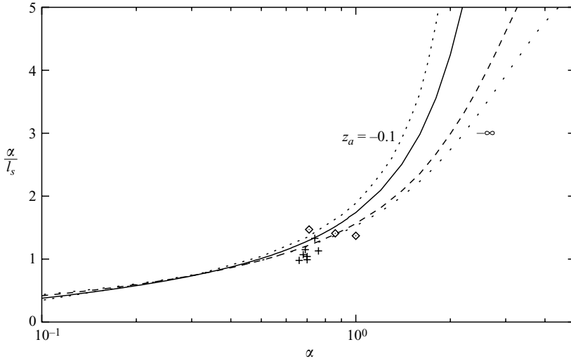
FIGURE 12. Streamwise wavenumber \alpha normalized by the preferred wavenumber l_s as a function of \alpha at various depths: z_a = -0.1, -1, -10 and z \rightarrow -\infty for \beta = 0.5 and \epsilon = 0.1 . \diamond , Data of Melville et al. (1998); +, data of Veron & Melville (2001).
