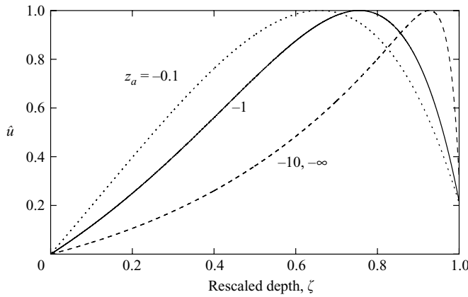
FIGURE 9. Perturbation eigenfunctions \hat{u} at l_s with \epsilon = 0.1 , \alpha = 1 and \beta = 0.5 for various depths -z_a = 0.1, 1, 10, \infty .
