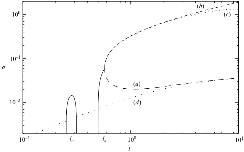
FIGURE 3. Comparison of the real part of the maximum growth rate \sigma = \epsilon\sigma_1 as a function of l for \epsilon=0.1 , \alpha=1 , \beta=0.5 and z_a=-1 : (a-c) with a free surface; (a) with (3.14) asymptotic to the distinguished limit (3.15); (b) with (3.14) asymptotic to the distinguished limit (3.16); (c) with (3.14) asymptotic to the regularized distinguished limit (3.17); (d) with rigid boundaries (from Phillips & Wu 1994).
