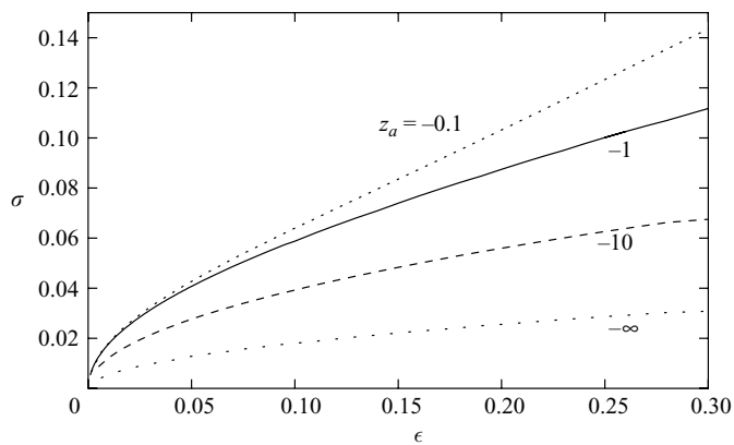
FIGURE 16. Variation in the growth rate \sigma = \epsilon \sigma_1 at l_s against wave slope for \alpha = 1, \beta = 0.5 at various depths, -z_a = 0.1, 1, 10, \infty .
