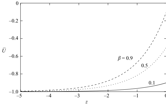
FIGURE 1. Eulerian mean velocity \bar{U} as a function of depth z for \beta = 0.1, 0.5, 0.9 and h = 1 . Curves for negative \beta are obtained by adding 2 to their positive- \beta counterparts.
