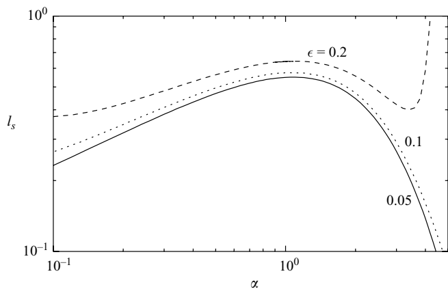
FIGURE 14. Trace of the preferred wavenumber l_s against \alpha for various wave slopes: \epsilon = 0.05, 0.1, 0.2 for \beta = 0.5 and z_a = -1 .
