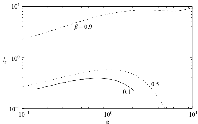
FIGURE 6. Trace of the preferred wavenumbers l_s of the instability as a function of \alpha for \epsilon = 0.1 and \beta = 0.1, 0.5, 0.9 for z_a = -1 .
