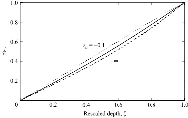
FIGURE 10. Perturbation eigenfunctions \hat{\phi} at l_s with \epsilon = 0.1 , \alpha = 1 and \beta = 0.5 for various depths -z_a = 0.1, 1, 10, \infty .
