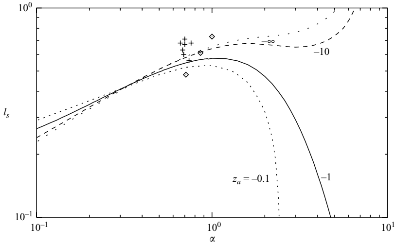
FIGURE 11. Trace of the preferred wavenumber l_s against \alpha at various depths: -z_a = 0.1, 1, 10, \infty for \beta = 0.5 and \epsilon = 0.1 . \diamond , Data of Melville et al. (1998); + , data of Veron & Melville (2001).
