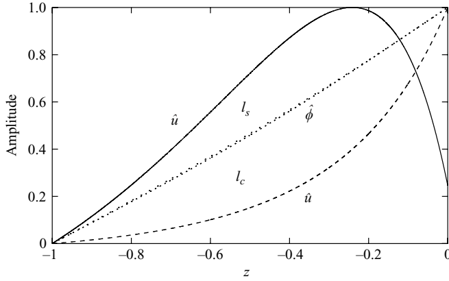
FIGURE 8. Perturbation eigenfunctions \hat{u} and \hat{\phi} at l_c = 0.28 and l_s = 0.57 with \epsilon = 0.1 , \alpha = 1 , \beta = 0.5 and z_a = -1 .
