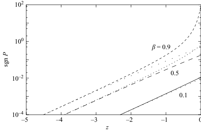
FIGURE 2. Primary pseudomomentum P as a function of depth z for \alpha=1 and \pm\beta = 0.1, 0.5, 0.9 with h=1 . In each instance the lower curve is for negative \beta . Note that the sign of P is determined by the sign of -\bar{U} .
