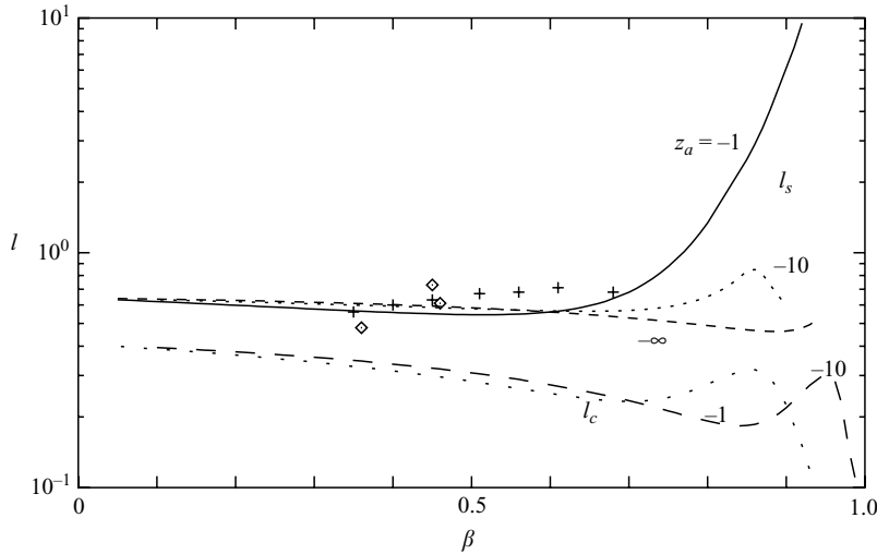
FIGURE 13. Trace of the preferred wavenumbers l_s and l_c of the instability as a function of \beta for \epsilon = 0.1 and \alpha = 0.7 for depths -z_a = 1, 10, \infty . \diamond , Data of Melville et al. (1998); +, data of Veron & Melville (2001).
