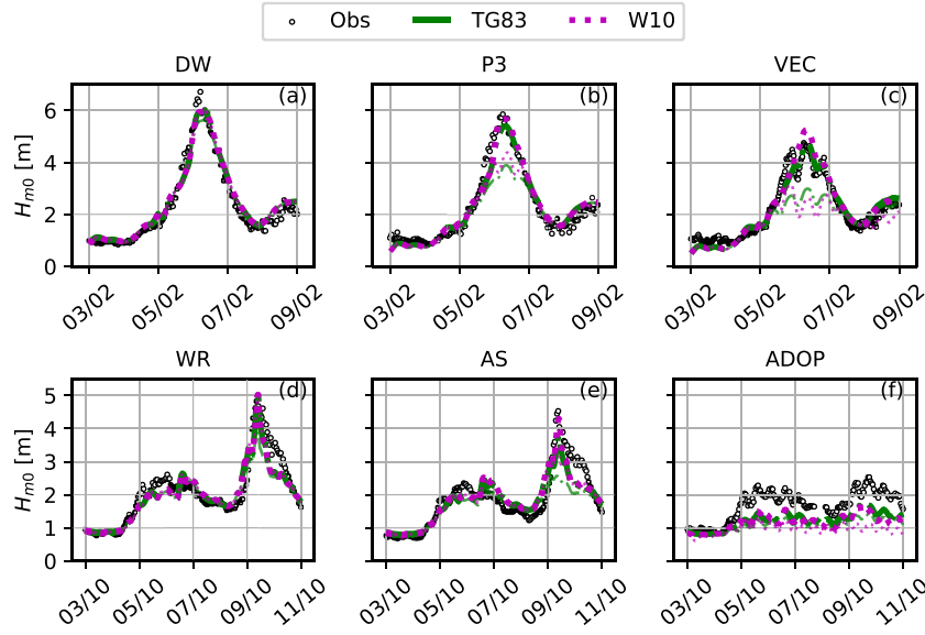
Fig. 7. Measured and simulated H_{m0} for the two study cases using TG83 and W10 formulations with the adaptive parameterization of the breaking coefficient. The thin light curves correspond to the results obtained with the default parameterizations.
