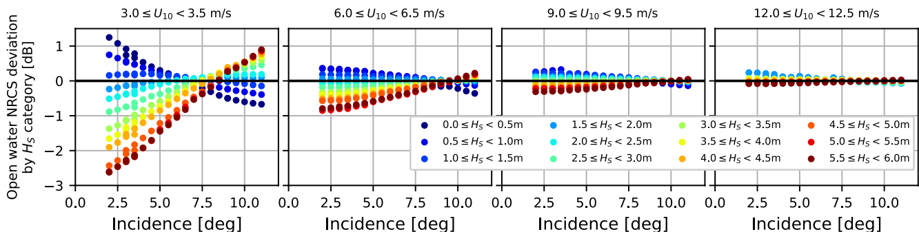
Figure 5. Distribution of Normalized Radar Cross-Section (NRCS) deviation from Equation 26 by H_s category over open water as a function of incidence angle for all off-nadir beams for four different wind speeds.
