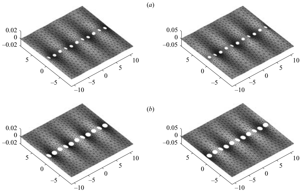
FIGURE 5. Rayleigh-Bloch wave excited in a semi-infinite array of cylinders with radius a_1 = 1/2 (left) and a_2 = 3/4 (right): (a) real part; (b) imaginary part.
