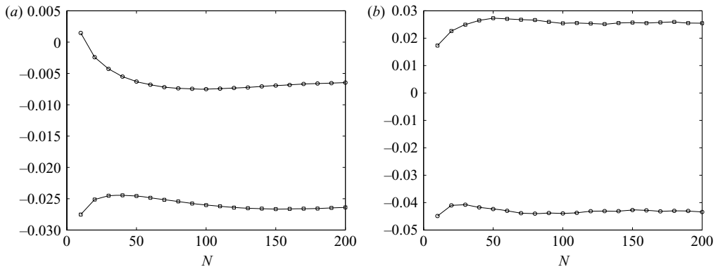
FIGURE 3. Real ( \square ) and imaginary ( \circ ) parts of c for an increasing number of cylinders, calculated using the projection method, for a_1 = 1/2 (a) and a_2 = 3/4 (b).
