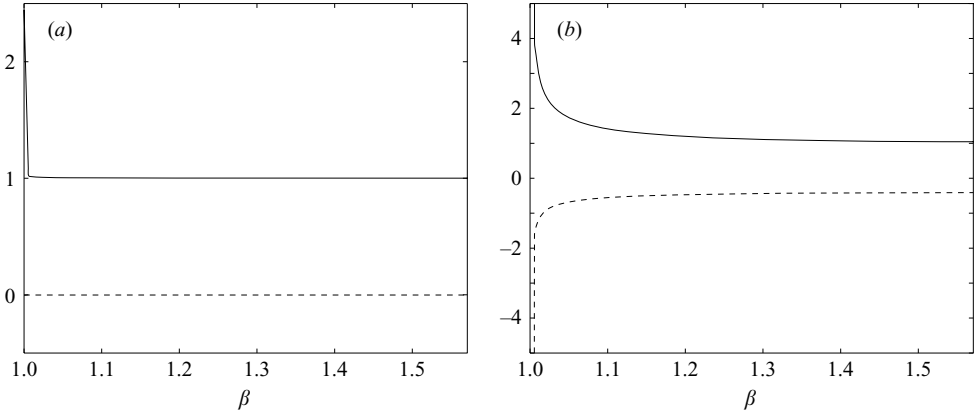
FIGURE 7. Real part (solid line) and imaginary part (dashed line) of the determinant of (\mathbf{I} - \mathbf{B}^t \mathbf{S}^{inf}(\beta)) plotted against \beta for a circular stiff plate with non-dimensional mass \tilde{\gamma} = 0 (a) and \tilde{\gamma} \rightarrow \infty (b).
