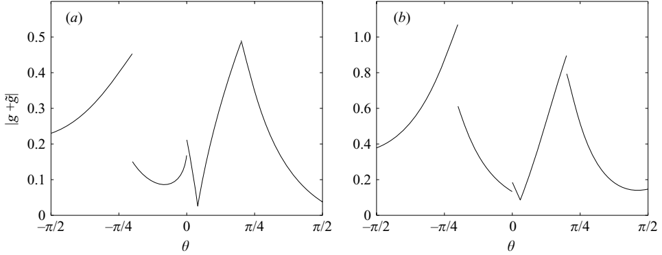
FIGURE 6. Absolute value of the amplitude of the circular wave, |g(\theta) + \tilde{g}(r, \theta)| , for r = 2\pi and a_1 = 1/2 (a) and a_2 = 3/4 (b).
