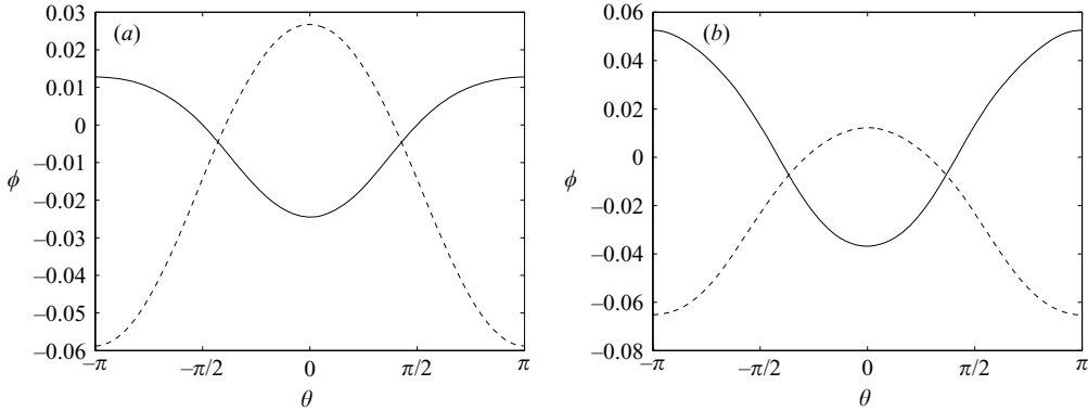
FIGURE 2. Real part (solid line) and imaginary part (dashed line) of the potential of the Rayleigh–Bloch wave associated with the zeroth cylinder at the cylinder boundary, \phi_0^{RB}(a_k, \theta) for a_1 = 1/2 (a) and a_2 = 3/4 (b), also see (8.2).
