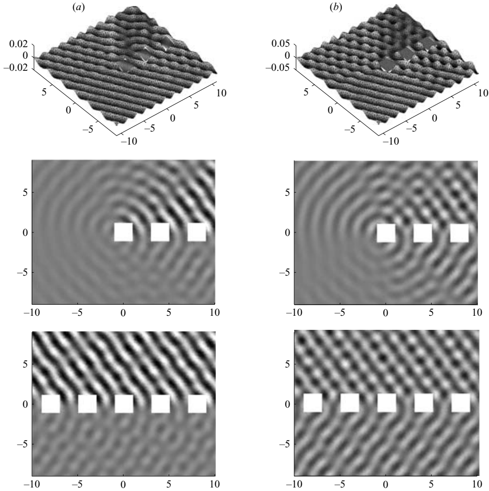
FIGURE 8. Solution to the scattering problem for an array of floating elastic plates with non-dimensional stiffness and mass \tilde{\beta} = \tilde{\gamma} = 0.02 (a) and a similar array of fixed docks (b). Top, total wave field; middle, scattered wave field; bottom, scattered wave field of the corresponding infinite array.
