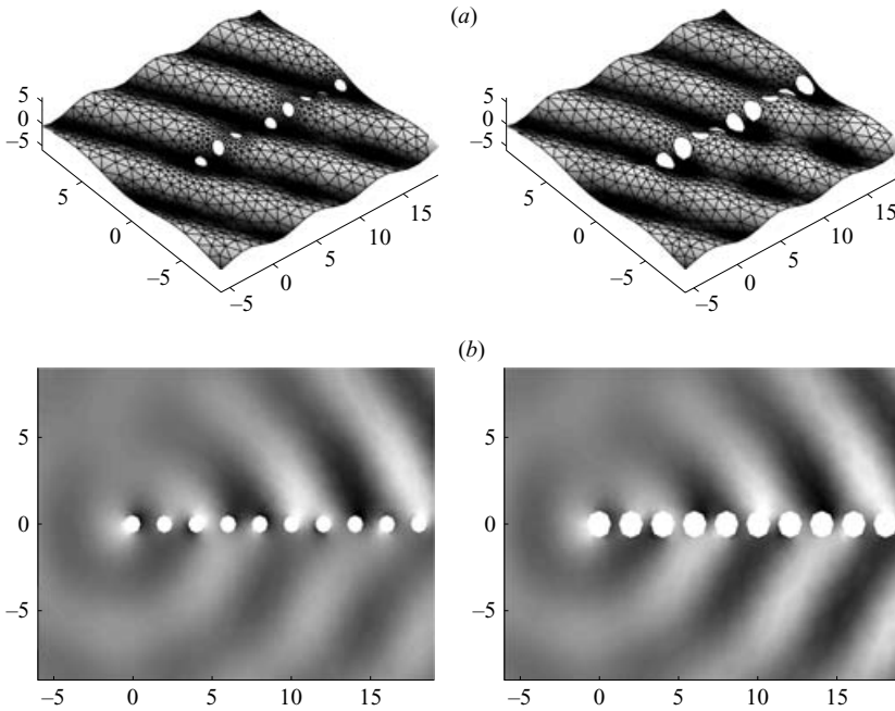
FIGURE 4. Total wave field (a) and scattered wave field only (b) from the solution for the semi-infinite array of cylinders with radius a_1 = 1/2 (left) or a_2 = 3/4 (right).
