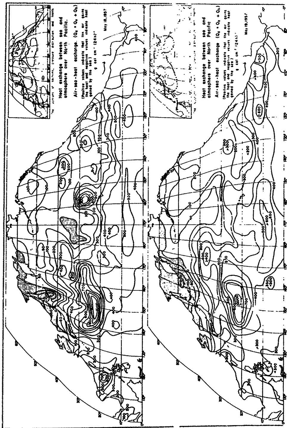
Figure 14. Air-Sea Heat Exchange ( \text{g cal/cm}^2/\text{day} ) Over the North Pacific For 18-19 May 1957 (After Laevastu).
