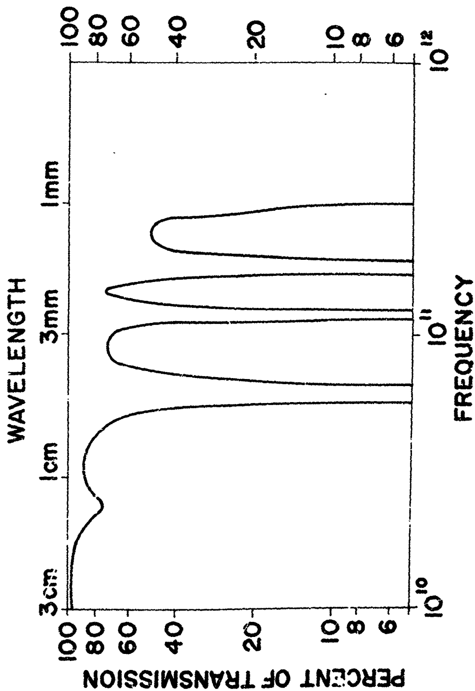
Figure 1b. Total Atmospheric Transmission.
