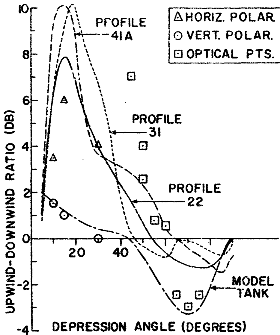
Figure 9 Comparison of Upwind-Downwind Ratios
