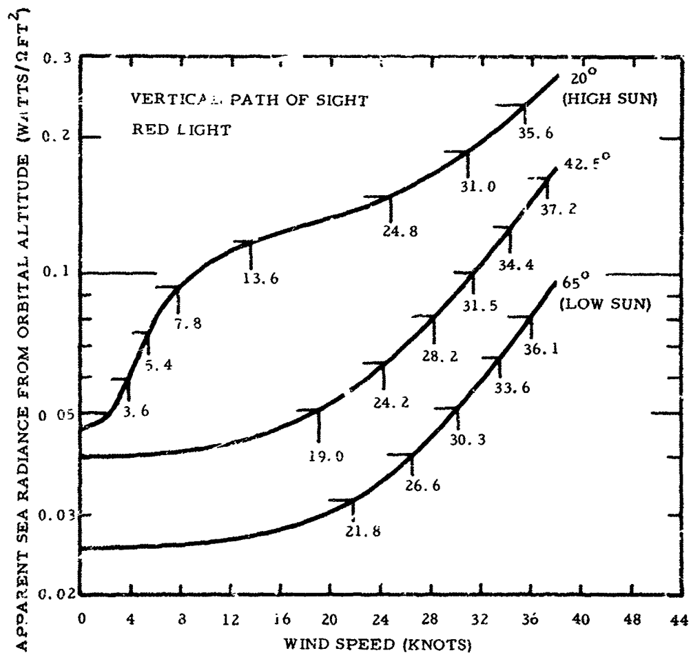
Figure 1. Apparent Sea Radiance From Orbital Altitude (Watts/Ω Ft 2 )
