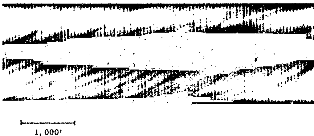
Figure 7. Pattern With Sewage Contamination of the Ocean Surface.
