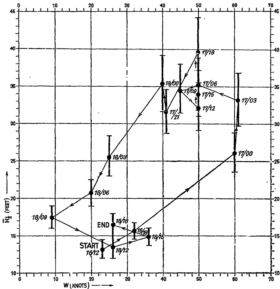
Fig. 4. Graph of significant wave heights (with upper 95% and lower 5% confidence limits) versus wind speed with time as the parameter
