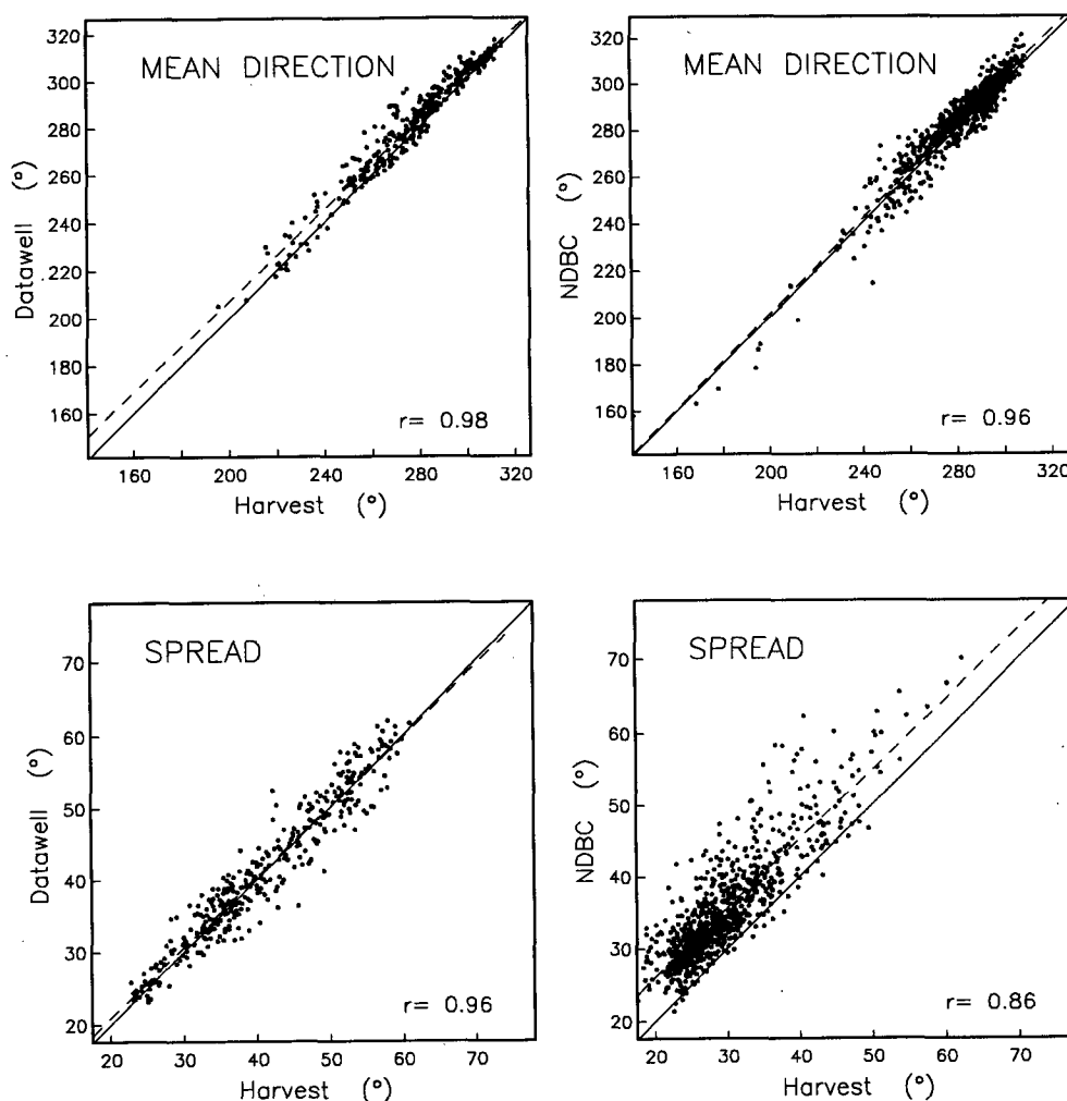
FIG. 6. Comparison of mean direction and spread estimates from the Harvest Platform array with the Datawell Directional Waverider buoy (left panels) and the NDBC 3-m discus buoy (right panels). See Fig. 5 caption.
