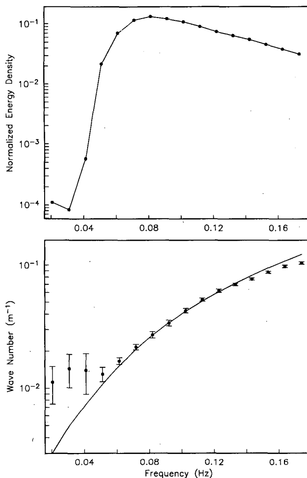
FIG. 4. Average spectral shape and wave numbers observed at Harvest Platform during May 1993. Upper panel: average of surface elevation spectra (each normalized by the total variance in the range 0.02–0.20 Hz). Lower panel: observed root-mean-square wavenumber [dots, Eq. (6)] vs frequency. Bars indicate plus/minus one standard deviation based on 198 data runs. The solid curve is the theoretical linear dispersion relation.
