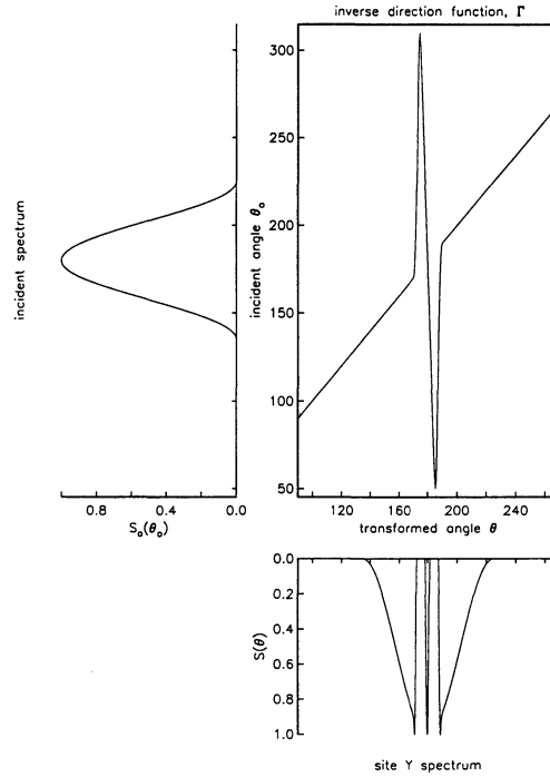
FIG. 2. Spectral Transformation of Arbitrarily Selected Incident ( f = 0.06 Hz) Wave Directional Spectrum (Upper-Left Panel) to Location Y (Lower-Right Panel); kC_{go}/k_oC_g = 1 . Units of Spectra are Arbitrary and Upper-Right Panel is Inverse Direction Function for Location Y in Fig. 1(c)
