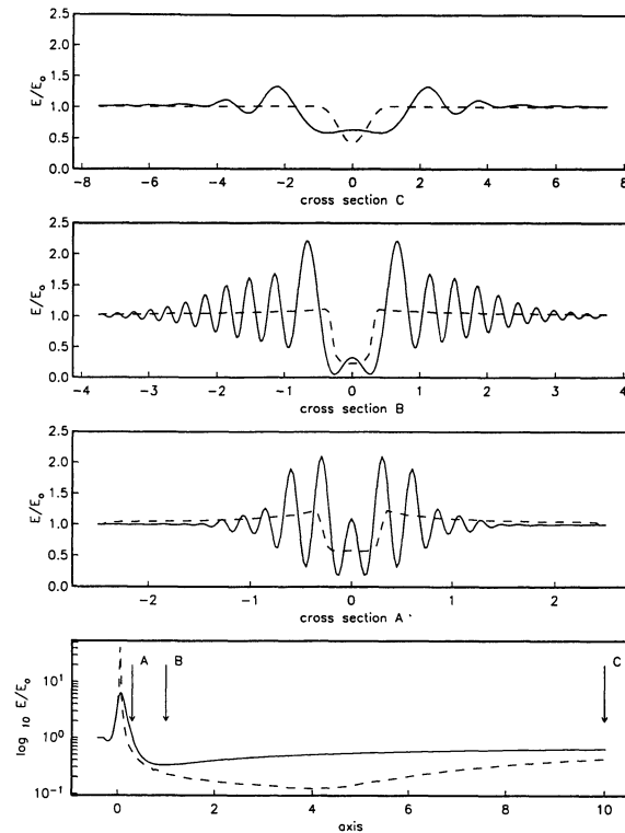
FIG. 6. Normalized, Directionally Integrated Wave Energy for Circular Shoal (Transect Locations Shown in Fig. 4). Narrow Directional Case, FWHM = 5^\circ , Wave Frequency f = 0.06 Hz. Solid and Dashed Lines are RD and R Models, Respectively. Distances in km
