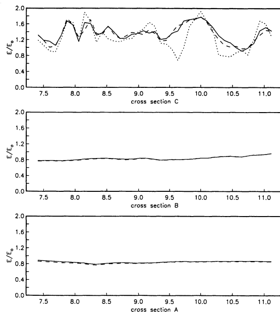
FIG. 10. Normalized, Directionally Integrated Wave Energy for Mission Beach, California. Broad Directional Case, FWHM = 45°. Same Format as Fig. 9
