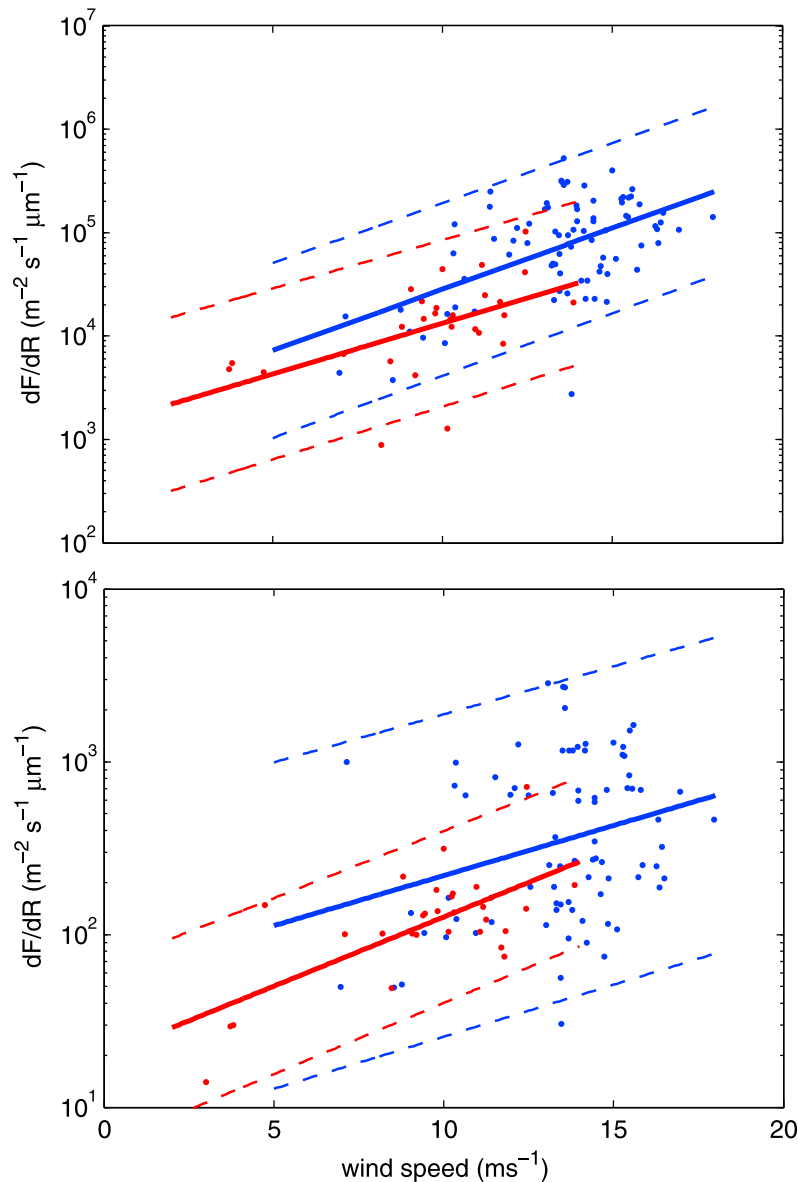
Figure 11. The effect of mean wave state on the particle flux variation with local 10 m wind speed for two contrasting particle sizes: (top) R_{80} = 0.9 \mu\text{m} ( 0.41\text{--}1.4 \mu\text{m} ) and (bottom) R_{80} = 3.9 \mu\text{m} ( 3.6\text{--}4.2 \mu\text{m} ). A mean wave slope of greater than 0.03 (blue) represents undeveloped seas; a value less than 0.03 (red) represents fully developed seas. The solid lines are the best fits (equation (2)), while the dashed lines represent the 95% confidence bounds on the fit.
