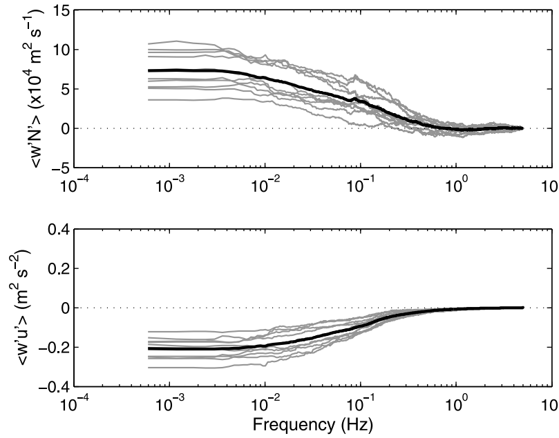
Figure 3. Ogive curves for nine consecutive 28 min records of (top) aerosol flux for particles with mean radius at R_{\text{amb}} = 0.35 \mu\text{m} (channel range of 0.29\text{--}0.41 \mu\text{m} ) and (bottom) the corresponding momentum fluxes at a mean wind speed of 11 \text{ m s}^{-1} on 24 March. The gray lines are the individual records; the black lines are the mean of all nine ogives in each case.
