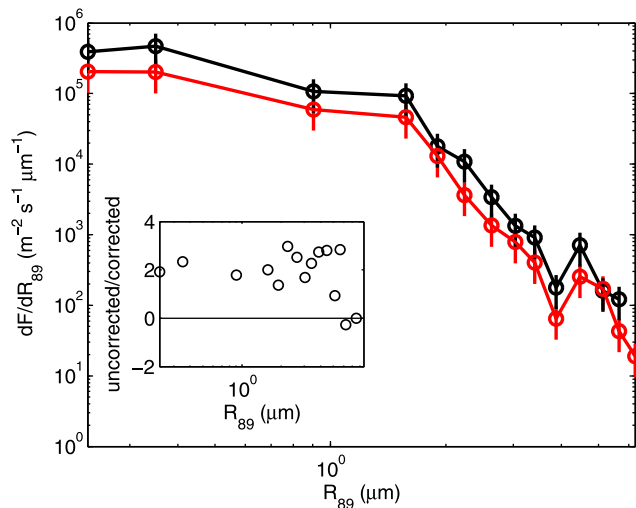
Figure 4. A single estimate of the particle flux spectrum corrected for the humidity flux induced bias (red line) and the uncorrected flux spectra (black line). The relative humidity for this record varied from 83% to 95%, with a mean of 89%; the water vapor flux was 0.012 \text{ g kg}^{-1} . The error bars show the median standard error for the entire data set (30%). The inset shows raw uncorrected flux spectrum divided by the correct flux spectrum.
