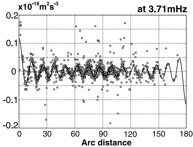
Figure 1. Plot of the real part of the stacked cross-spectral density as a function of station separation distance at a fixed frequency of 3.71 mHz. The Legendre function with angular order of 29 is superposed as a reference.
