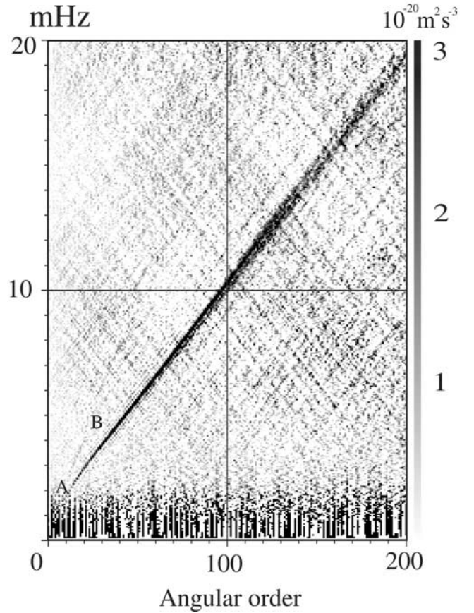
Figure 2. Wavenumber-frequency spectral representation of the ground noise. The wavenumber is given by the angular order l , which corresponds to the wavelength 2\pi R/(l + 1/2) , where R is the radius of the Earth. This illustration shows strong energy concentration along the fundamental mode branch up to angular order 200 and weak energy concentration along the first overtone branch (from points A to B). Stripes along the fundamental dispersion branch and those in mirror symmetry are due to spatial alias of the energy of fundamental Rayleigh waves.
