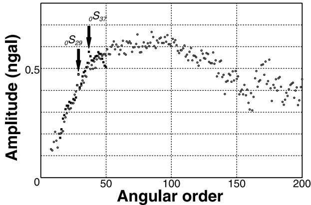
Figure 4. Rms amplitudes of the fundamental spheroidal modes (fundamental Rayleigh waves). Open circles show the modal amplitudes obtained in the present study. Closed squares in the lower frequency range indicate the modal amplitudes obtained through the normal mode approach [Nishida et al. , 2000]. The modes denoted as 0S_{29} and 0S_{37} are theoretically expected to be coupled with acoustic free oscillations in the atmosphere.
