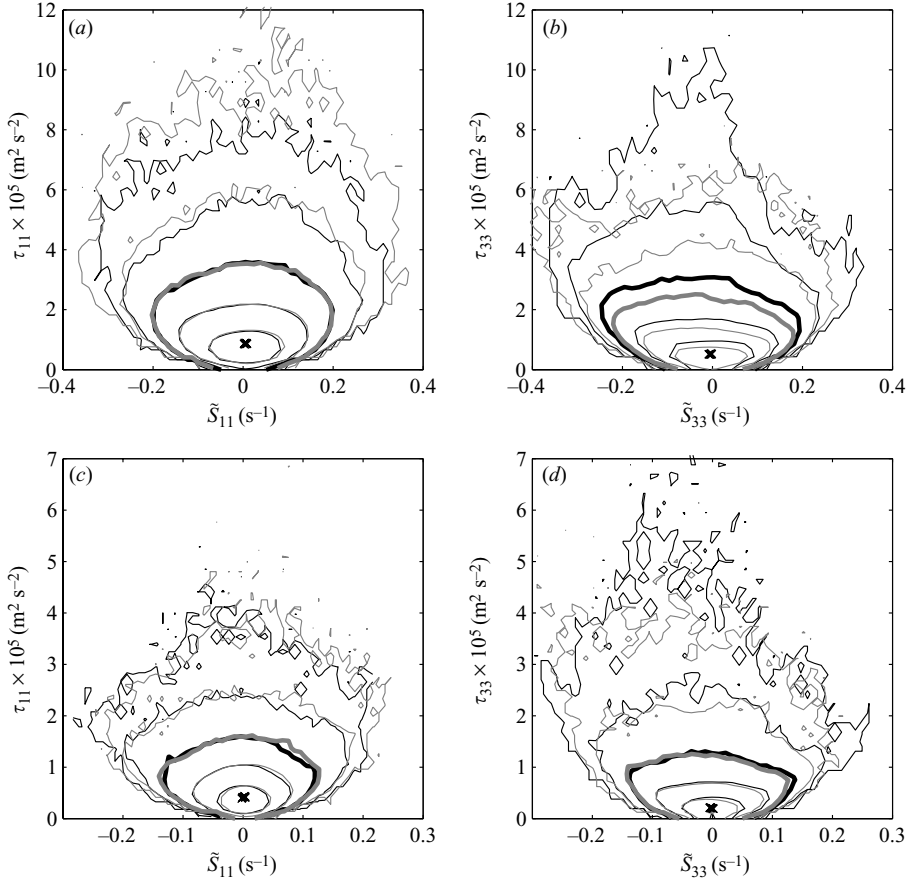
FIGURE 12. Joint PDFs of \tau_{ii} and \tilde{S}_{ii} conditionally sampled on wave phase for \Delta/\delta=8 . (a, b) run C, (c, d) run E. Black contours are for -135^\circ < \Phi'' < -45^\circ , grey contours are for 45^\circ < \Phi'' < 135^\circ . Contours are at 10^{-6}, 10^{-5}, \dots, 10^{-1} with the level at 10^{-4} emphasized. The crosses indicate the variation of the conditionally sampled mean values.
