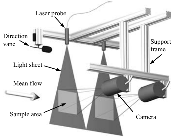
FIGURE 1. A three-dimensional schematic of the submerged components of the PIV system. The scale of the sample areas is given in table 1.
