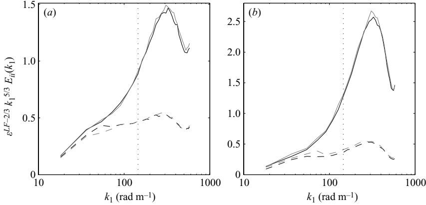
FIGURE 13. Compensated spectra ( \varepsilon^{LF-2/3} k_1^{5/3} E_{ii}(k_1) ) for (a) run C and (b) run E. Solid lines: E_{11}(k_1) ; dashed lines: E_{33}(k_1) . Black lines: -135^\circ < \Phi'' < -45^\circ , grey lines: 45^\circ < \Phi'' < 135^\circ . \varepsilon^{LF} is the spectral line-fit estimate of the dissipation taken from NS05: run C, \varepsilon^{LF} = 7.65 \times 10^{-7} \text{ m}^2 \text{ s}^{-3} ; run E, \varepsilon^{LF} = 1.92 \times 10^{-7} \text{ m}^2 \text{ s}^{-3} . The vertical dotted line indicates the scale of \Delta/\delta = 8 .
