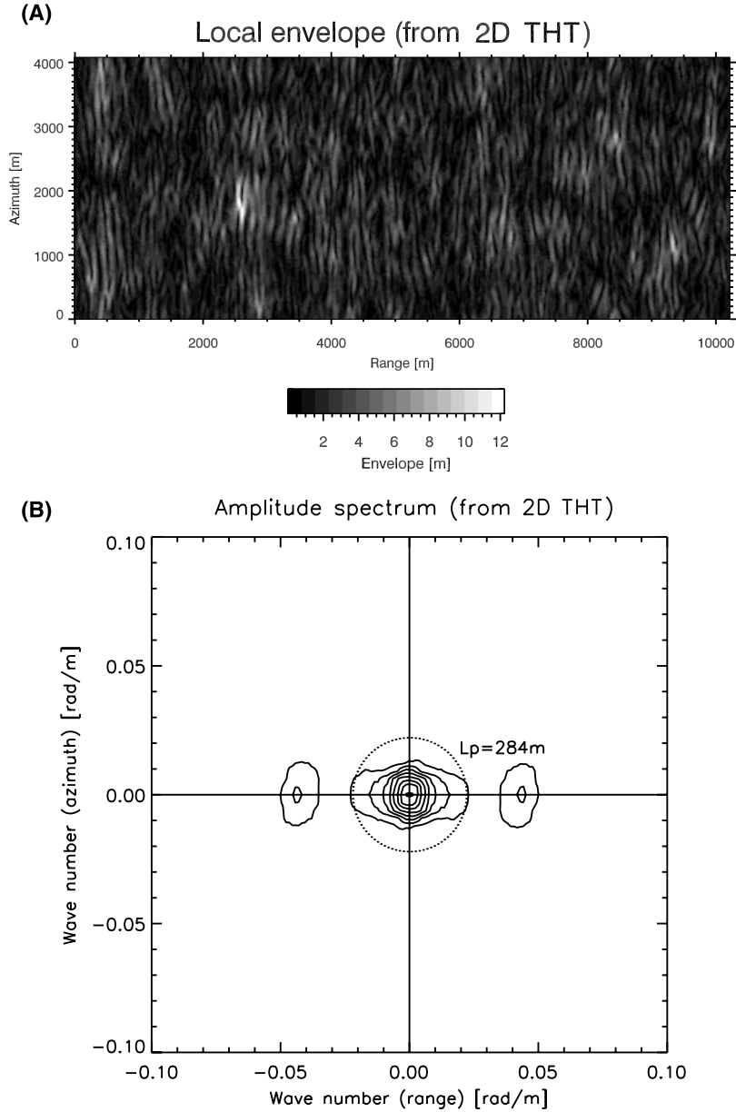
Figure 6. (a) Two-dimensional envelope \rho_I(\mathbf{r}) (see Equation 14) derived from the two-dimensional THT of the wave elevation map shown in Figure 3. (b) Corresponding spectral density of \rho_I(\mathbf{r}) . The dotted line indicates the circle k = k_p = 2\pi/L_p .
