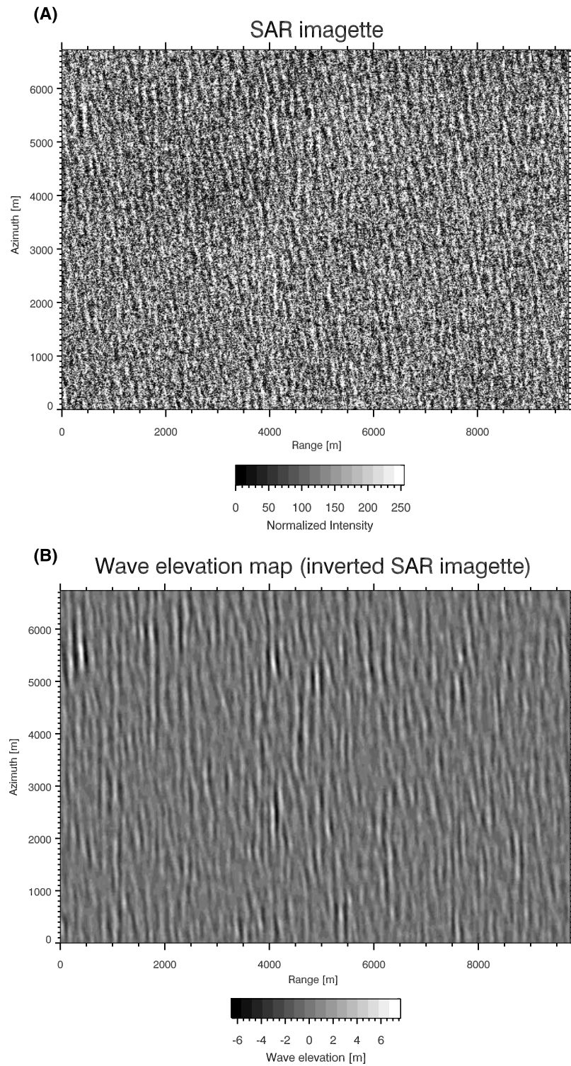
Figure 9. (a) Normalized intensity image and (b) its corresponding wave elevation map derived from the LISE method. The measurement was taken by the ENVISAT ASAR in wave mode on 9 July 2002 at 1925:17 UTC. The image location is 42.71^{\circ}\text{N} and 136.96^{\circ}\text{W} .
