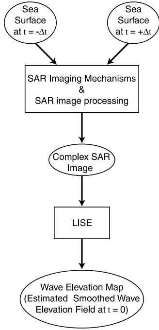
Figure 2. Scheme illustrating the application of the LISE method.
