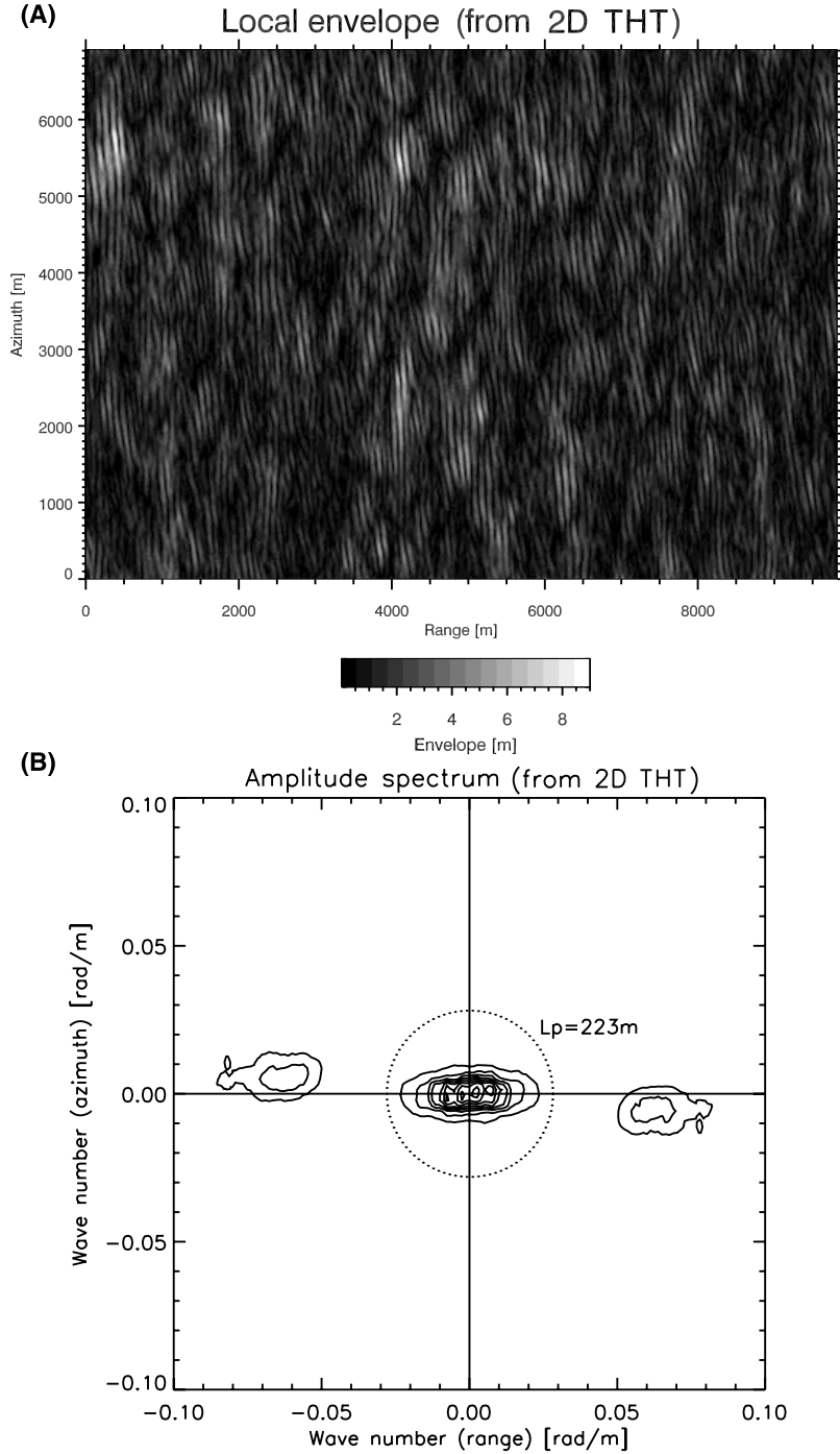
Figure 12. (a) Two-dimensional envelope \rho_A(\mathbf{r}) (see equation (14)) derived from the THT of the wave elevation map showed in Figure 9. (b) Corresponding spectral density of \rho_A(\mathbf{r}) . The dotted line indicates the circle k = k_p = 2\pi/L_p .
