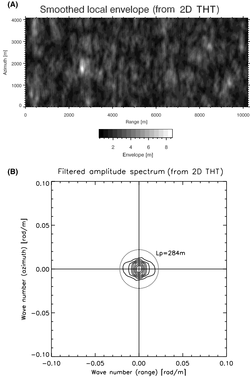
Figure 7. (a) Smoothed envelope \tilde{\rho}_f(\mathbf{r}) . (b) Corresponding spectral density \tilde{\rho}_f(\mathbf{r}) . The dotted line indicates the circle k = k_p = 2\pi/L_p .
