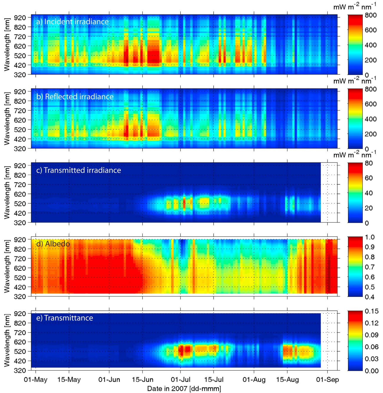
Figure 6. Time series of (a) incoming, (b) reflected, and (c) transmitted spectral irradiance as well as spectral (d) albedo and (e) transmittance. One spectrum is shown per day, from the observation with the highest solar elevation angle. As the under-ice sensor had to be retrieved on 28 August, no transmitted irradiance or transmittance data are available afterward. Blanked (white) areas in the albedo and transmittance data result from the reduction in wavelength range due to data quality issues.
