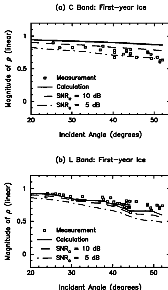
Figure 25. Effects of noise in correlation coefficient of first-year ice at (a) C band and (b) L band.
