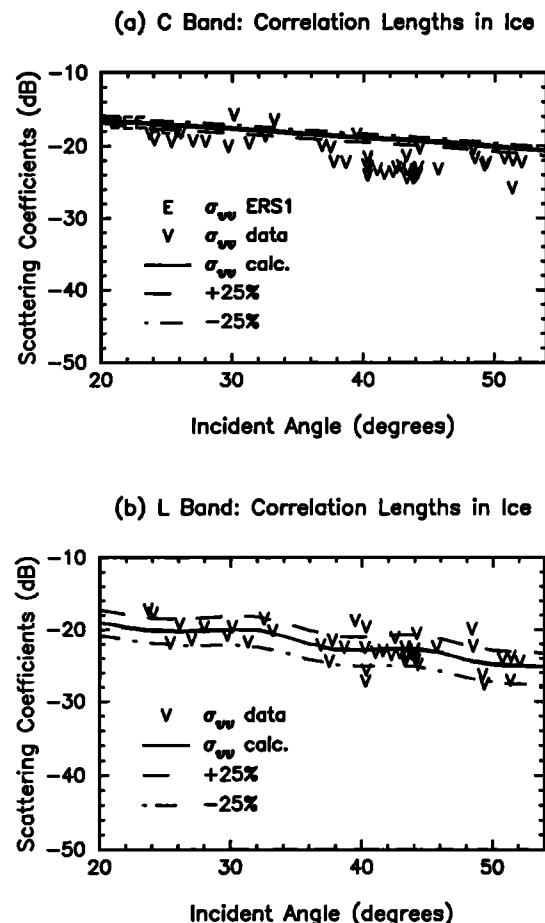
Figure 14. Variations in calculated backscattering coefficients due to \pm 25\% change in correlation lengths of brine inclusions for (a) C band and (b) L band.
