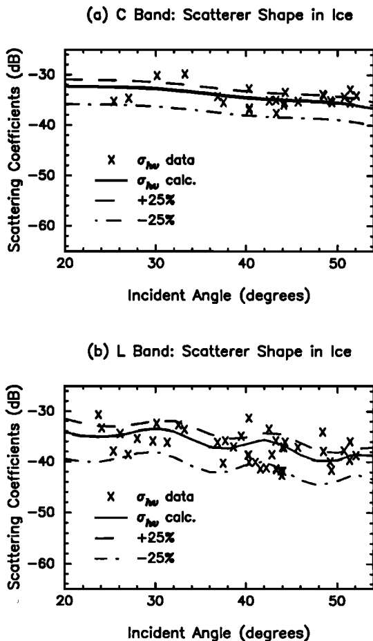
Figure 15. Variations in calculated backscattering coefficients due to \pm 25\% change in ratios of brine correlation lengths for (a) C band and (b) L band.
