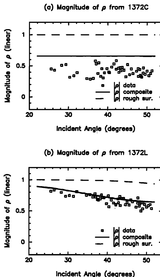
Figure 21. Comparisons of measured and calculated correlation coefficients for thin lead ice at (a) C band and (b) L band. Solid curves are calculated from the complete composite model. Dashed curves are for surface scattering without volume scattering.
