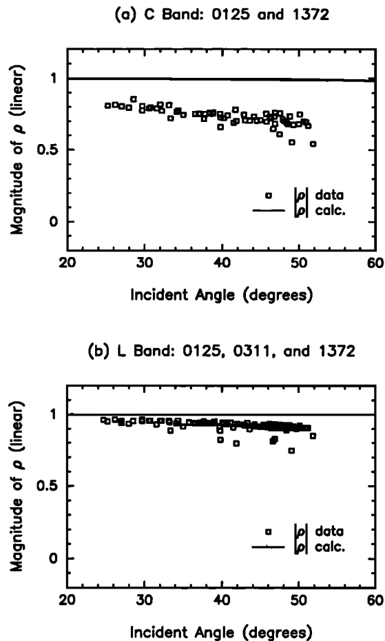
Figure 6. Comparisons of measured and calculated correlation coefficients for multiyear ice at (a) C band and (b) L band.
