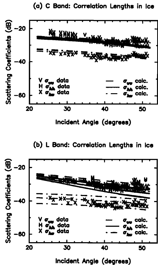
Figure 23. Variations in calculated coefficients due to \pm 25\% change in correlation lengths of brine inclusions for (a) C band and (b) L band. For each type of backscattering coefficient, the upper curve is for the increase in correlation lengths, the lower is for the decrease, and the middle is the same as in Figure 18 or 19 replotted as a reference.
