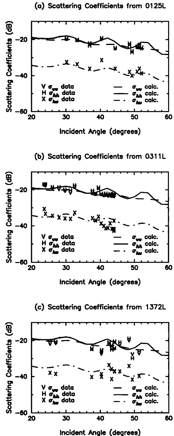
Figure 12. Comparisons of measured and calculated backscattering coefficients at L band for first-year ice in (a) scene 0125, (b) scene 0311, and (c) scene 1372.
