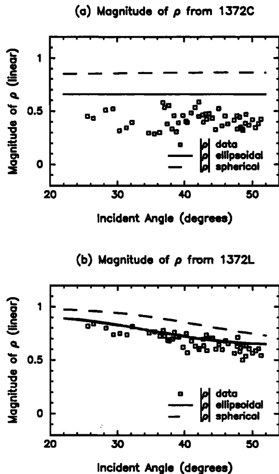
Figure 22. Comparisons of measured and calculated correlation coefficients for thin lead ice at (a) C band and (b) L band. Solid curves are calculated from the complete composite model with ellipsoidal brine inclusions. Dashed curves are for spherical brine inclusions.
