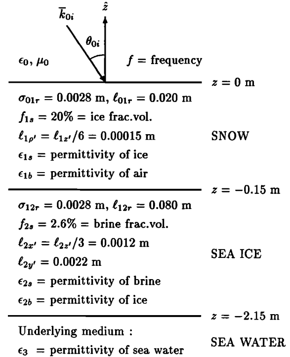
Figure 10. Physical parameters for first-year sea ice.
