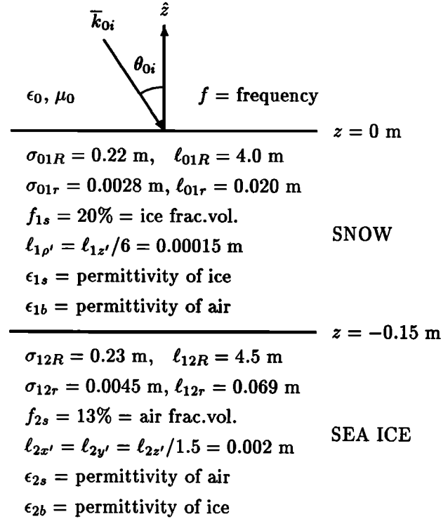
Figure 3. Physical parameters for multiyear sea ice.
