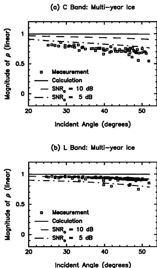
Figure 24. Effects of noise in correlation coefficient of multiyear ice at (a) C band and (b) L band.
