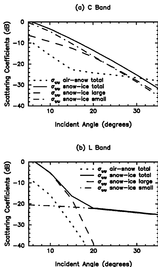
Figure 8. Composition of surface scattering at small incident angles for (a) C band and (b) L band. Dotted curves are total surface scattering from air-snow interface. For snow-ice interface, solid curves are for total surface scattering, dashed curves are scattering from large-scale roughness due to hummocks, and dash-dotted curves are scattering from small-scale roughness.
