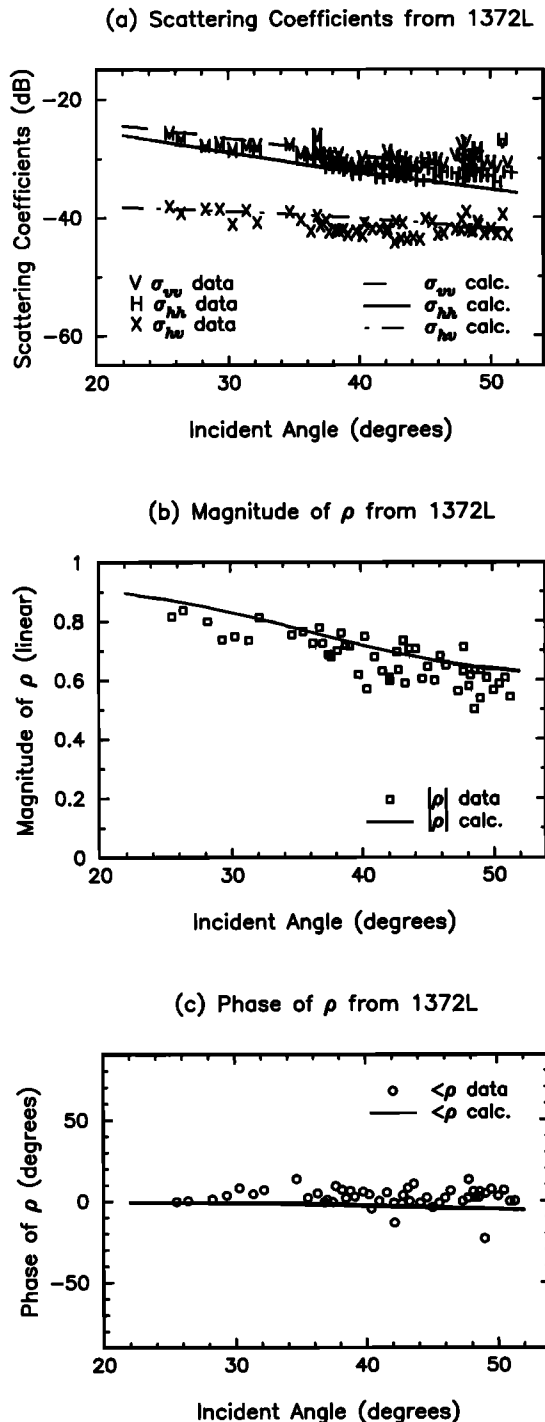
Figure 19. Comparisons of measured and calculated backscattering and correlation coefficients for thin lead ice at L band for (a) conventional backscattering coefficients, (b) magnitude of correlation coefficient, and (c) phase of correlation coefficient.
