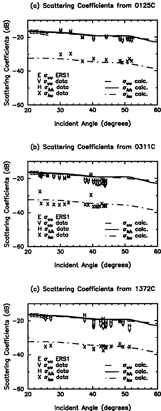
Figure 11. Comparisons of measured and calculated backscattering coefficients at C band for first-year ice in (a) scene 0125, (b) scene 0311, and (c) scene 1372.
