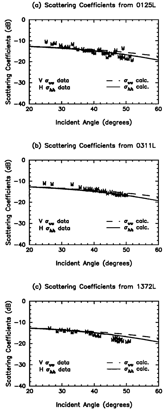
Figure 5. Comparisons of measured and calculated backscattering coefficients at L band for multiyear ice in (a) scene 0125, (b) scene 0311, and (c) scene 1372.
