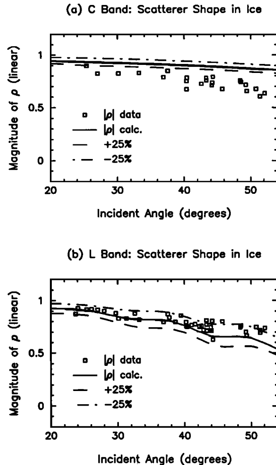
Figure 16. Variations in calculated correlation coefficients due to \pm 25\% change in ratios of brine correlation lengths for (a) C band and (b) L band.
