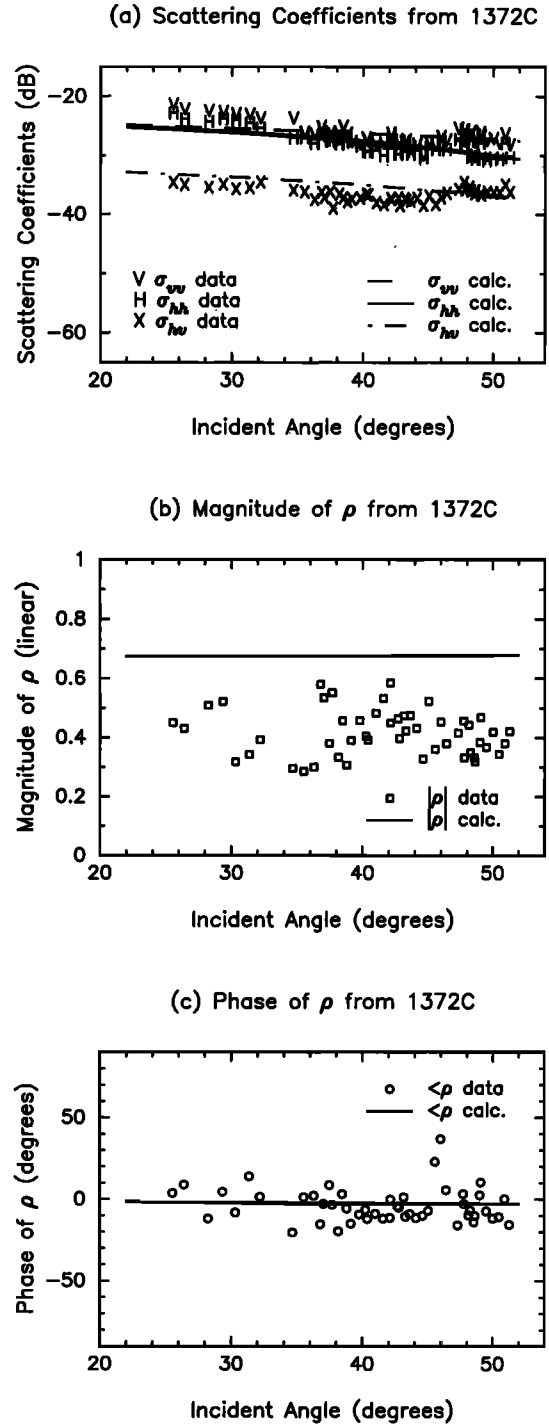
Figure 18. Comparisons of measured and calculated backscattering and correlation coefficients for thin lead ice at C band for (a) conventional backscattering coefficients, (b) magnitude of correlation coefficient, and (c) phase of correlation coefficient.
