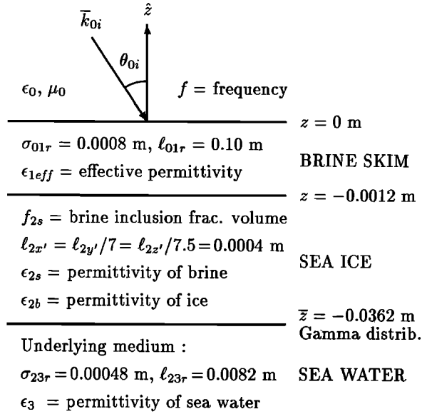
Figure 17. Physical parameters for thin lead ice.
