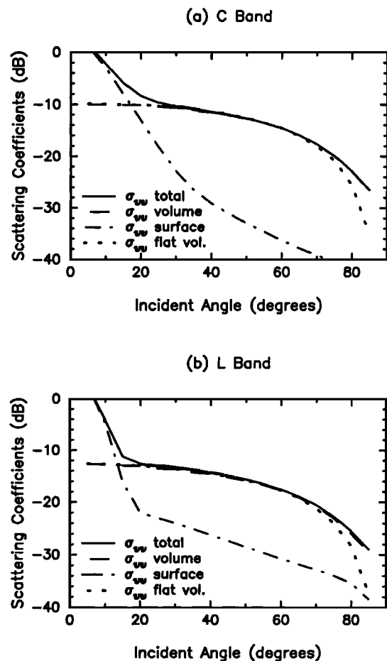
Figure 7. Composition of scattering from sea ice for (a) C band and (b) L band. Solid curves are total, dashed curves are volume scattering with effects of hummocks, dash-dotted curves are surface scattering with both small-scale roughness and large-scale hummocks, and dotted curves are volume scattering with flat interfaces.
