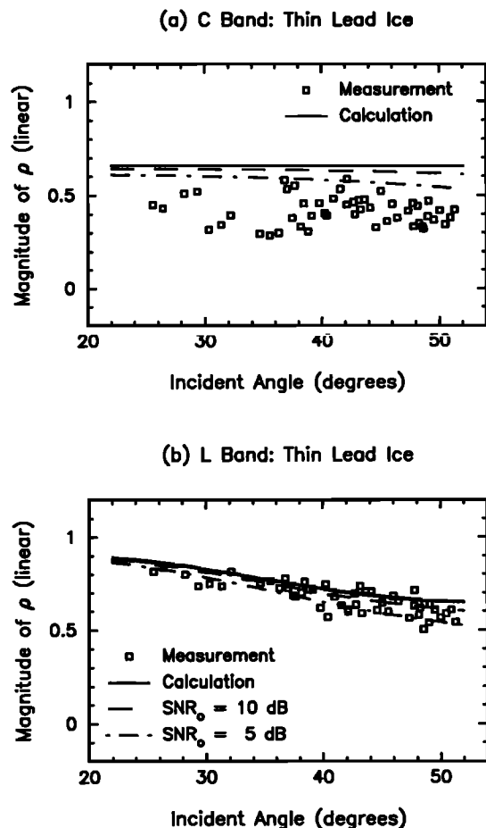
Figure 26. Effects of noise in correlation coefficient of thin lead ice at (a) C band and (b) L band.
