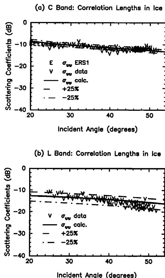
Figure 9. Variations in calculated backscattering coefficients due to \pm 25\% change in correlation lengths of air inclusions for (a) C band and (b) L band.
