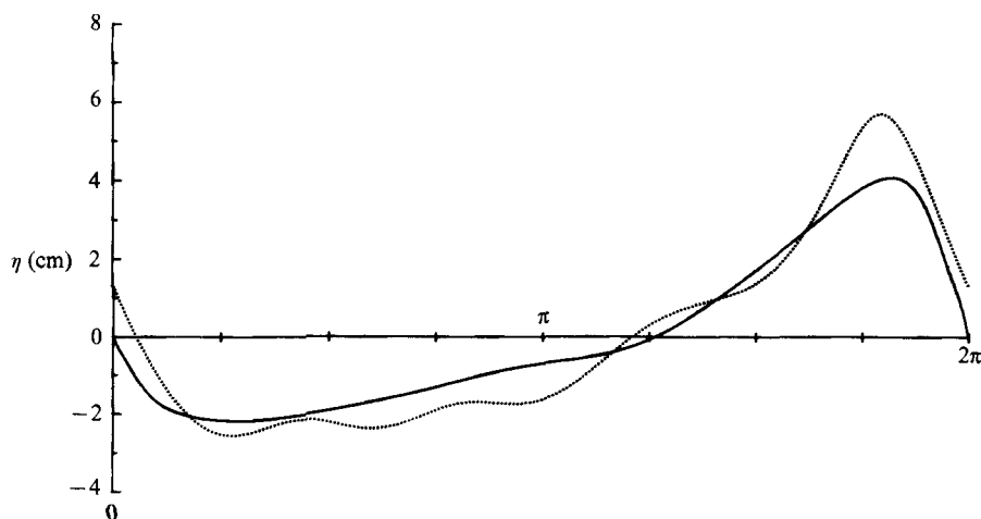
FIGURE 24. Inversely estimated wave profile consistent with ·····, the irrotational velocity field; and —, measured wave profile.
