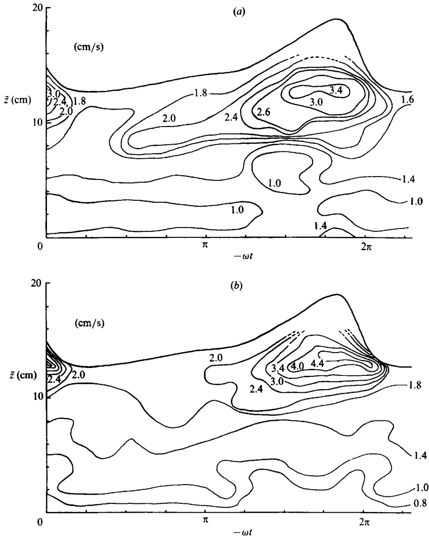
FIGURE 14. Distribution of horizontal and vertical components of turbulence intensity (a) u' and (b) w' , detected by a moving average method.
