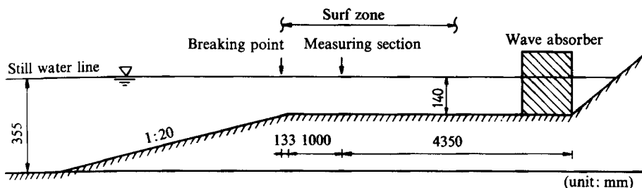
FIGURE 1. Experimental equipment.
