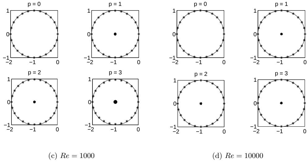
Figure 4-1: Eigenvalue footprints for element Jacobi preconditioned 1-D convection-diffusion
