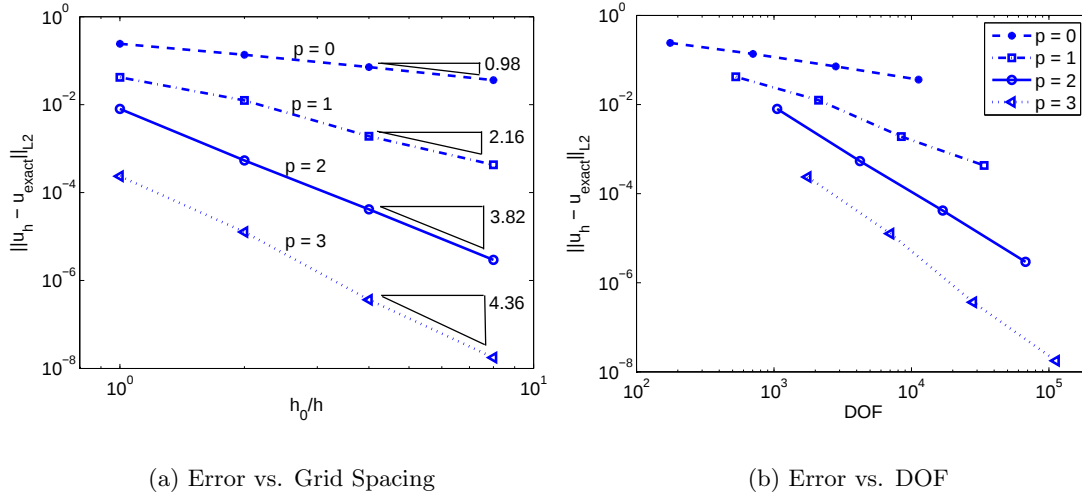
Figure 5-2: Accuracy results for 0 \leq p \leq 3 for Poiseuille flow test case
