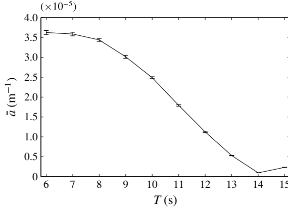
FIGURE 8. Wave energy attenuation coefficient \bar{a} as a function of wave period T in the range 6–15 s. The error bars represent the standard error of each estimated value of \bar{a} , and account for the goodness of the least-square fit and the variability in the ensemble of simulations.
