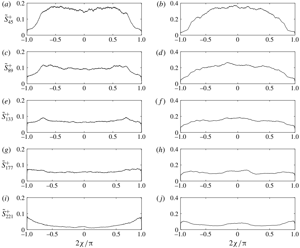
FIGURE 7. Ensemble average of the normalized forward energy density function \tilde{S}_q^+(\chi) for T=6 s (a,c,e,g,i) and 9 s (b,d,f,h,j). The energy densities are plotted for (a,b) q=45 (i.e. x \approx 10 km), (c,d) q=89 (i.e. x \approx 20 km), (e,f) q=133 (i.e. x \approx 30 km), (g,h) q=177 (i.e. x \approx 40 km) and (i,j) q=221 (i.e. x \approx 50 km).
