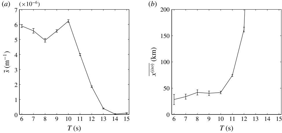
FIGURE 9. (a) Rate of directional spreading \bar{s} as a function of wave period T in the range 6–15 s. (b) Distance to isotropy \bar{x}^{(iso)} plotted over the same range of wave periods. Error bars are computed as in figure 8.
