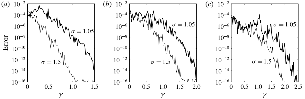
FIGURE 3. Estimated error on values of the reflection coefficient against the truncation parameter \gamma . The convergence analysis is conducted for (a) T=6 s, (b) 9 s and (c) 12 s, and two grating spacings.
