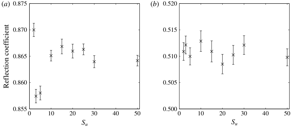
FIGURE 5. Ensemble average of the reflection coefficient by a 100-slab array computed for different values of S_u . The array in each unique slab is generated using the FSD described in § 5.2 with dimensions L_x = 220 m and L_y = 51L_x . Results are shown for (a) T = 6 s and (b) T = 9 s. Averages are computed from 50 random realizations of the array and wave forcing (with a cosine square spread).
