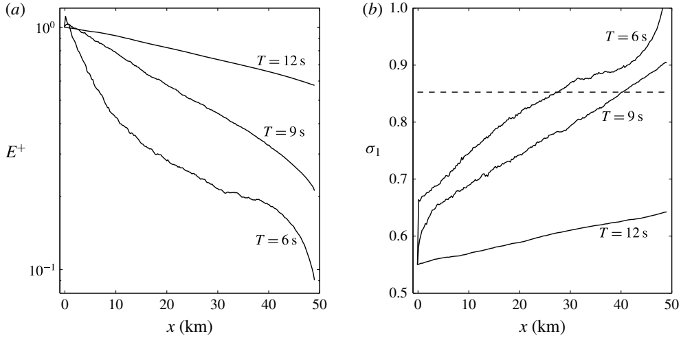
FIGURE 6. (a) Ensemble average of the forward propagating wave energy E^+ and (b) the directional spread \sigma_1 through \approx 50 km of simulated MIZ, for T = 6, 9 and 12 s. In (b) the dashed line corresponds to the theoretical value of \sigma_1 characterizing an isotropic directional wave field. This value is independent of the wave period.
