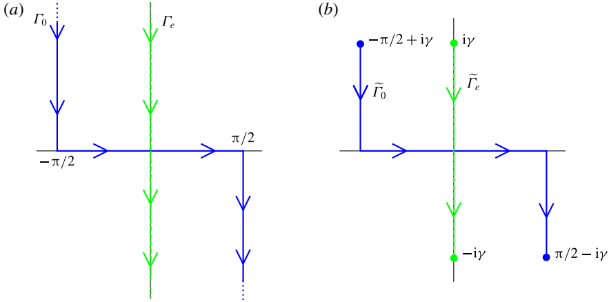
FIGURE 2. (Colour online) (a) The integration contours \Gamma_0 (blue solid) and \Gamma_e (green dashed) in the complex \chi -plane, which describe the domains of the amplitude functions A_{m;q}^{\pm}(\chi) for travelling ( m = 0 ) and evanescent ( m \geq 1 ) vertical modes respectively. The arrows indicate the directions of the contours. (b) The corresponding truncated contours \tilde{\Gamma}_0 (blue solid) and \tilde{\Gamma}_e (green dashed) used in the numerical approximation discussed in § 3.2.
