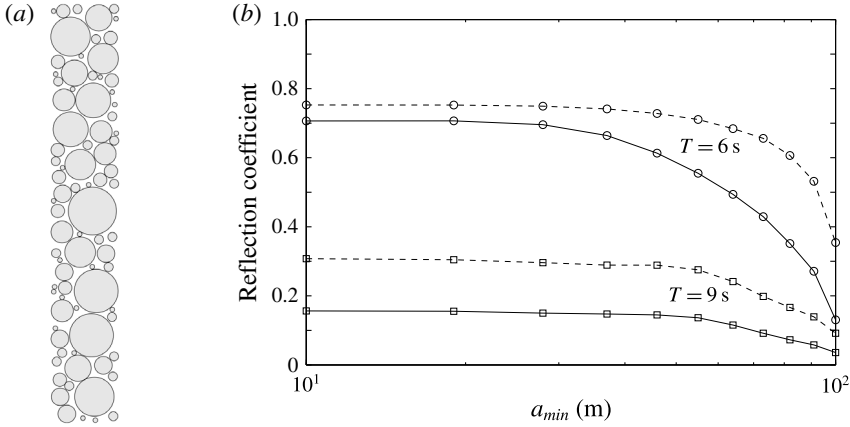
FIGURE 4. (a) Example of array generated using the random array generator described in appendix B. (b) Ensemble averages of reflection coefficients plotted against the minimum floe radius of the power-law FSD used to generate random realizations of the arrays. Results are given for single- and 10-slab arrays (solid and dashed lines respectively) and wave periods T=6 and 9 s (circle and square markers respectively). The wave forcing is a random sea state with normalized cosine square energy spreading.
