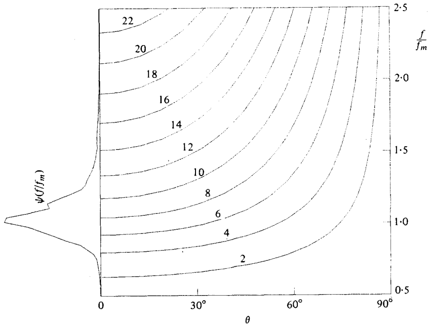
FIGURE 7. The same as figures 5 and 6 except that the contours of \Delta C/C_0 normalized by E_1(2\pi f_m)^4/g^2 are shown as a function of f/f_m and \theta . The corresponding frequency spectrum \psi_1 is shown in the left-hand side with arbitrary density scale.
