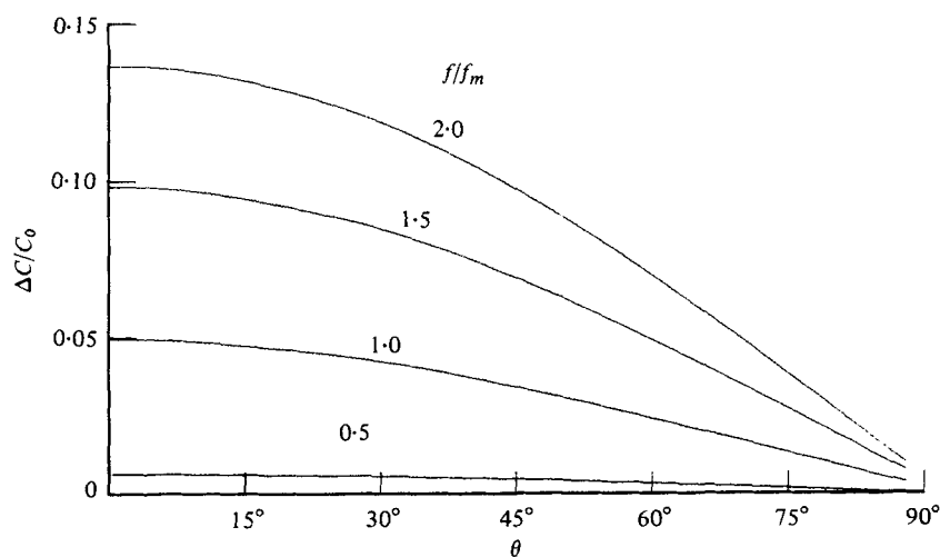
FIGURE 6. The change in phase velocity of the spectral component \Delta C/C_0 vs. \theta the propagation direction for various f/f_m .
