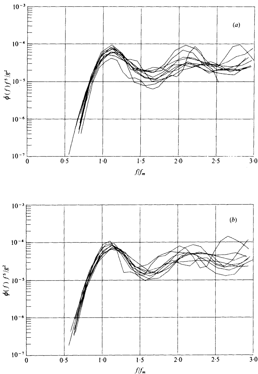
FIGURE 13. Normalized forms of the duration-limited wave spectra. (a) \bar{U}_* = 0-30.3 cm/s, F = 13 m. (b) \bar{U}_* = 0-30.6 cm/s, F = 18 m.
