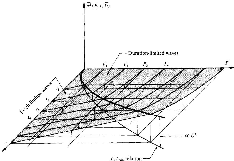
FIGURE 2. Schematic growth surface of wind-wave energy \bar{\eta}^2 for a duration time t , fetch F and a fixed wind speed \bar{U} .
