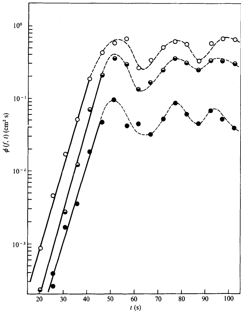
FIGURE 15. Growth of the spectral components with duration time. \bar{U}_* = 0\text{--}30.6 cm/s, F = 18 m. ●, f = 1.563 Hz; ●, f = 1.953 Hz; ○, f = 2.344 Hz.
