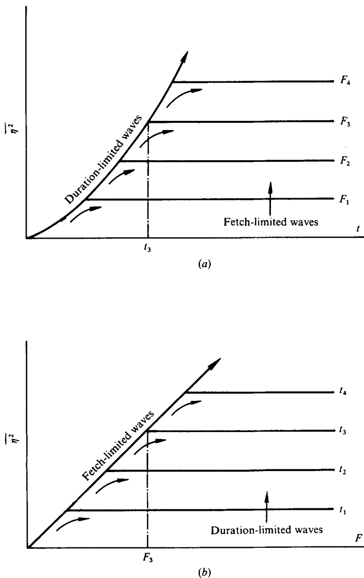
FIGURE 1. Schematic growth curves of wind-wave energy \overline{\eta^2} for a duration time t or fetch F with a fixed wind speed. (a) \overline{\eta^2} , t curve for various fetches F . (b) \overline{\eta^2} , F curve for various duration times t .
