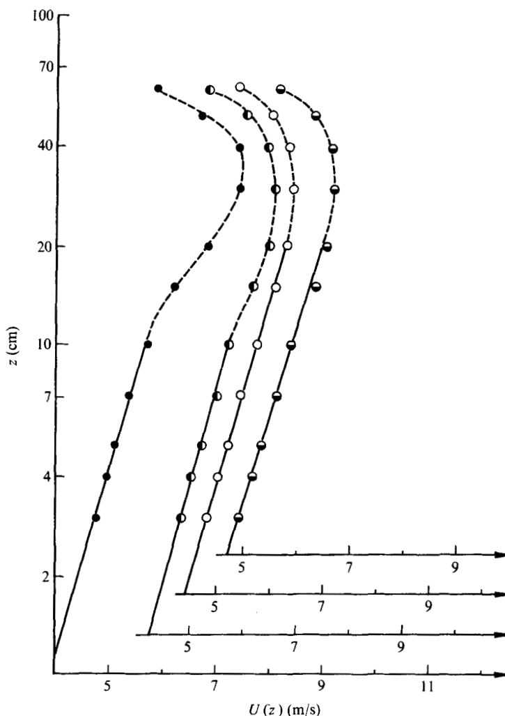
FIGURE 5. Wind profiles U(z) over the water surface. Abscissa is shifted successively for different fetches. \bullet , F = 3 m; \circ , F = 8 m; \circ , F = 13 m; \bullet , F = 18 m.
