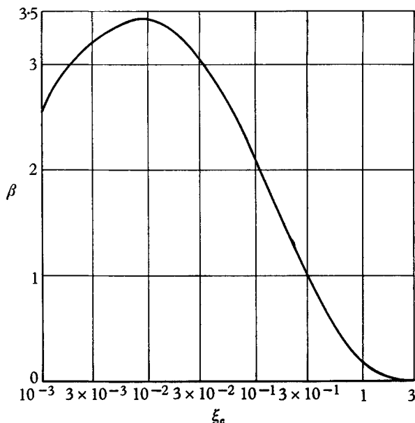
FIGURE 2. \beta vs \xi_c .
