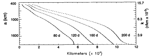
FIG. 9. The transform maximums corresponding to the dispersion tongues. The evolution of the line in time gives the group velocity. Note the gradual flattening of the lines in the western region.
