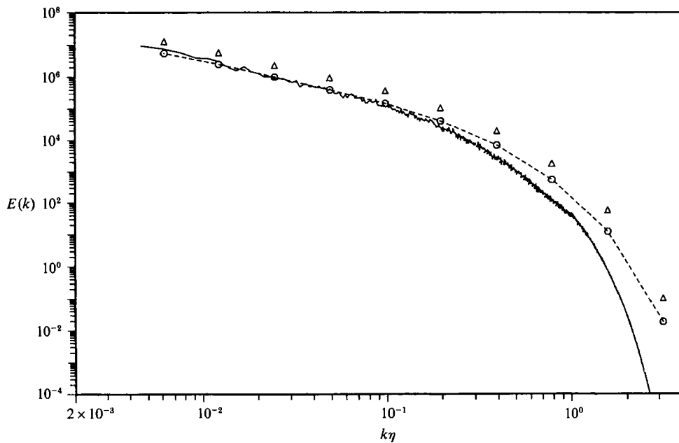
FIGURE 7. Dual energy spectrum of the turbulent flow behind the circular cylinder (streamwise one-dimensional spectrum). —, Usual Fourier spectrum; ○, wavelet spectrum; △, wavelet mean energy at every scale to which one standard deviation (computed from the spatial fluctuations) has been added.
