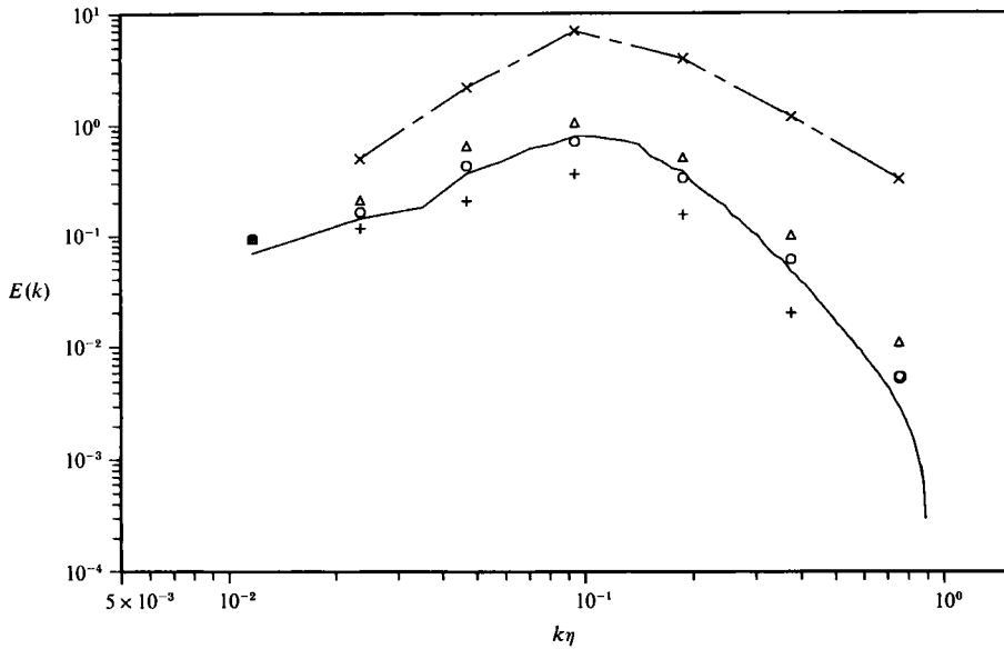
FIGURE 11. Dual spectrum of the homogeneous shear flow. These are total spectra (sum over all three velocity components). —, Usual (radial) Fourier spectrum; \circ , wavelet spectrum; \Delta and + , mean spectrum plus and minus the standard deviation of the spatial fluctuations of the energies at every scale. The \times correspond to the maximum spatial energy occurring at every scale.
