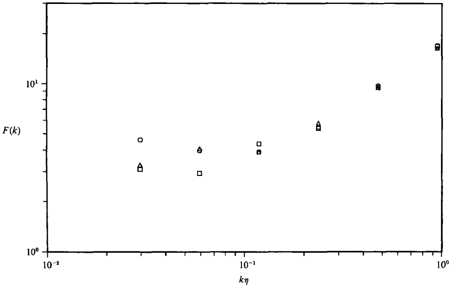
FIGURE 12. Flatness factors of the wavelet coefficients computed from the simulation of isotropic turbulence. Different symbols correspond to different velocity components: \square , u ; \circ , v ; \triangle , w .
