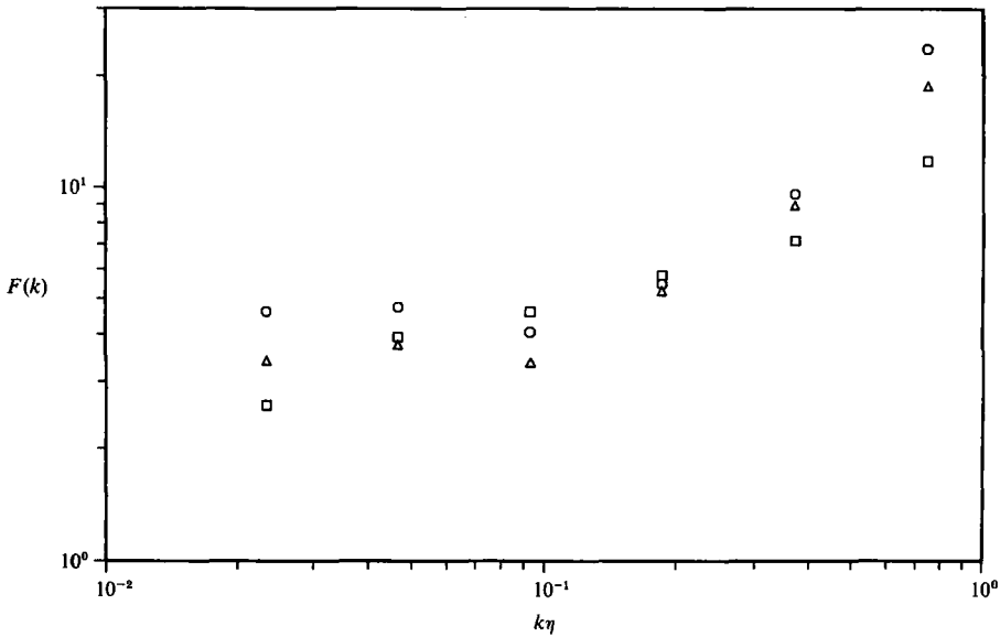
FIGURE 13. Flatness factors of the wavelet coefficients computed from the simulation of homogeneous sheared turbulence. Different symbols correspond to different velocity components: \square , u ; \circ , v ; \triangle , w .
