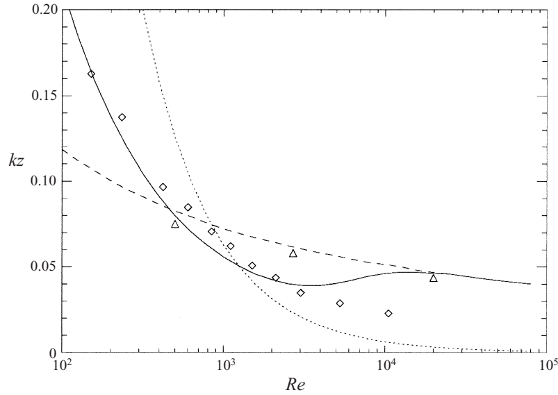
FIGURE 8. Inner region depth in flow over hills: —, kl from (3.5); — —, kl_H from (3.1); ···, z^+ = 10 ; symbols denote half the height where \max(\text{Re}[\hat{w}]/u_*) is located, from the low- Re ( \diamond ) and high- Re ( \triangle ) models.
