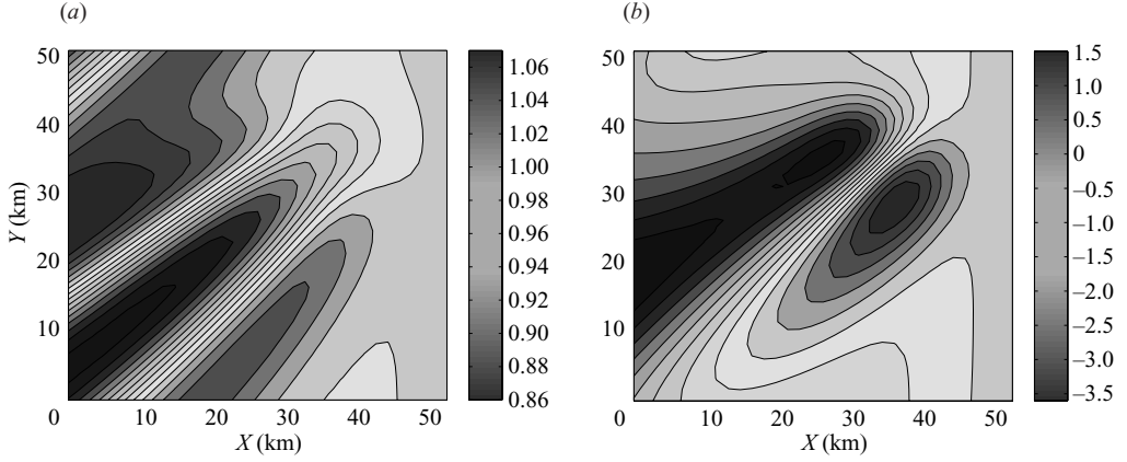
FIGURE 2. Steady-state wave amplitude in the baseline case: (a) |A|(X) (m); (b) \Theta(X) (rad).
