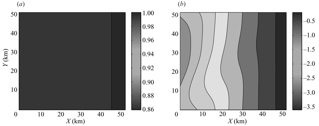
FIGURE 3. Steady-state wave amplitude: (a) |A|(X) [m] without the bottom depression; (b) \Theta(X) (rad) without the currents.
