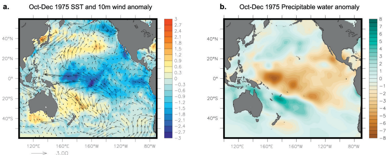
FIG. 2. Seasonal mean anomalies of (a) SST (in °C) from the HADISST1 (Rayner et al. 2003) and 10-m wind (in m s -1 ) and (b) precipitable water content (in kg m -2 ) for Oct–Dec 1975 from the National Centers for Environmental Prediction (NCEP) Twentieth Century Reanalysis (Compo et al. 2011).
